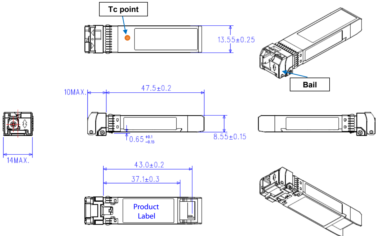
Figure 7. Package outline diagram and example
