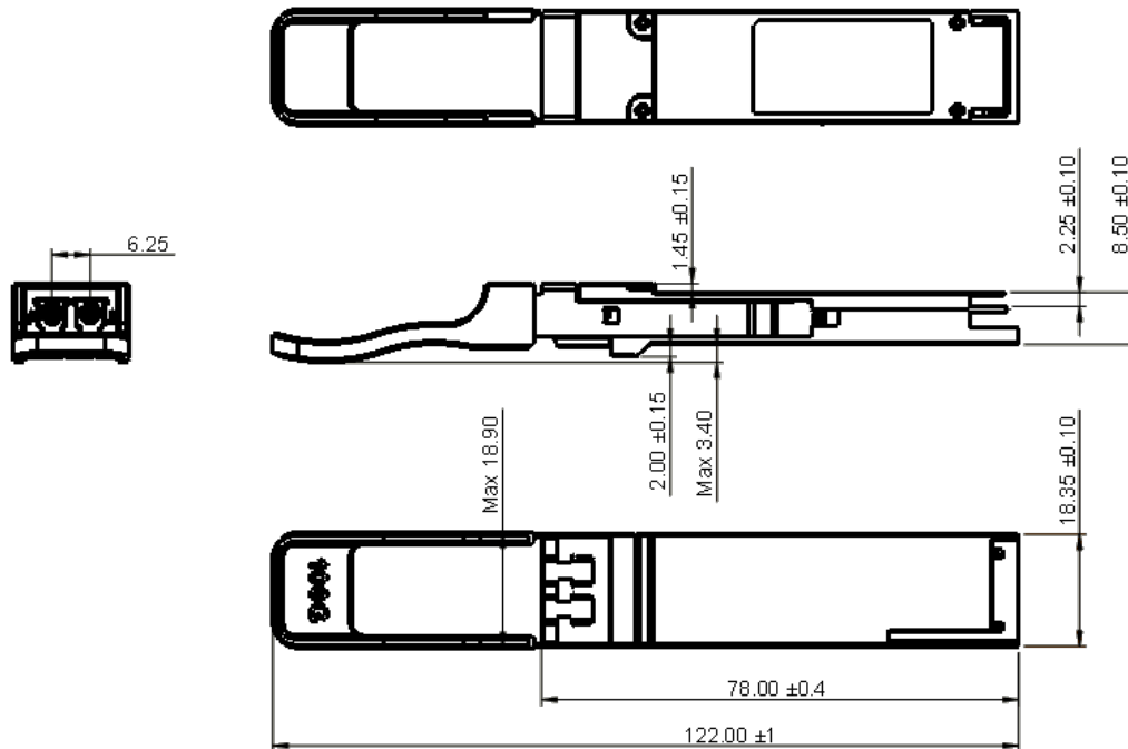
Figure 5. Mechanical Outline
