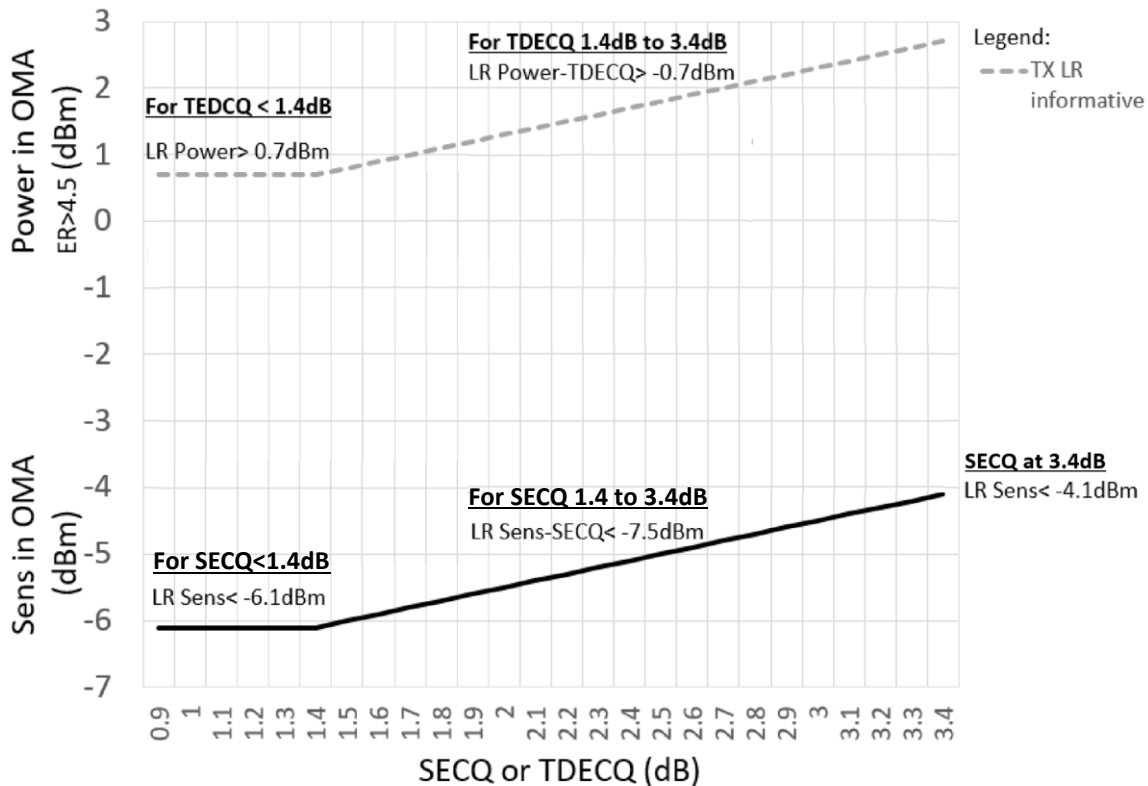
Figure 4. Stressed Receiver Sensitivity Mask for 400G-LR4
