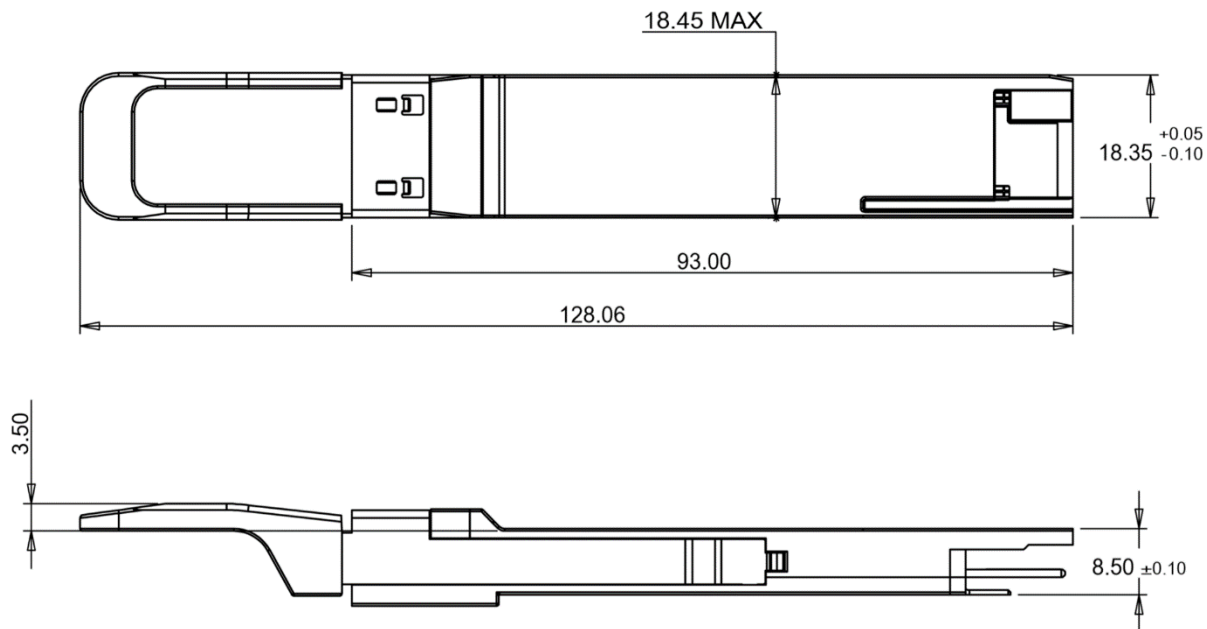
Figure 5. Mechanical Outline
