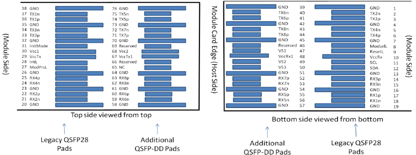
Figure 2. MSA Compliant Connector
