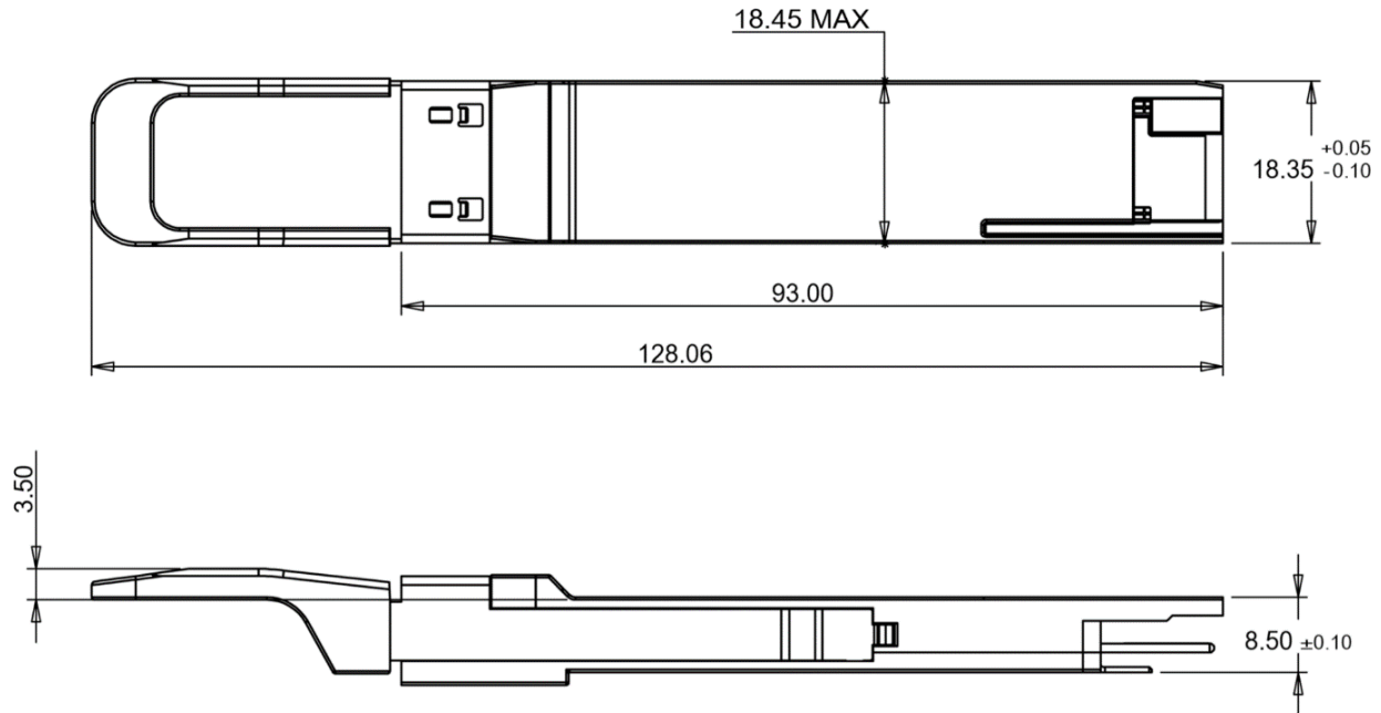
Figure 5. Mechanical Outline
