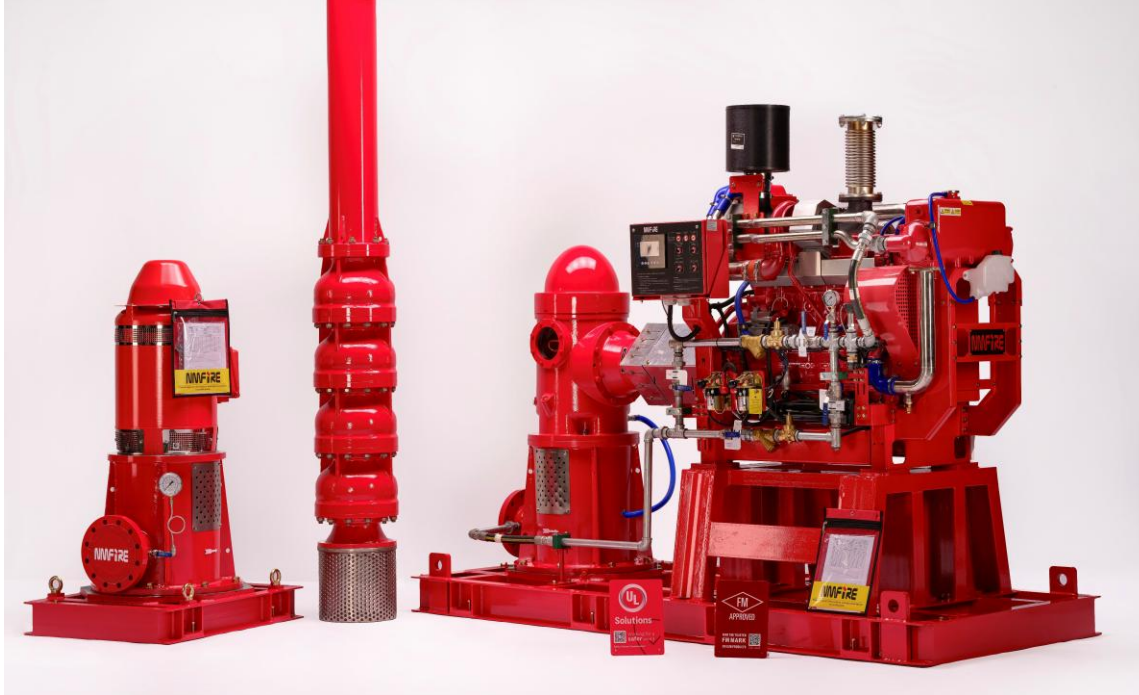
Vertical Turbine Pump, Engine : 3000 GPM, 140 PSI Jockey Pump : 40 GPM, 150 PSI
