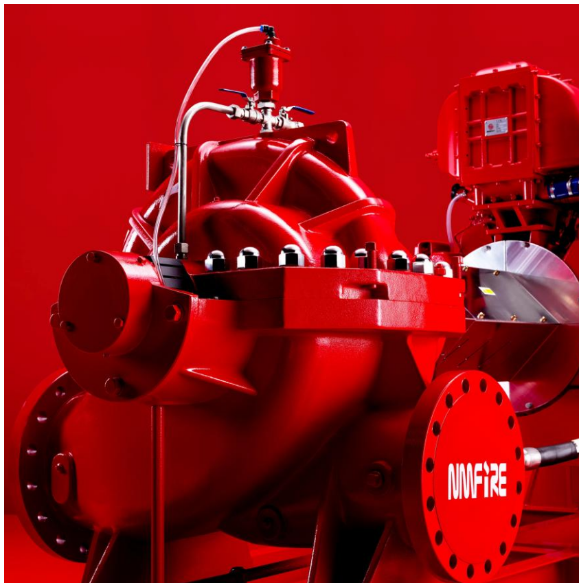
Horizontal Split Case Pump, Engine : 1000 GPM, 152 PSI Jockey Pump : 20 GPM, 160 PSI
