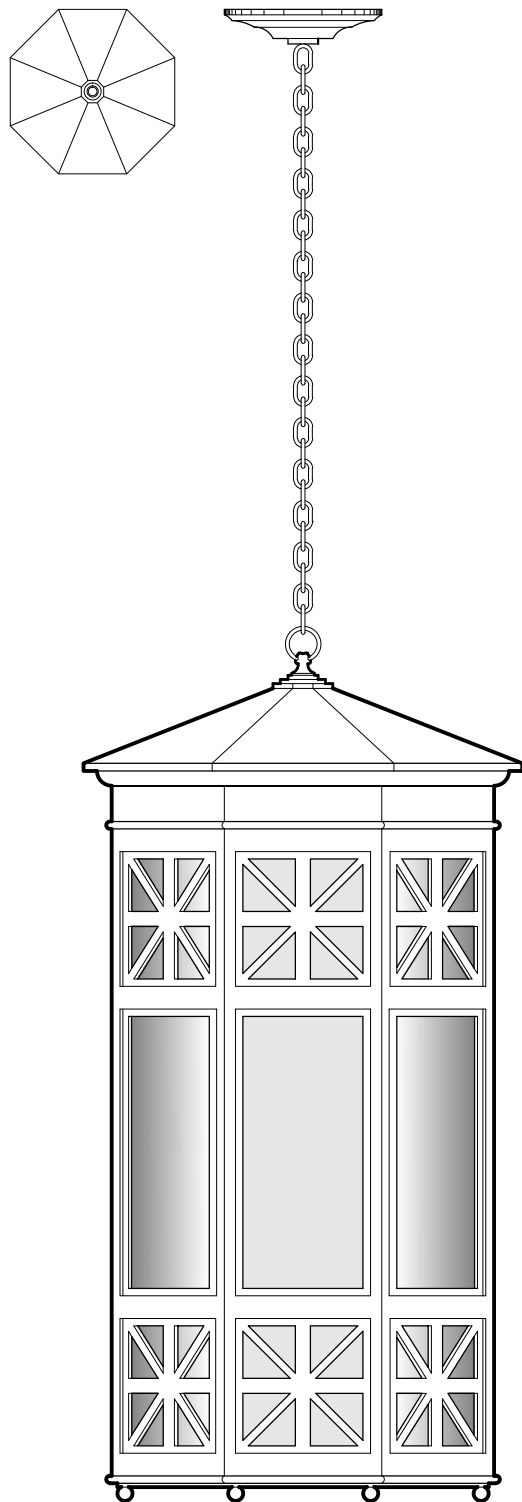
P1842 26" SQ. x 53" H BRONZE METALWORK TRANSLUCENT WHITE GLASS DIFFUSER
