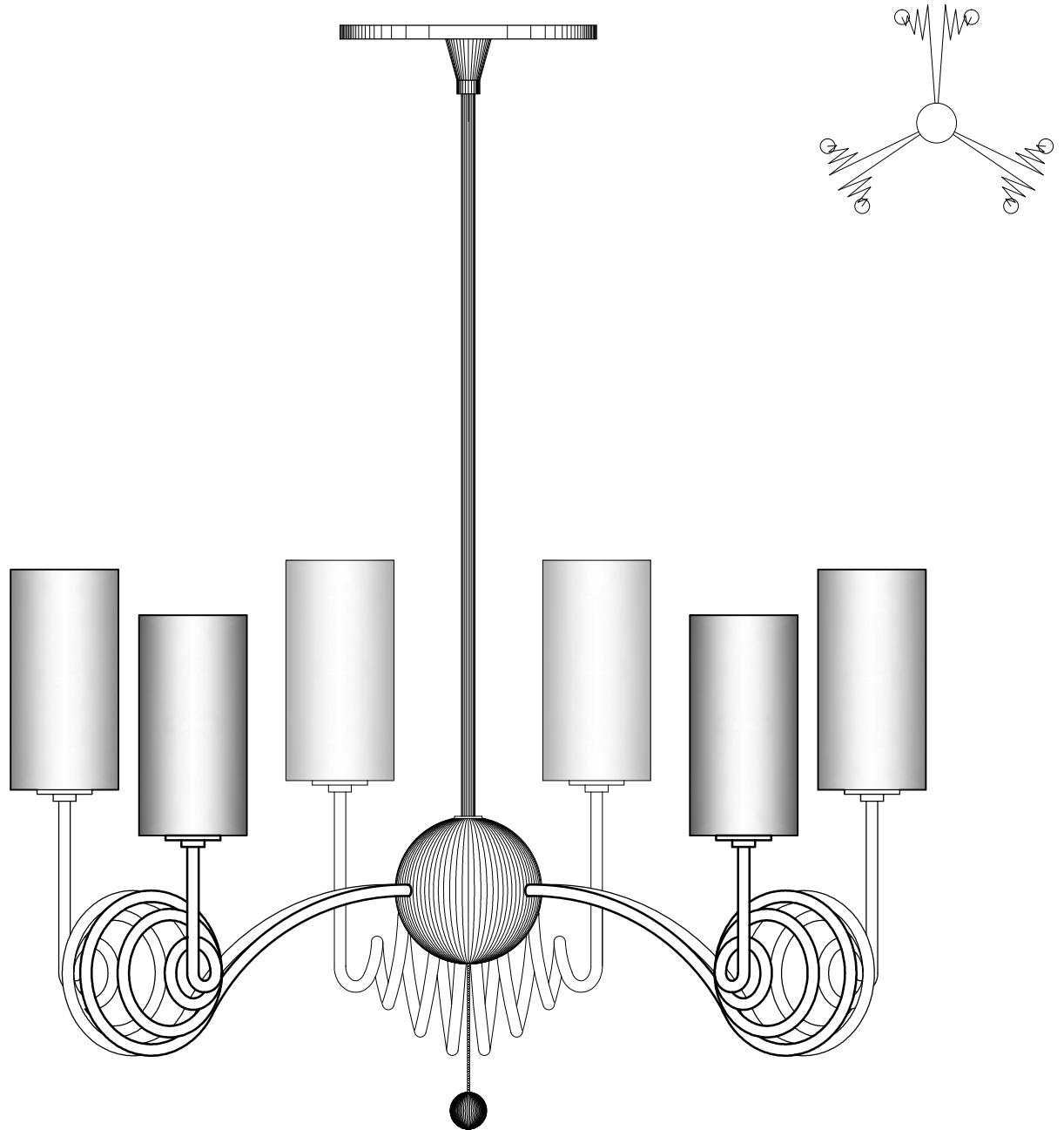
P1896 48" DIAMETER STEEL METALWORK NOMAX FABRICATED SHADE
