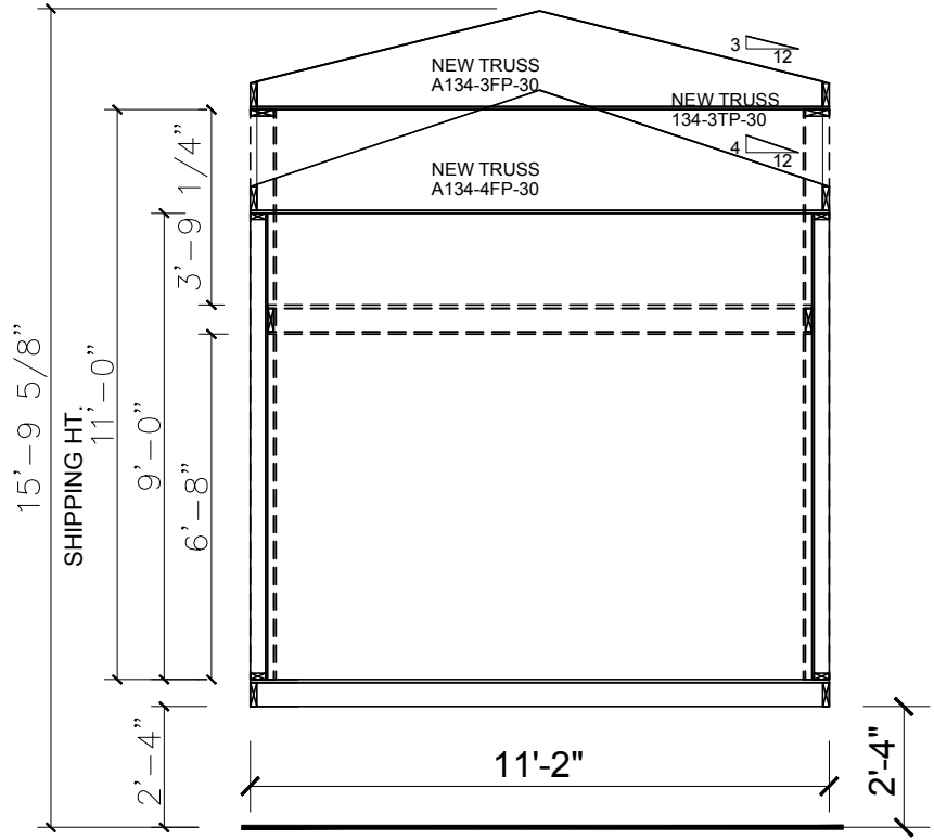
9' flat CROSS SECTION STD. 11' flat CROSS SECTION W/OPT. LOFT
