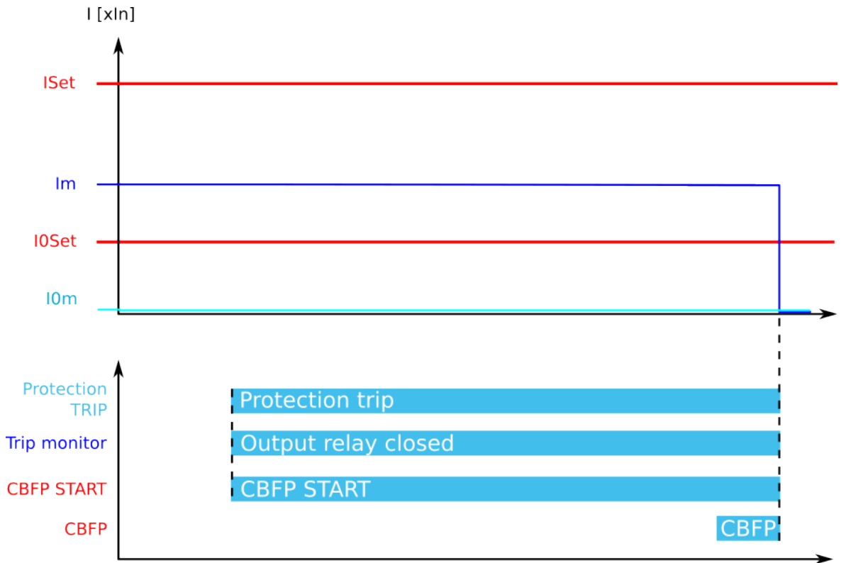
Figure. 4.4.8 - 106. CBFP when "Current or DO" is the selected criterion.
