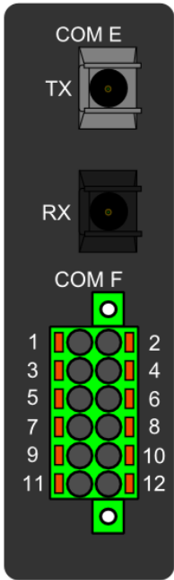
Figure. 7.5.5 - 201. Serial RS-232 module connectors.
