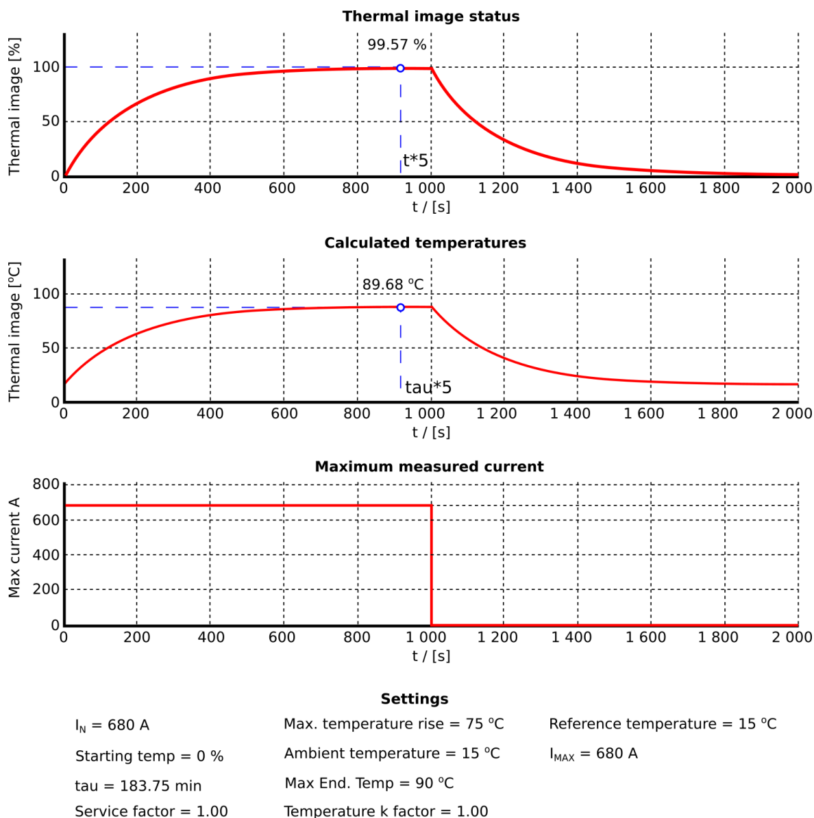
Figure. 4.4.14 - 140. Thermal image response with maximum load (installation according to presumptions).
