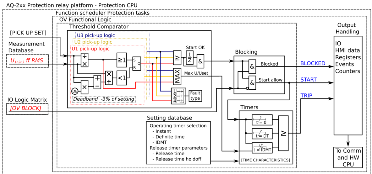
Figure. 4.4.9 - 109. Simplified function block diagram of the U> function.
