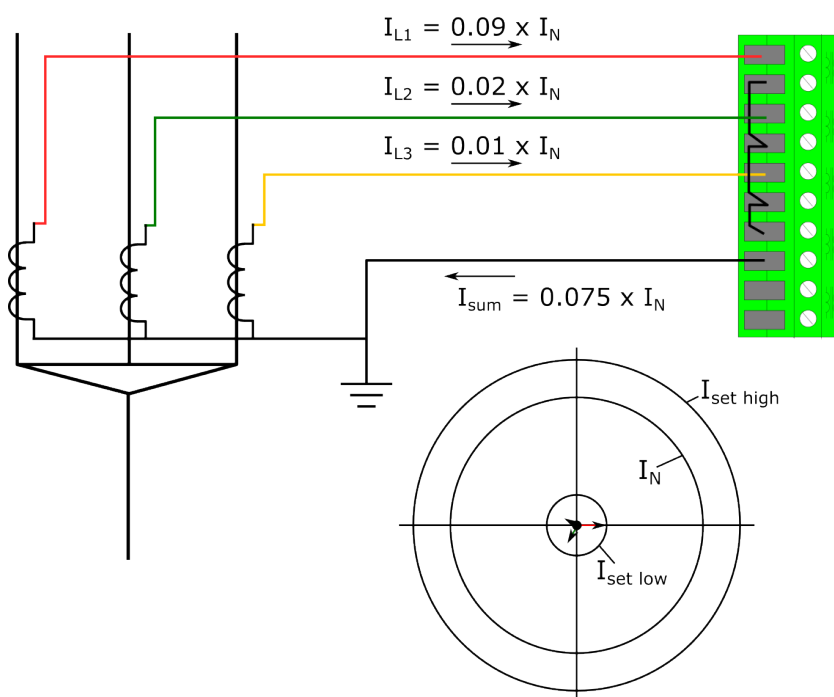
Figure. 4.6.1 - 166. Low current and heavy unbalance.
