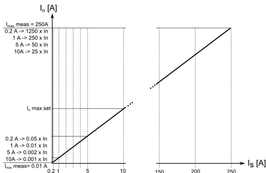
Figure. 4.4.1 - 84. Measurement range in relation to the nominal current.
