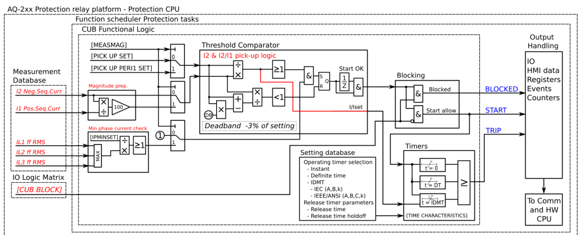
Figure. 4.4.6 - 95. Simplified function block diagram of the I2> function.
