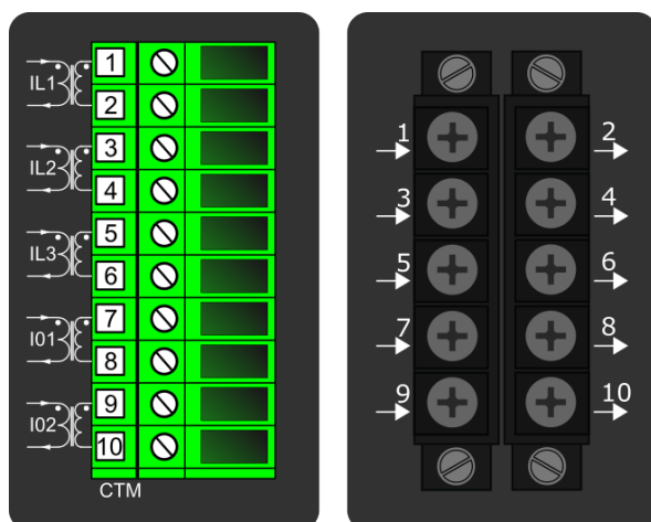
Figure. 7.3 - 193. Module connections with standard and ring lug terminals.
