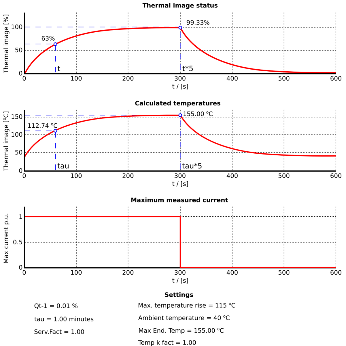
Figure. 4.4.14 - 131. Example of thermal image calculation with nominal conditions.
