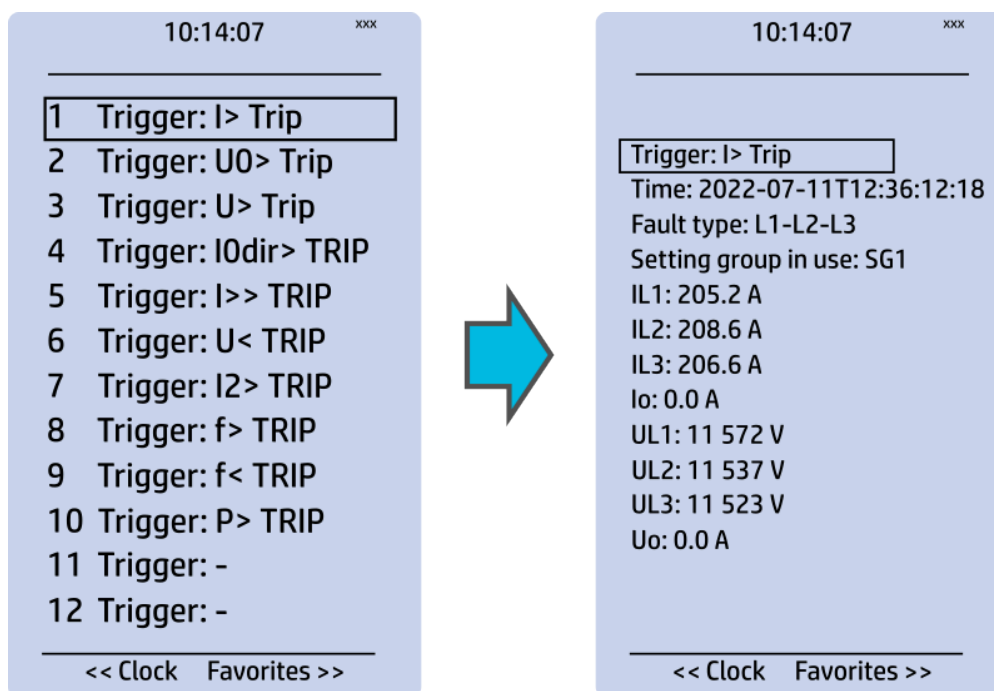
Figure. 4.6.7 - 178. 12 latest recordings can be accessed from HMI if "Fault registers" view has been enabled in "Carousel designer" tool.
