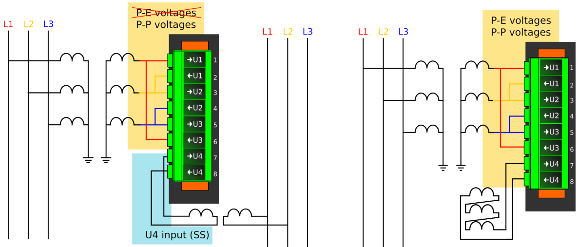
Figure. 4.4.10 - 115. Selectable measurement magnitudes with 3LL+U4 VT connection (P-E voltages not available without residual voltage).
