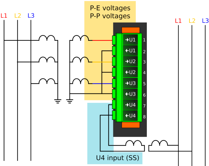
Figure. 4.4.9 - 110. Selectable measurement magnitudes with 3LN+U4 VT connection.
