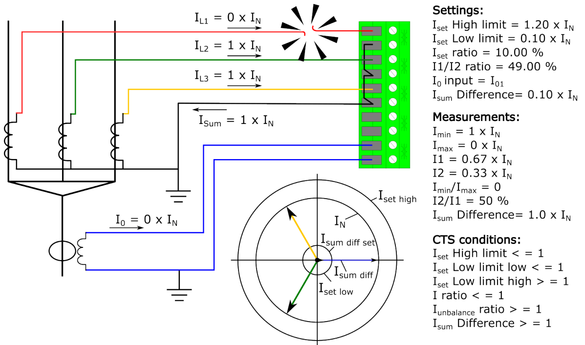
Figure. 4.6.1 - 168. Broken secondary phase current wiring.
