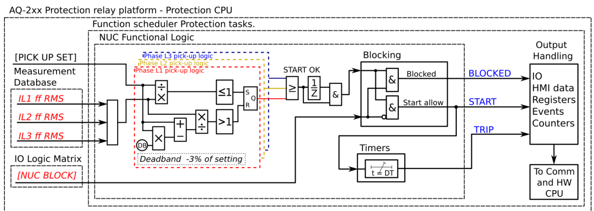
Figure. 4.4.13 - 130. Simplified function block diagram of the I< function.
