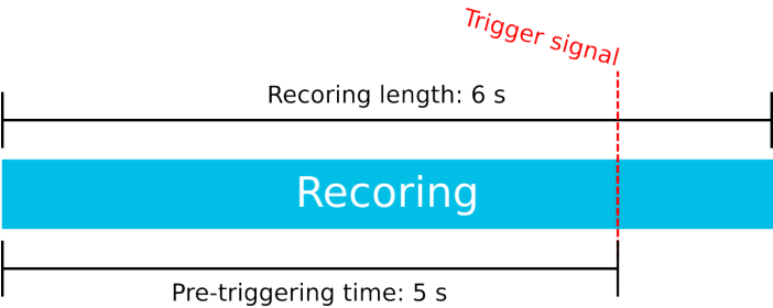
Figure. 4.6.4 - 176. Effects of recording length and pre-triggering time signals. This example is based on the settings shown above.
