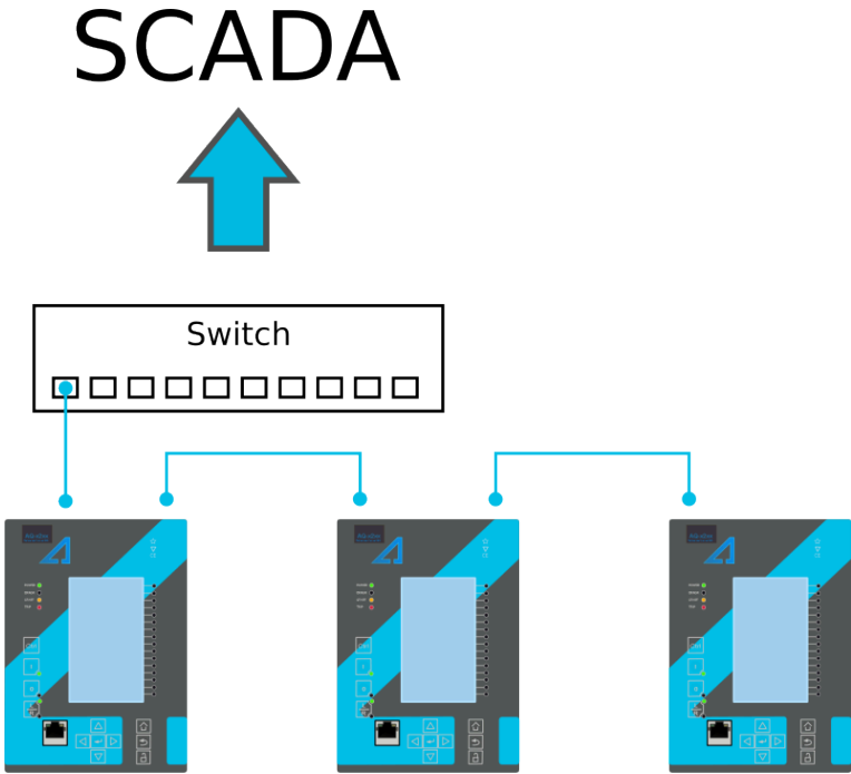
Figure. 7.5.8 - 207. Example of a multidrop configuration.
