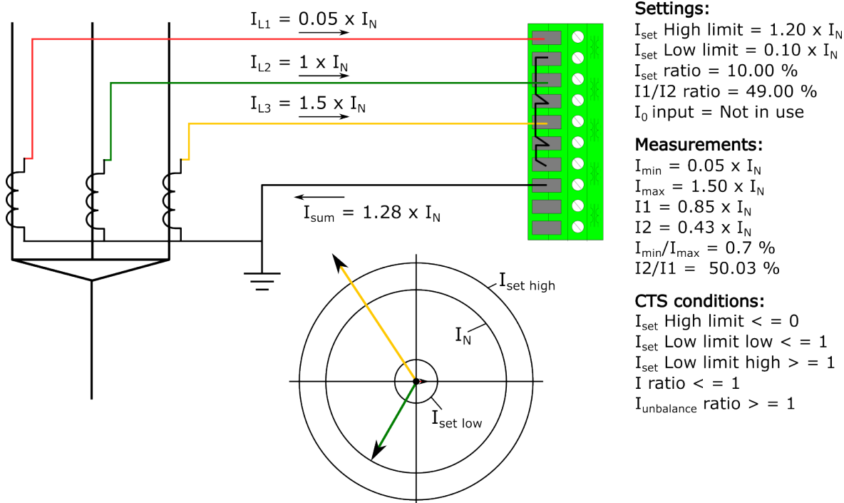
Figure. 4.6.1 - 165. No wiring fault but heavy unbalance.
