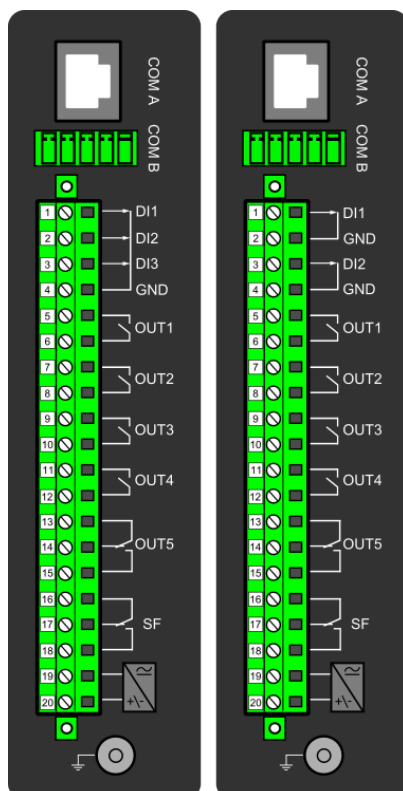
Figure. 7.2 - 192. CPU module.
