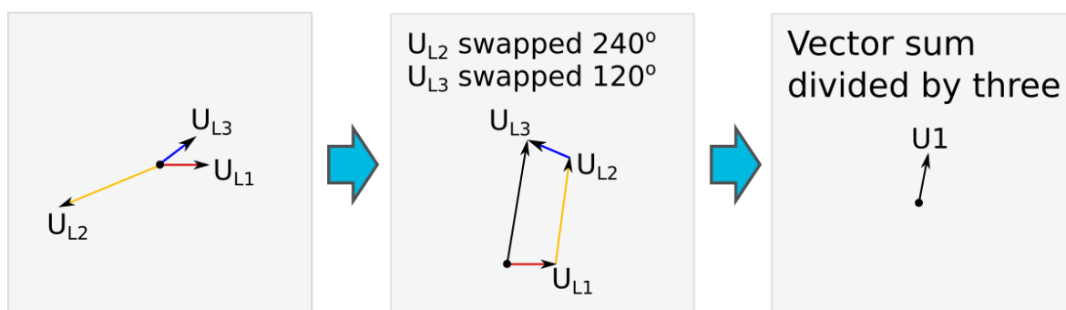
Figure. 4.4.12 - 127. Close-distance short-circuit between phases 1 and 3.
