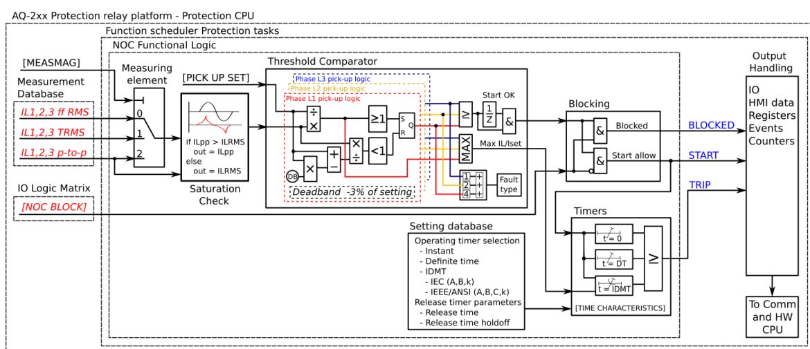
Figure. 4.4.4 - 93. Simplified function block diagram of the I> function.
