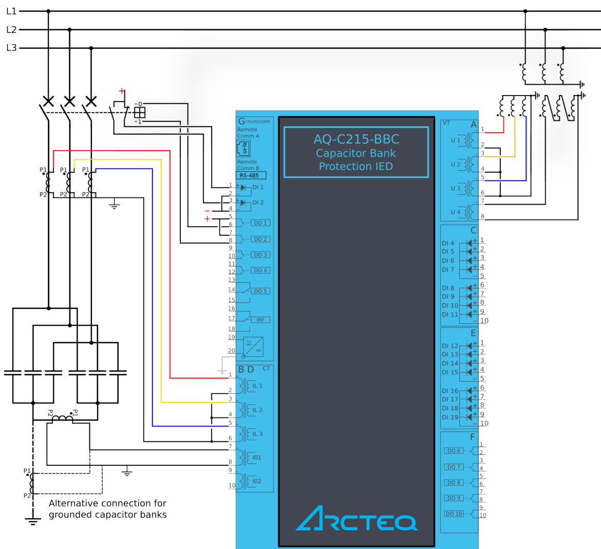
Figure. 6.2 - 183. Application example and its connections in double wye bank.
