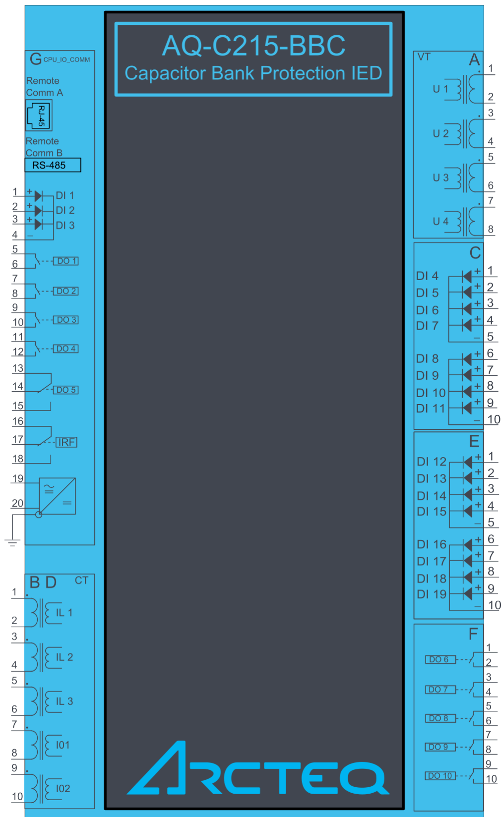
Figure. 6.1 - 180. The AQ-C215 variant with digital input and output modules.
