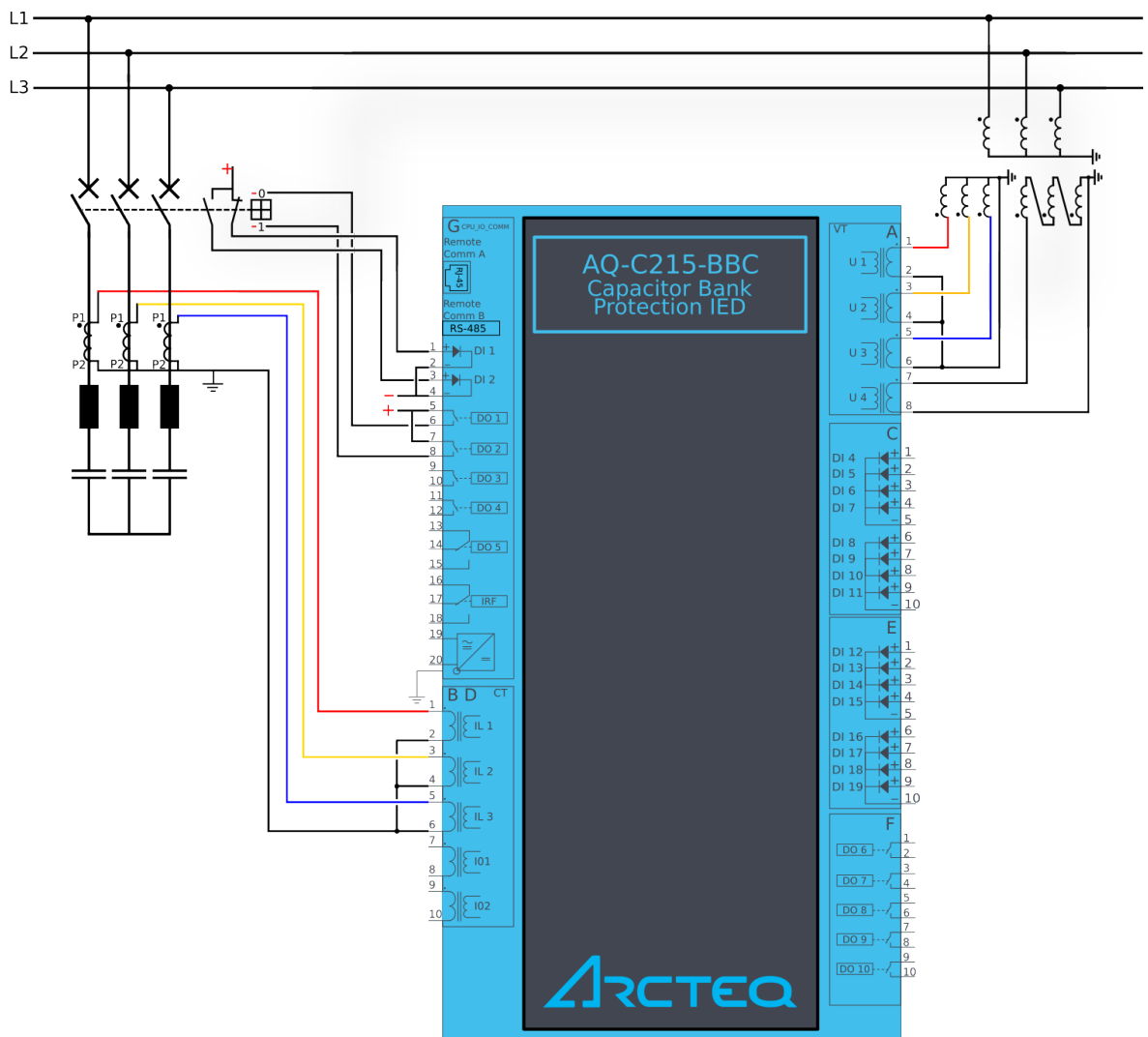
Figure. 6.2 - 182. Application example and its connections.
