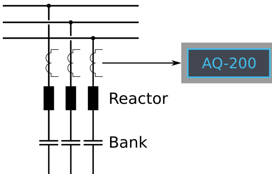
Figure. 4.4.3 - 92. Measurement connection of the luc> function.
