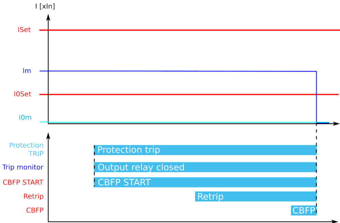
Figure. 4.4.8 - 102. Retrip and CBFP when "Current or DO" is the selected criterion.
