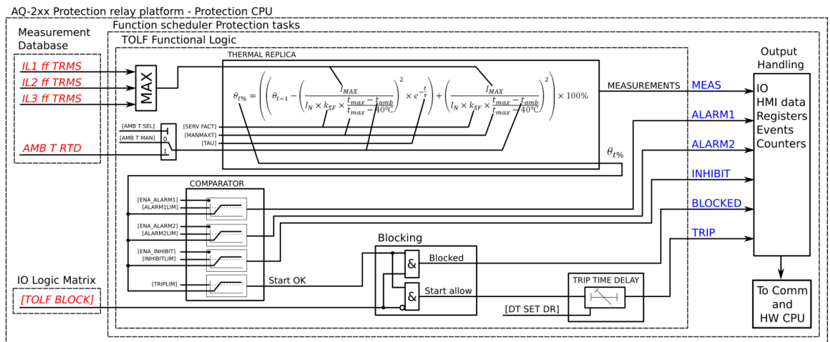
Figure. 4.4.14 - 143. Simplified function block diagram of the TF> function.
