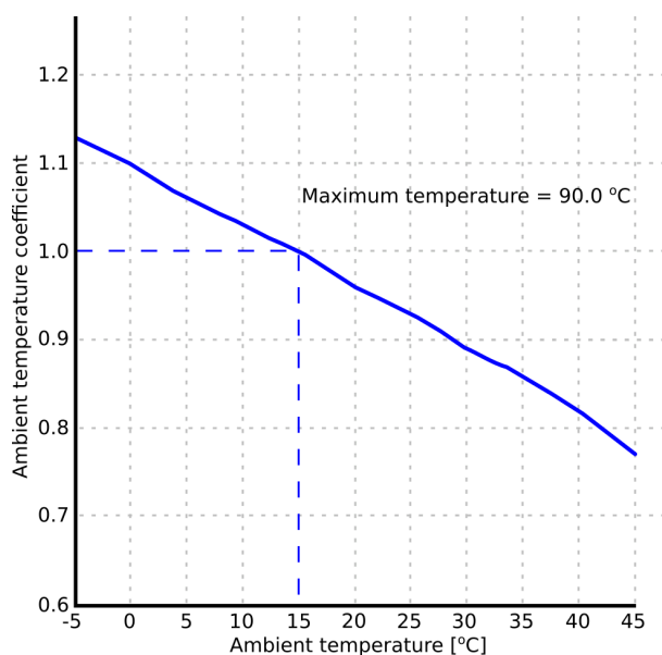
Figure. 4.4.14 - 135. Set correction curve for ambient temperature.
