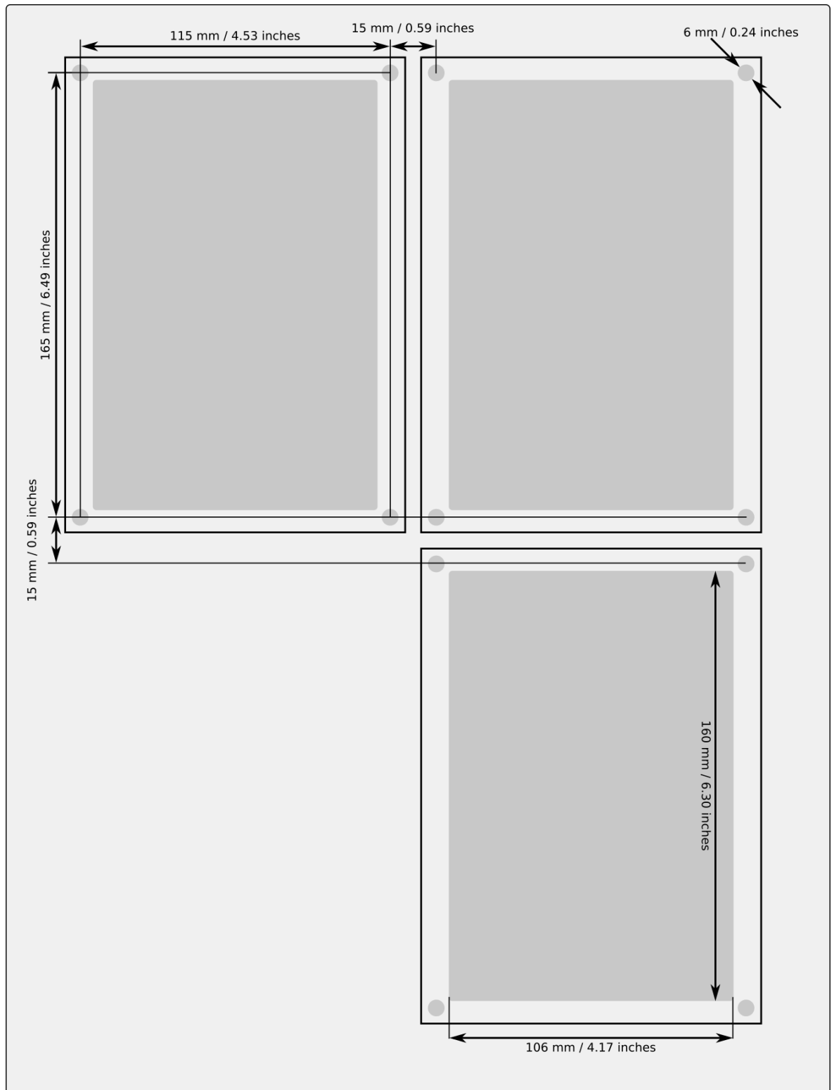
Figure. 7.6 - 211. Panel cutout dimensions and device spacing.
