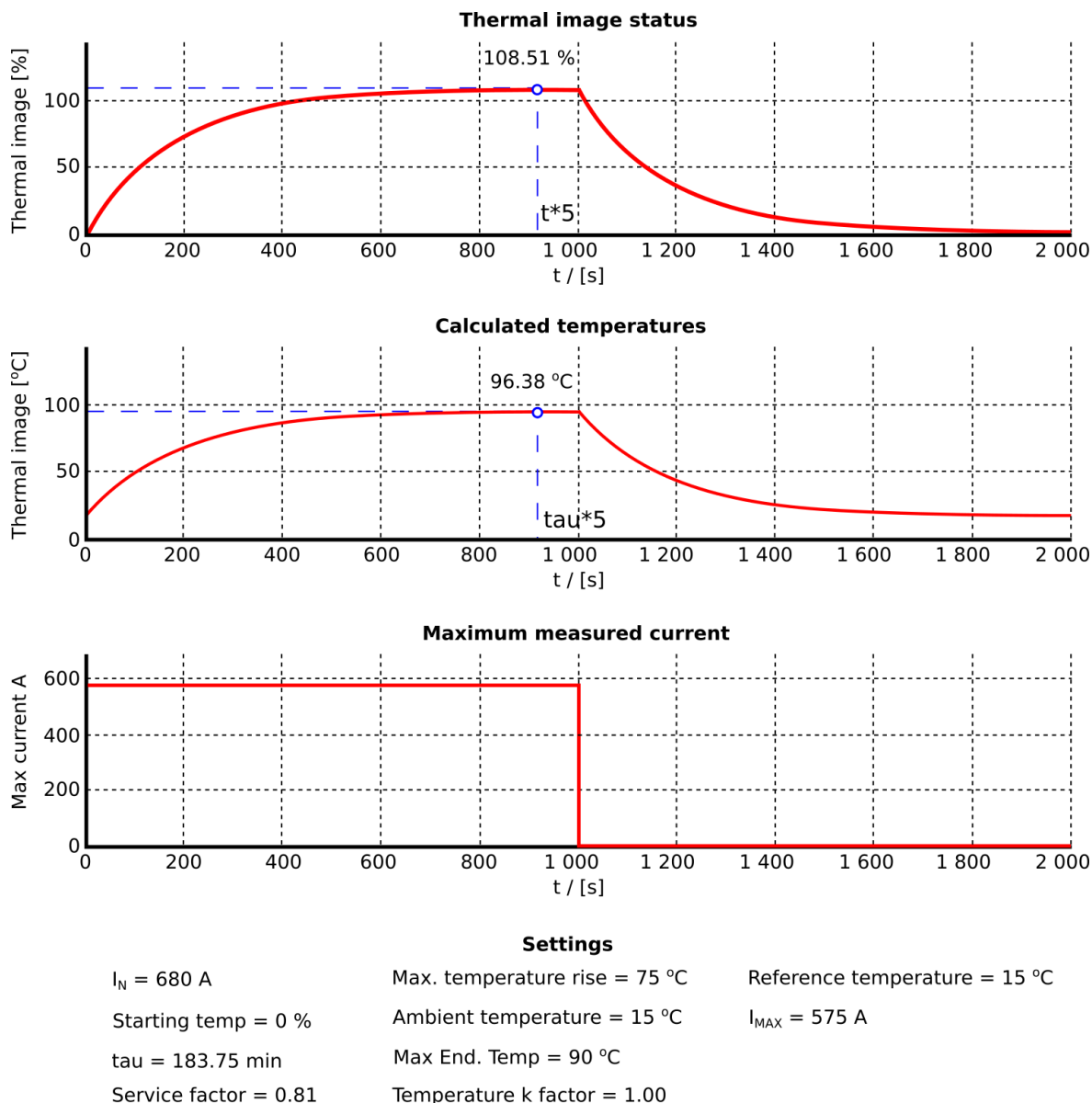
Figure. 4.4.14 - 141. Thermal image response with nominal currents and fine-tuned k_{\text{SF}} correction factor.
