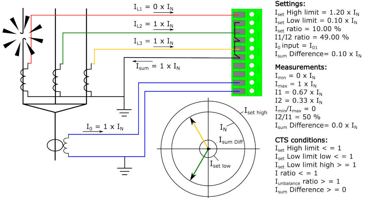
Figure. 4.6.1 - 169. Broken primary phase current wiring.
