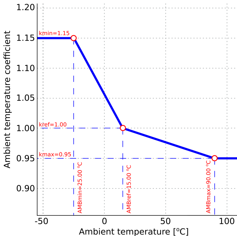
Figure. 4.4.14 - 132. Ambient temperature coefficient calculation (a three-point linear approximation and a settable correction curve).
