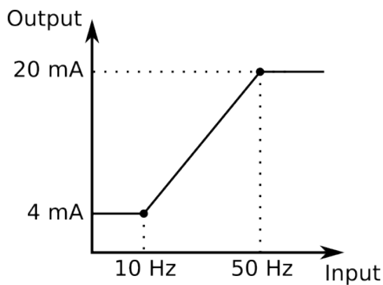
Figure. 4.5.6 - 156. Example of the effects of mA output channel settings.
