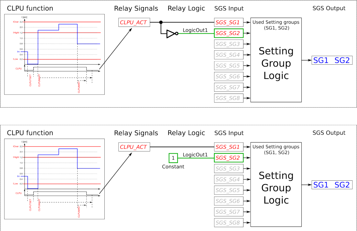
Figure. 4.5.2 - 152. Entirely application-controlled setting group change with the cold load pick-up function.
