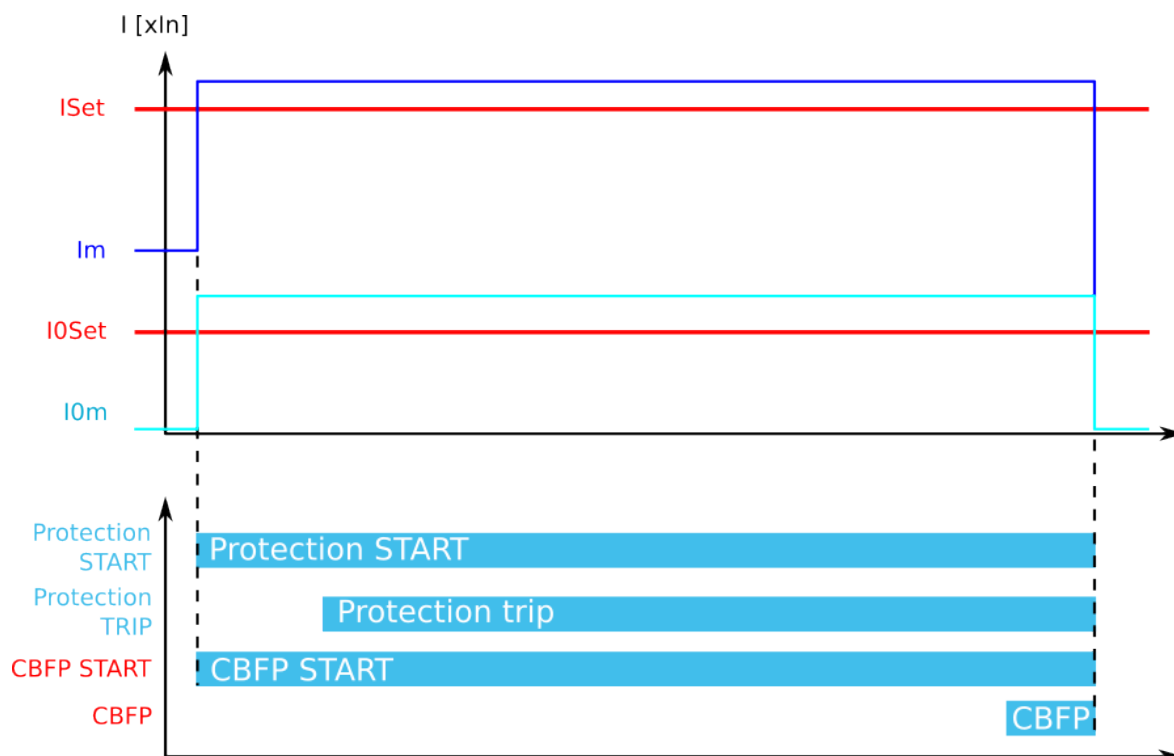
Figure. 4.4.8 - 104. CBFP when "Current" is the selected criterion.
