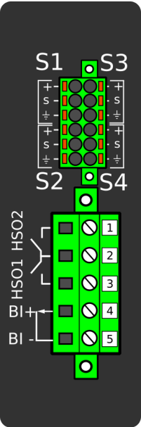
Figure. 7.5.3 - 198. Arc protection module.
