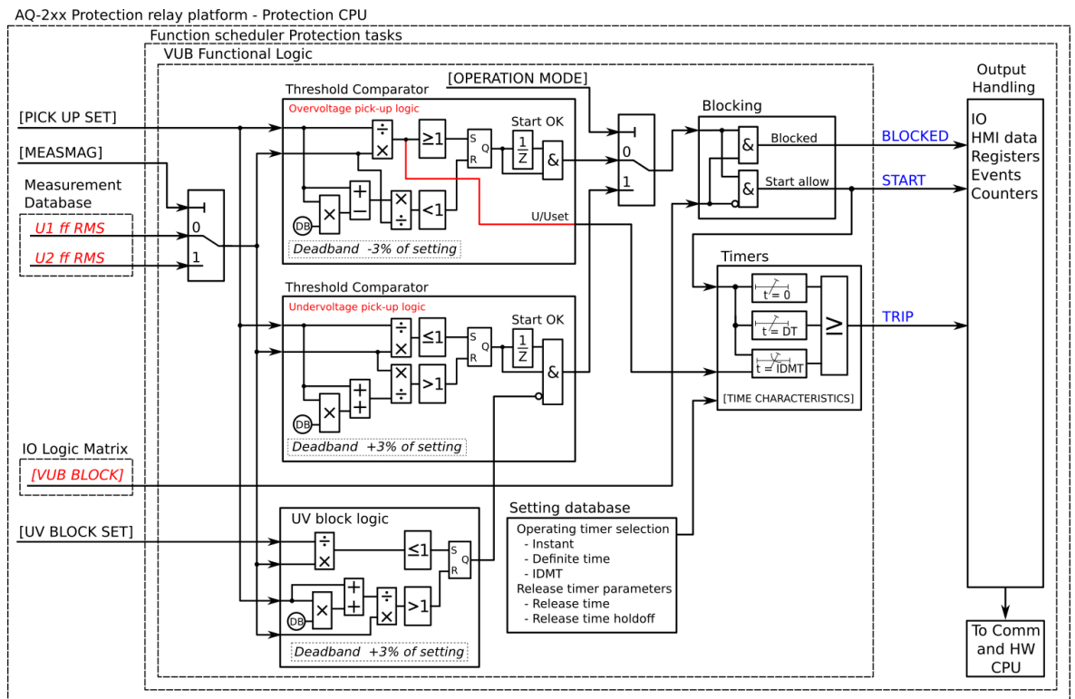
Figure. 4.4.12 - 128. Simplified function block diagram of the U1/U2>/< function.
