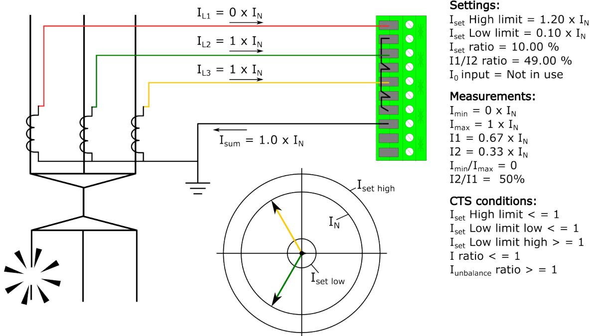
Figure. 4.6.1 - 164. Primary circuit fault in phase L1 wiring.
