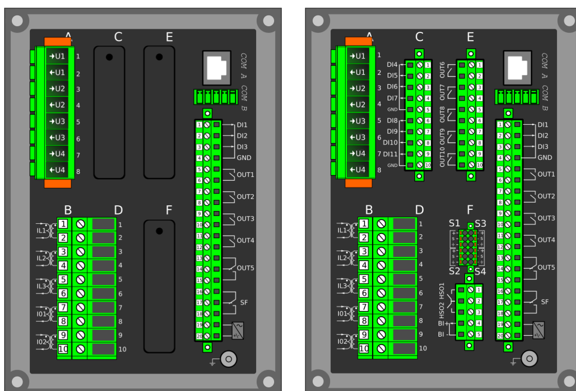
Figure. 7.1 - 190. Modular construction of AQ-X215.
