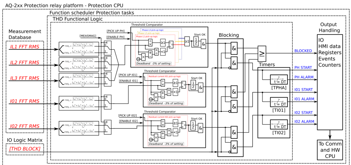
Figure. 4.6.3 - 174. Simplified function block diagram of the total harmonic distortion monitor function.
