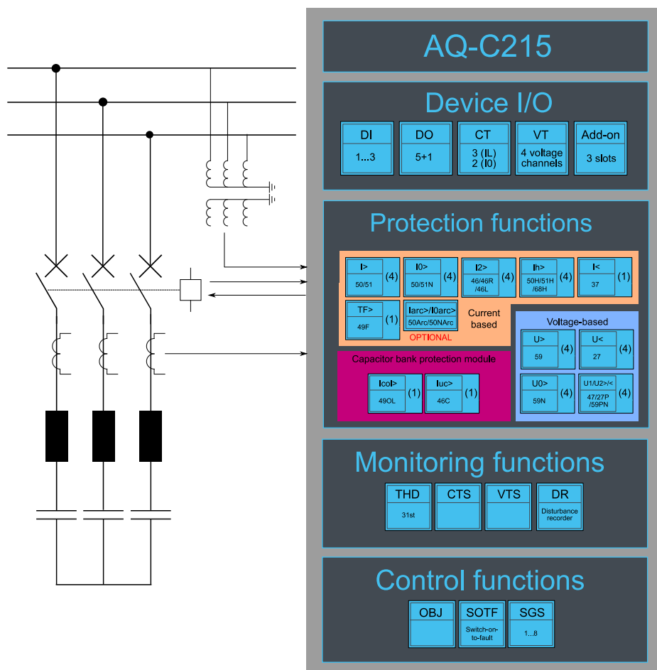
Figure. 6.1 - 181. AQ-C215 application example with function block diagram.
