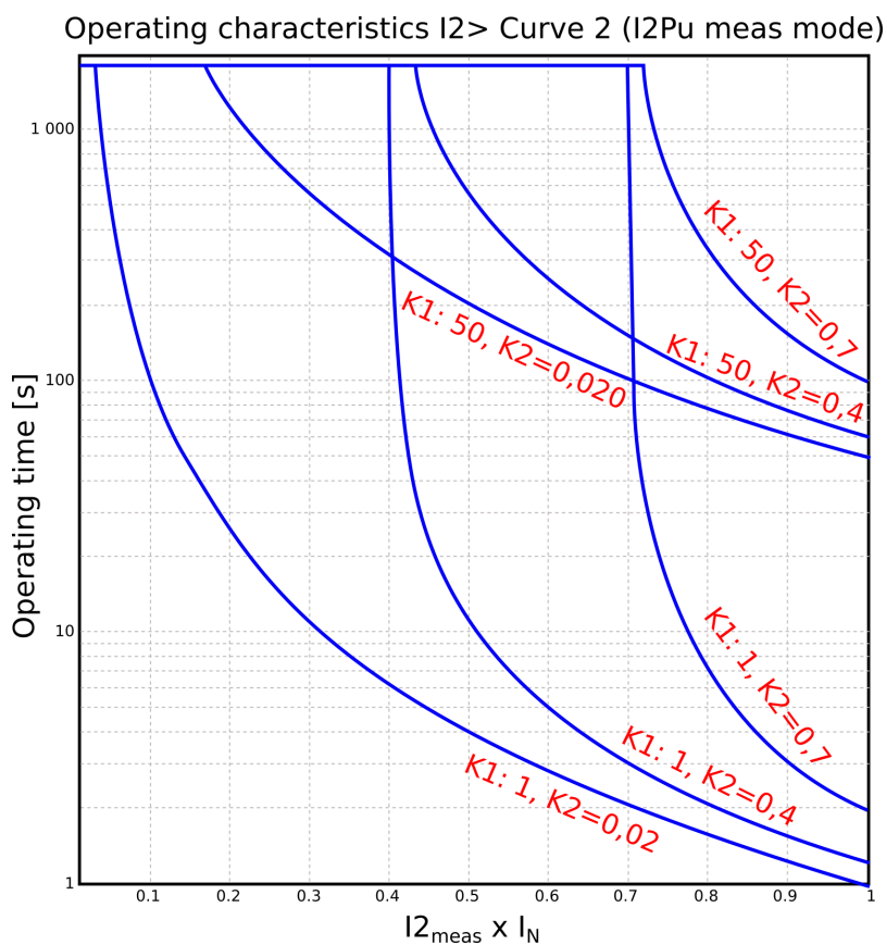
Figure. 4.4.6 - 96. Operation characteristics curve for I2> Curve2.
