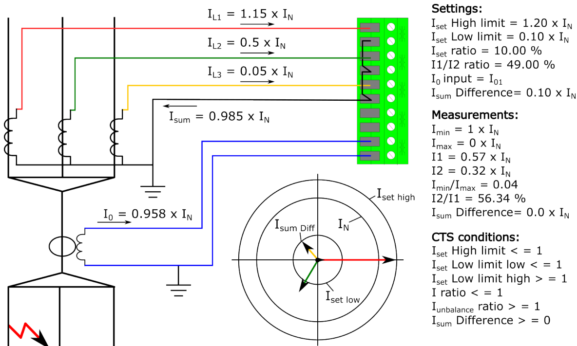
Figure. 4.6.1 - 170. Primary side high-impedance earth fault.
