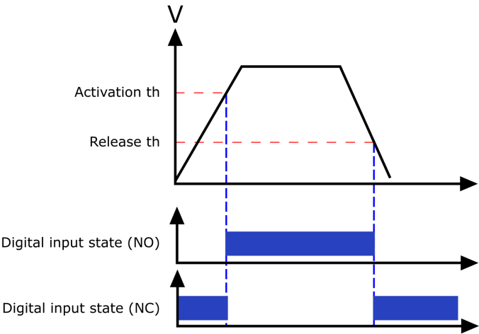
Figure. 7.5.1 - 196. Digital input state when energizing and de-energizing the digital input channels.
