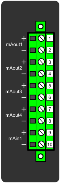
Figure. 7.5.9 - 208. Milliampere (mA) I/O module connections.
