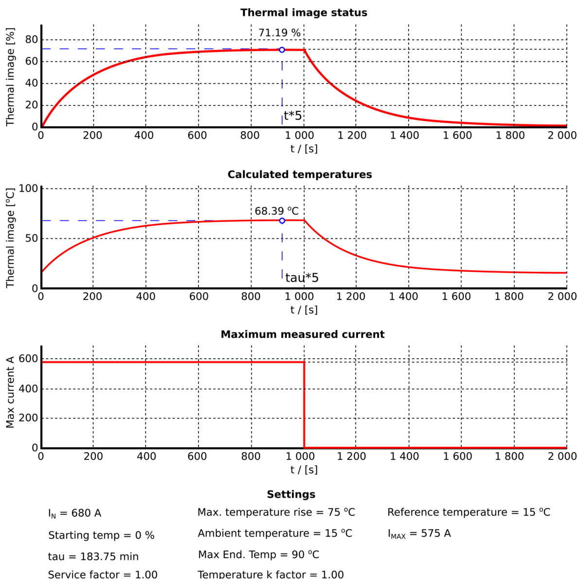
Figure. 4.4.14 - 139. Thermal image response with nominal load (installation according to presumptions).
