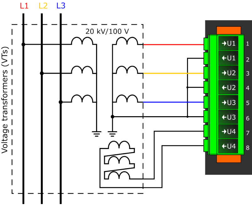
Figure. 4.2.2 - 69. Connections.
