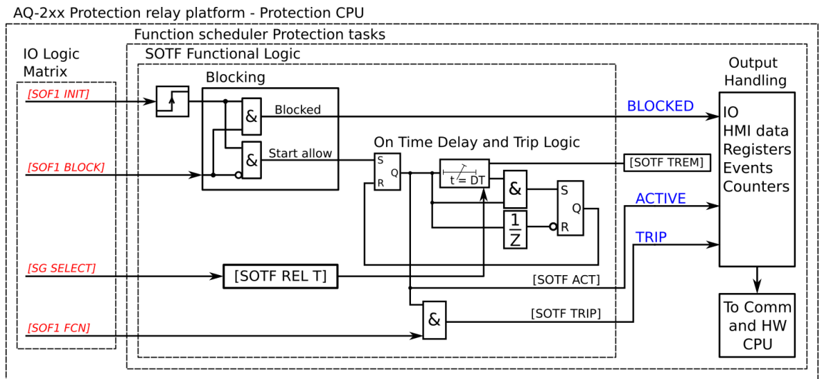
Figure. 4.5.5 - 155. Simplified function block diagram of the switch-on-to-fault function.
