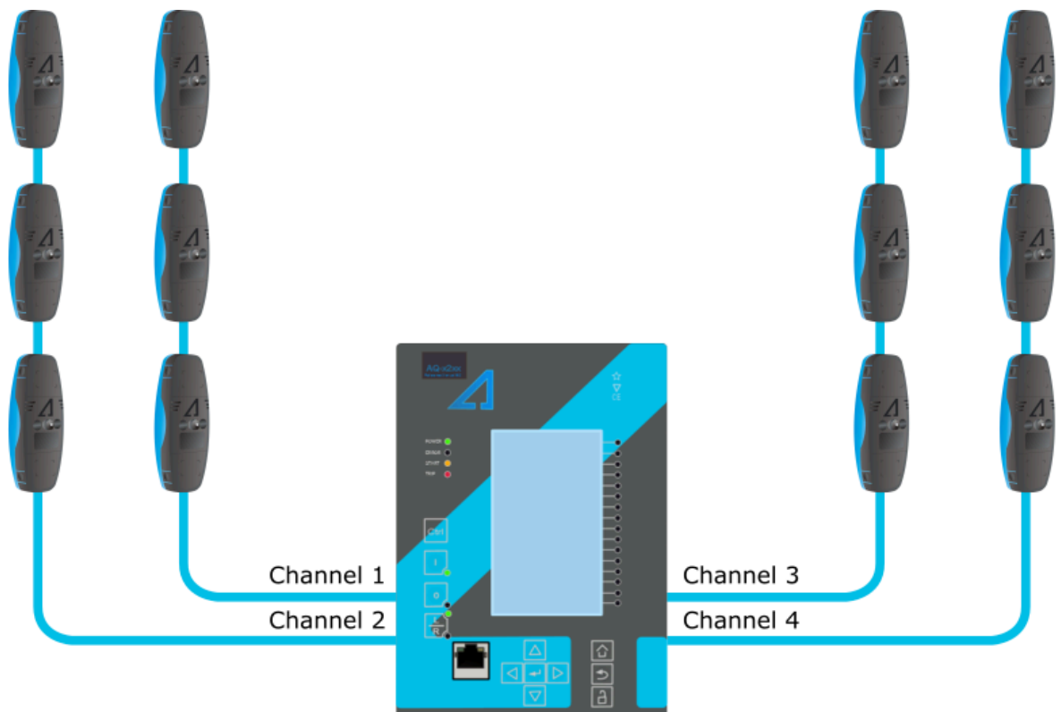
Figure. 4.4.17 - 144. Protection relay equipped with arc protection.
