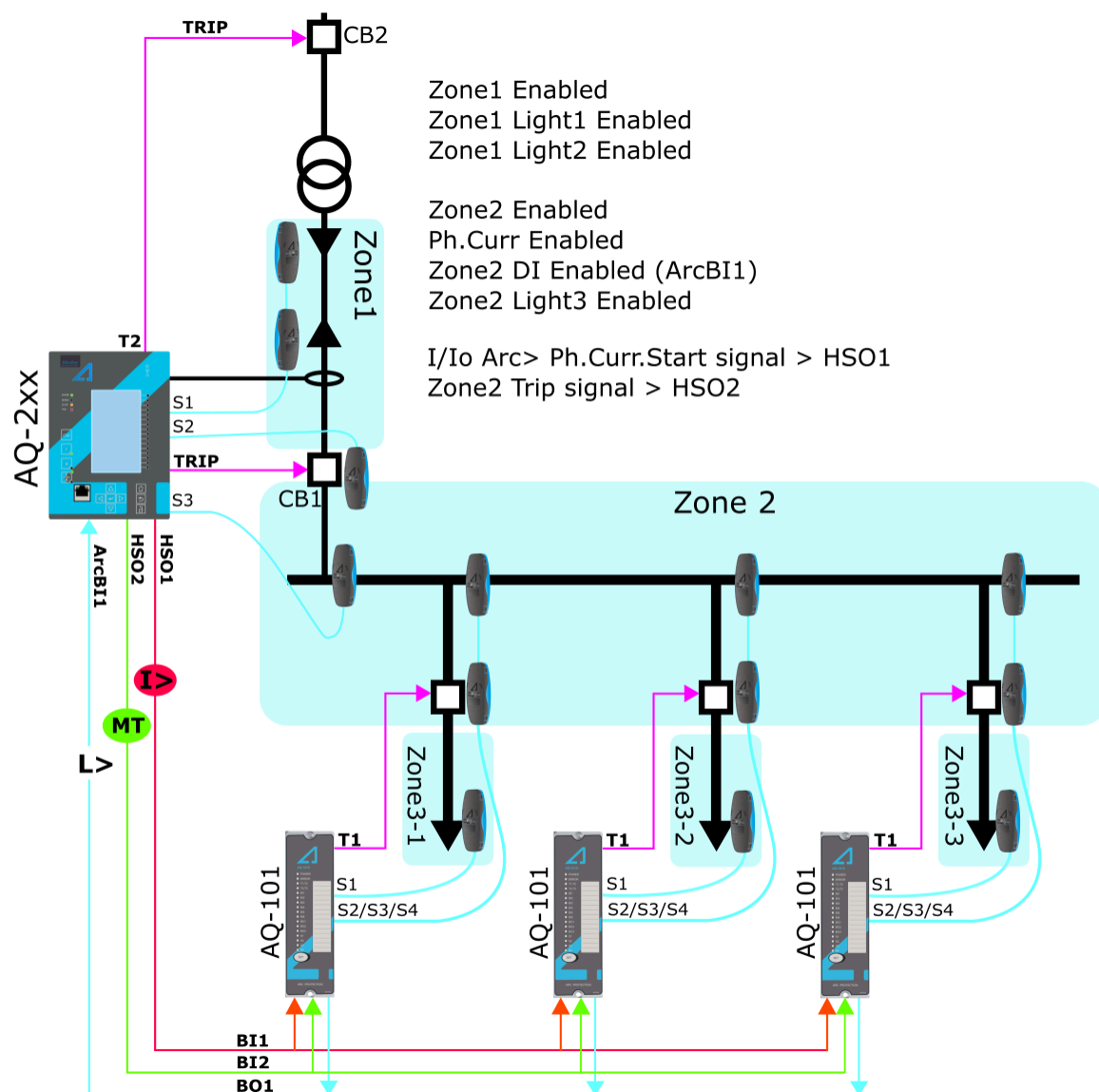
Figure. 4.4.17 - 145. Scheme IA1 (with AQ-101 arc protection relays).
