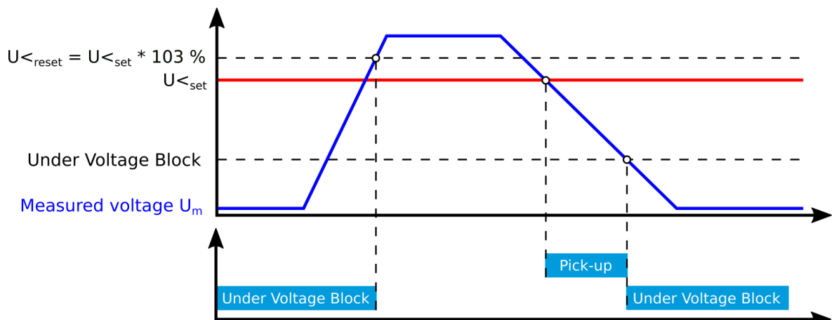
Figure. 4.4.10 - 117. Example of the block setting operation.
