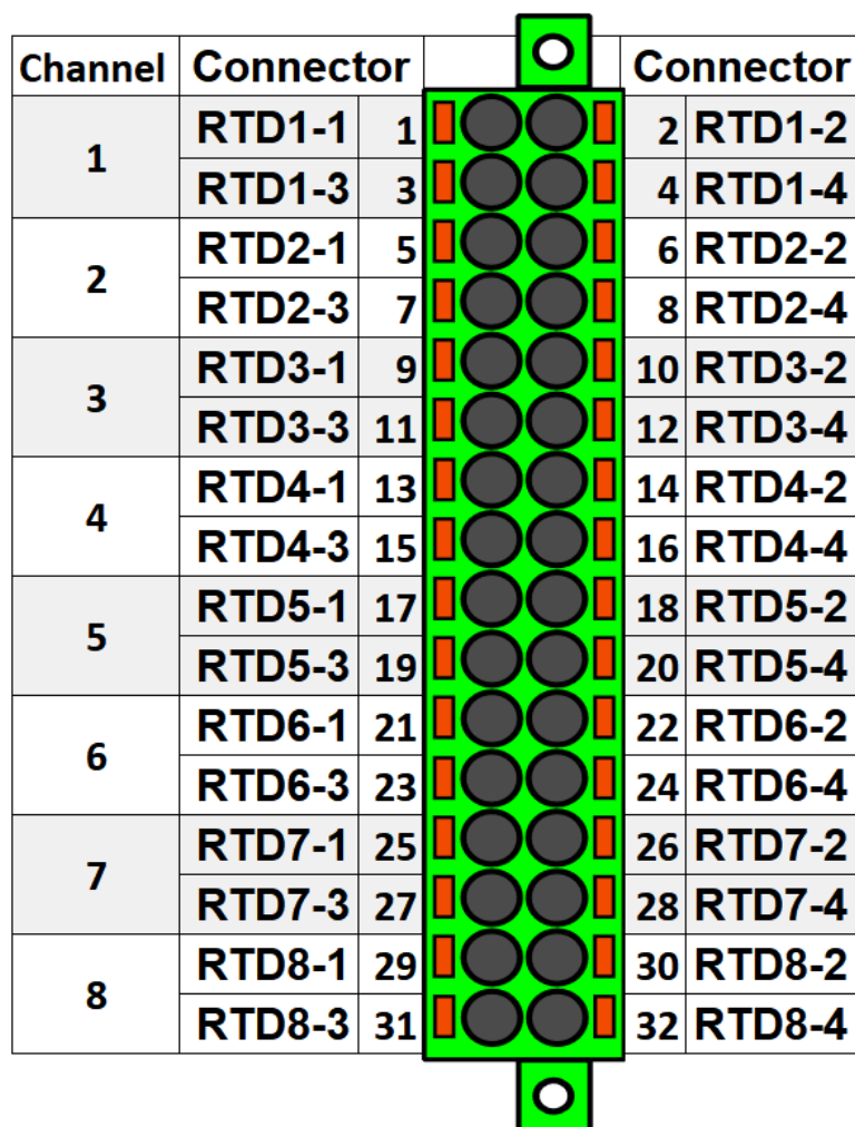
Figure. 7.5.4 - 199. RTD input module connectors.
