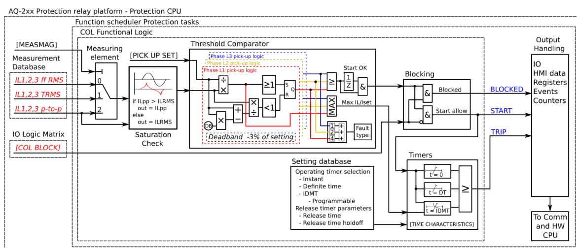
Figure. 4.4.2 - 91. Simplified function block diagram of the Icol> function.
