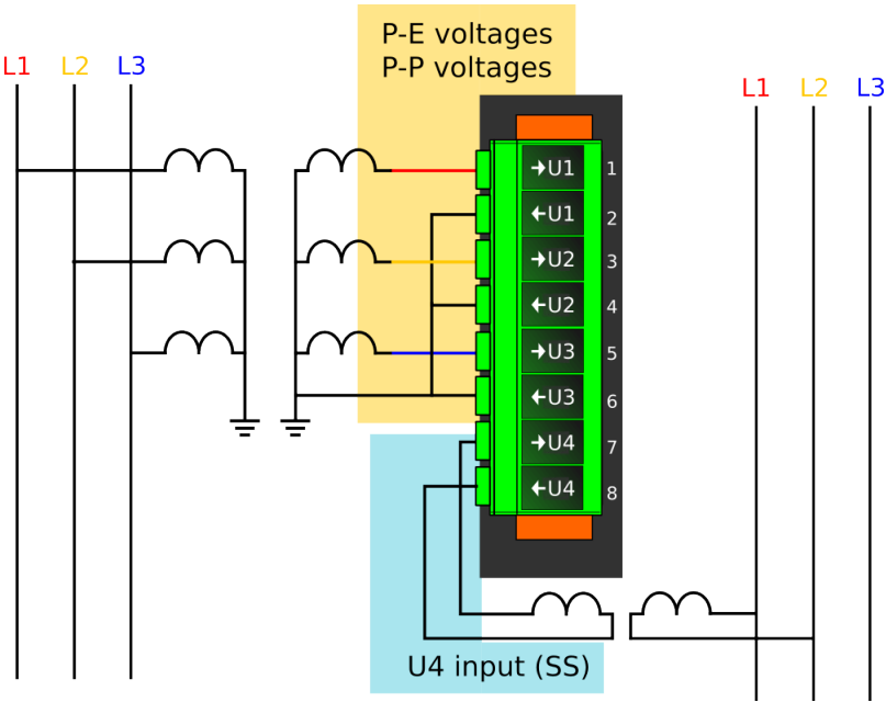
Figure. 4.4.10 - 114. Selectable measurement magnitudes with 3LN+U4 VT connection.
