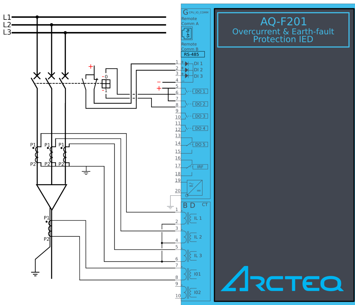
Figure. 6.2 - 142. Application example and its connections.
