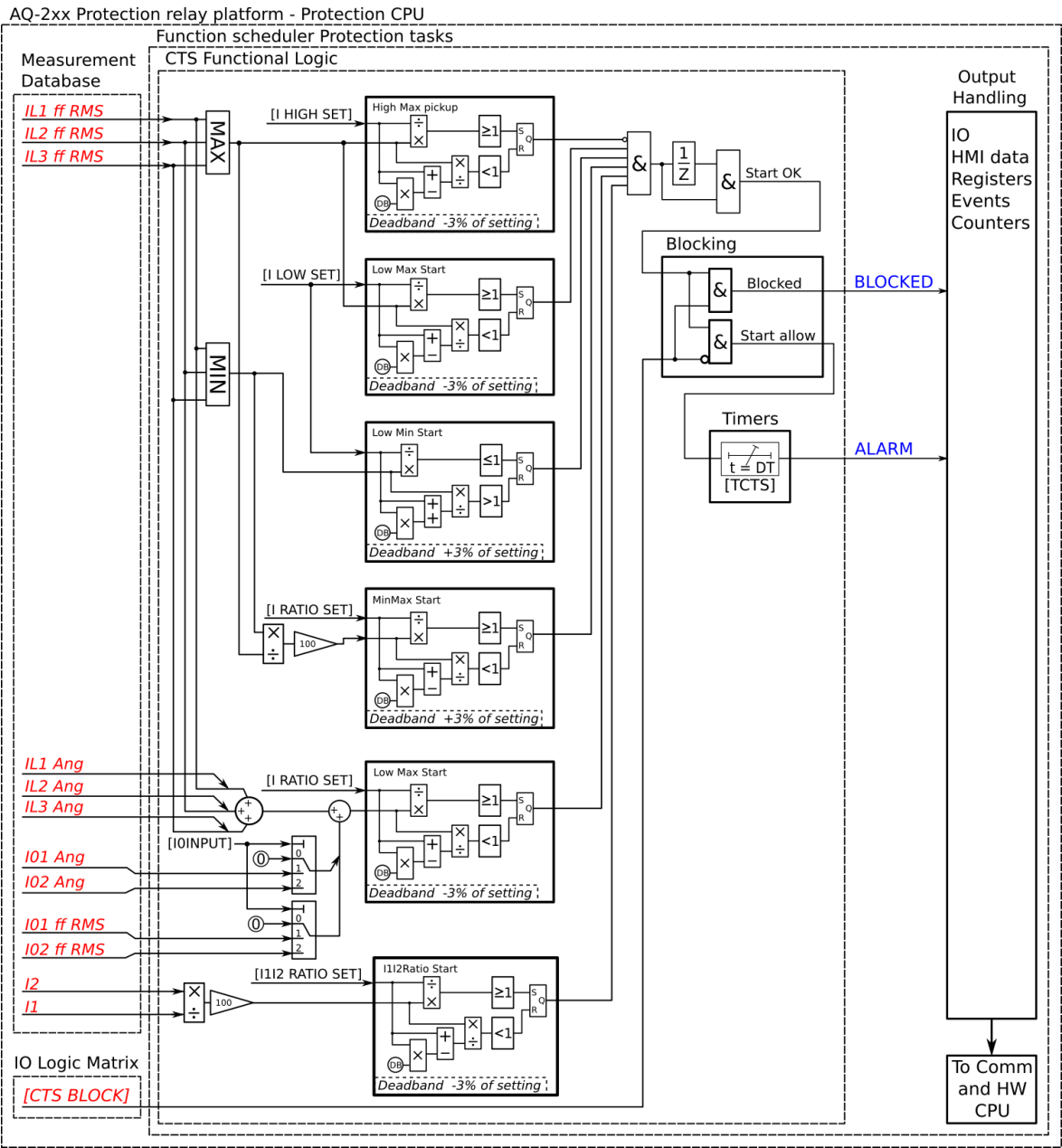
Figure. 4.6.1 - 122. Simplified function block diagram of the CTS function.
