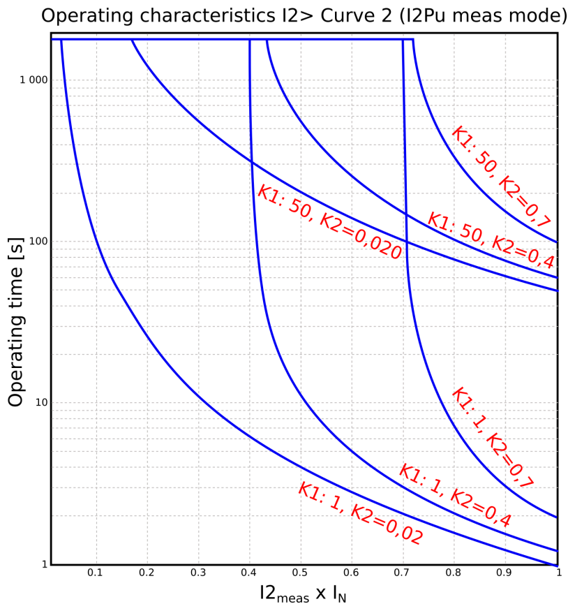
Figure. 4.4.4 - 76. Operation characteristics curve for I_2 > \text{Curve2} .
