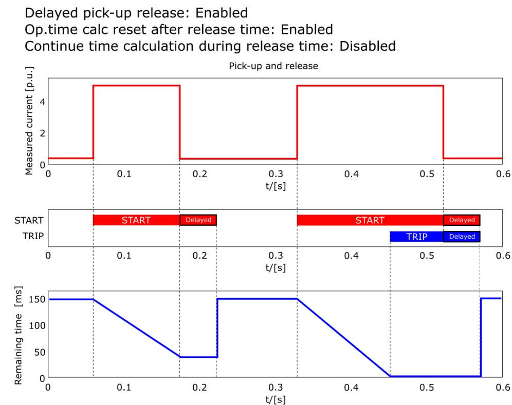
Figure. 4.4.1 - 71. Delayed pick-up release, delay counter value is held during the release time.
