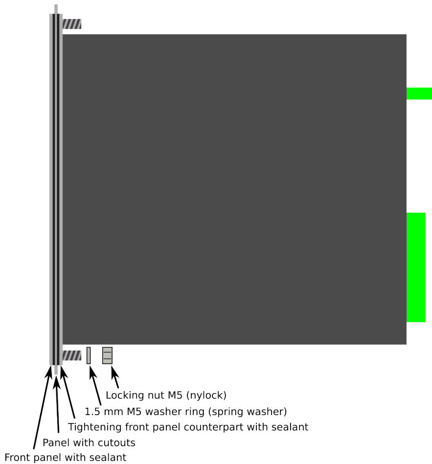
Figure. 7.5 - 153. Device installation.
