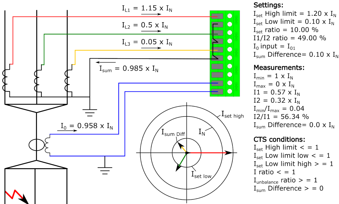
Figure. 4.6.1 - 131. Primary side high-impedance earth fault.
