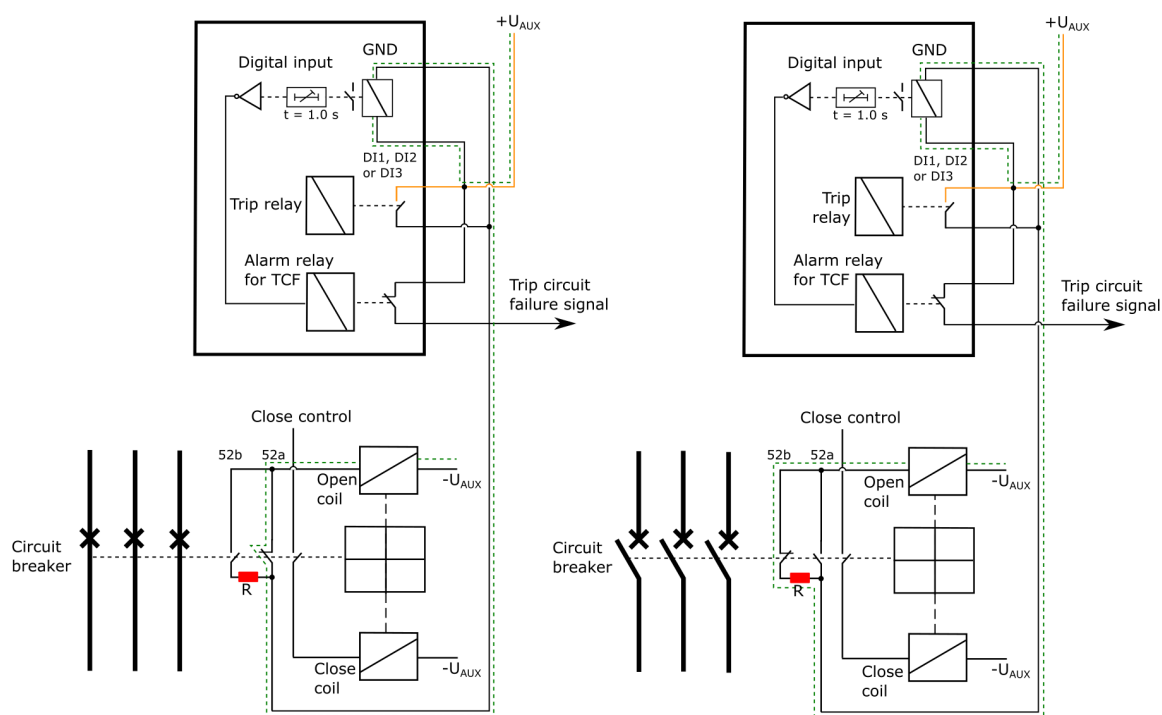
Figure. 6.4 - 144. Trip circuit supervision with one DI and one non-latched trip output.
