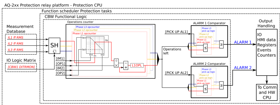
Figure. 4.6.2 - 133. Simplified function block diagram of the circuit breaker wear function.
