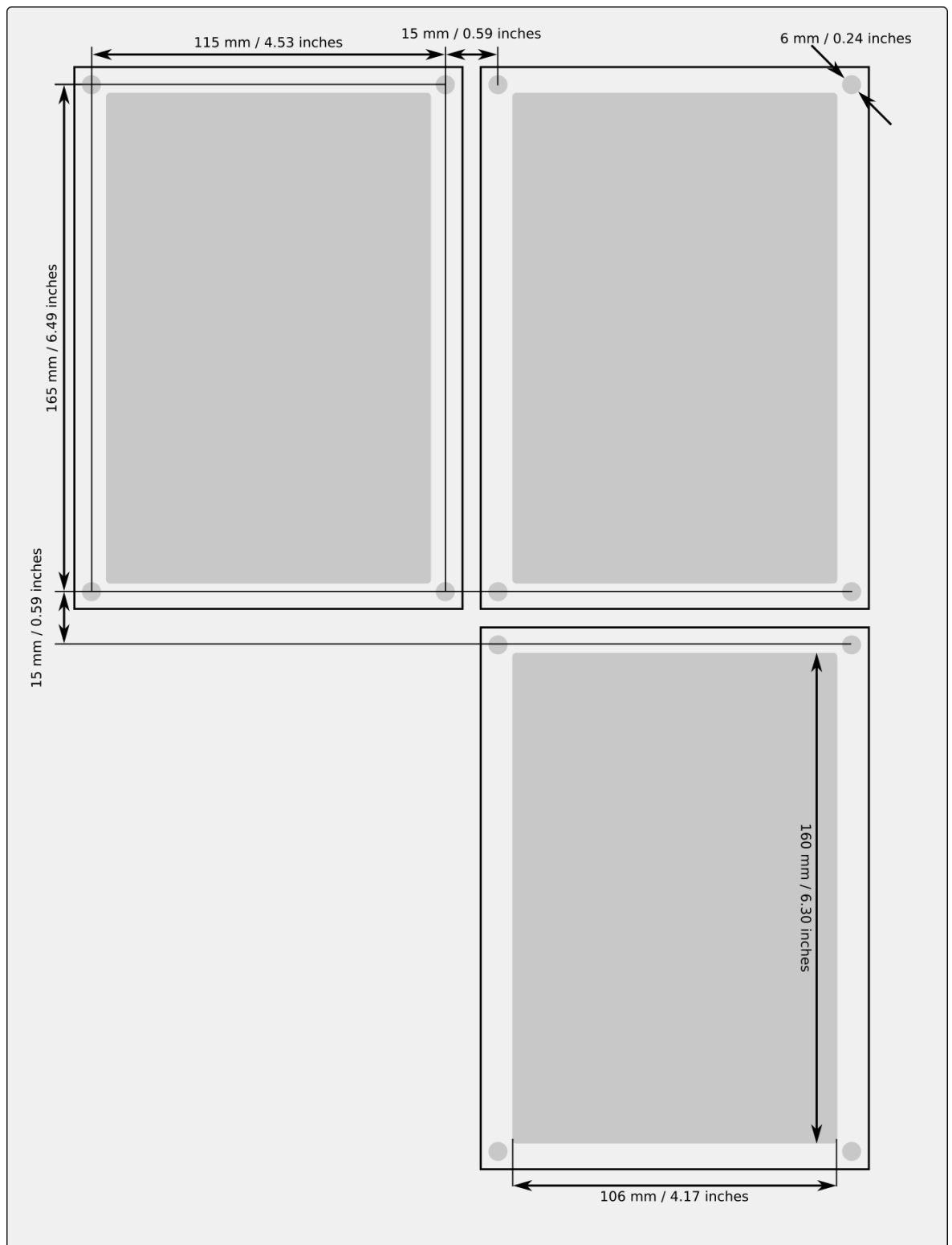
Figure. 7.5 - 154. Panel cutout dimensions and device spacing.
