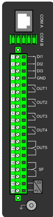
Figure. 7.2 - 150. CPU module.
