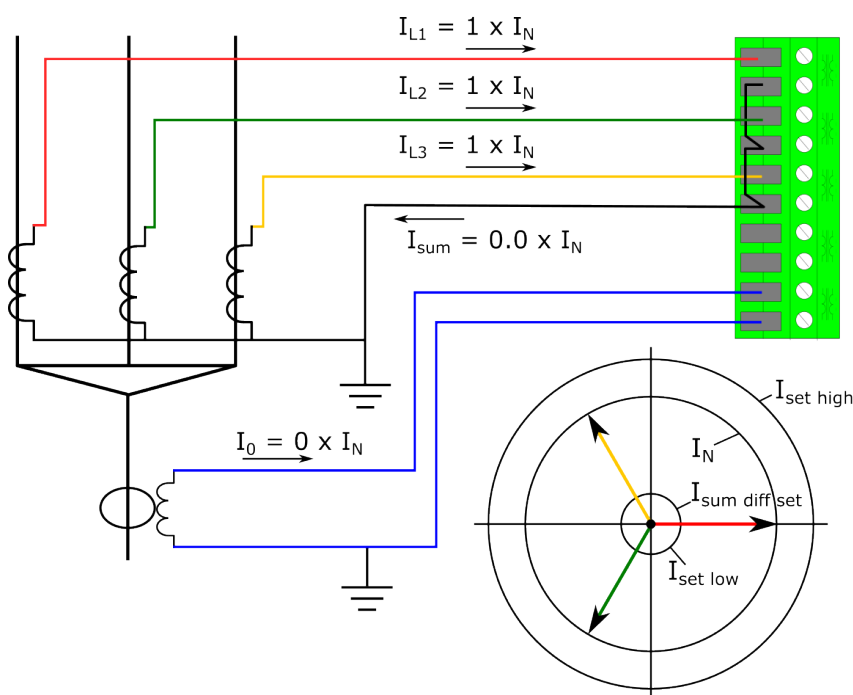
Figure. 4.6.1 - 128. Normal situation, residual current also measured.
