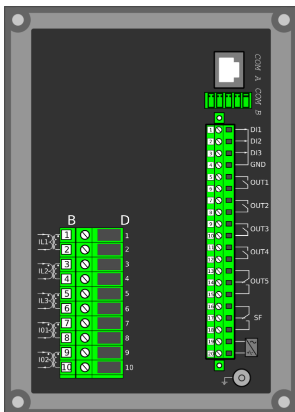
Figure. 7.1 - 149. Connections and modules in AQ-F201.
