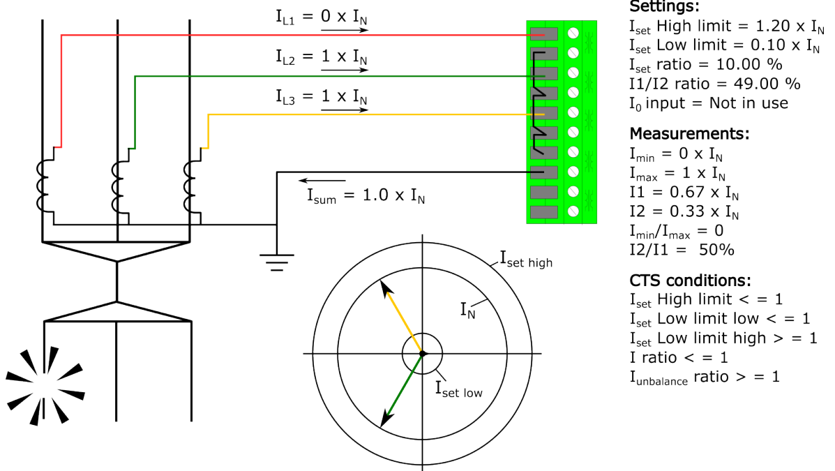
Figure. 4.6.1 - 125. Primary circuit fault in phase L1 wiring.
