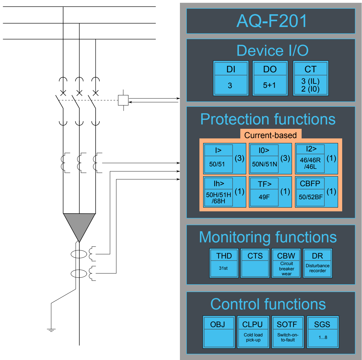
Figure. 6.1 - 141. AQ-F201 application example with function block diagram.
