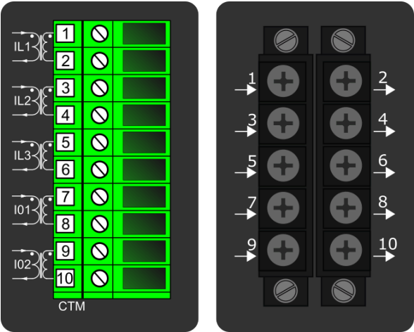
Figure. 7.3 - 151. Module connections with standard and ring lug terminals.
