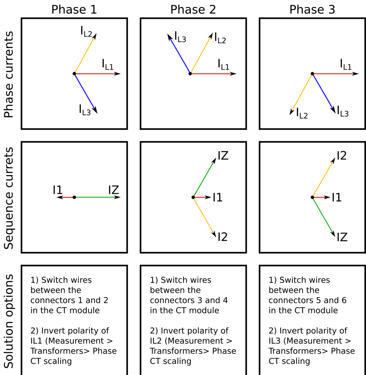
Figure. 4.2.1 - 62. Common phase polarity problems.
