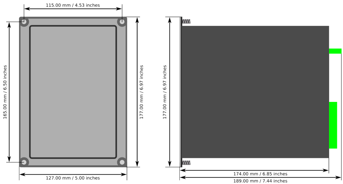
Figure. 7.5 - 152. Device dimensions.
