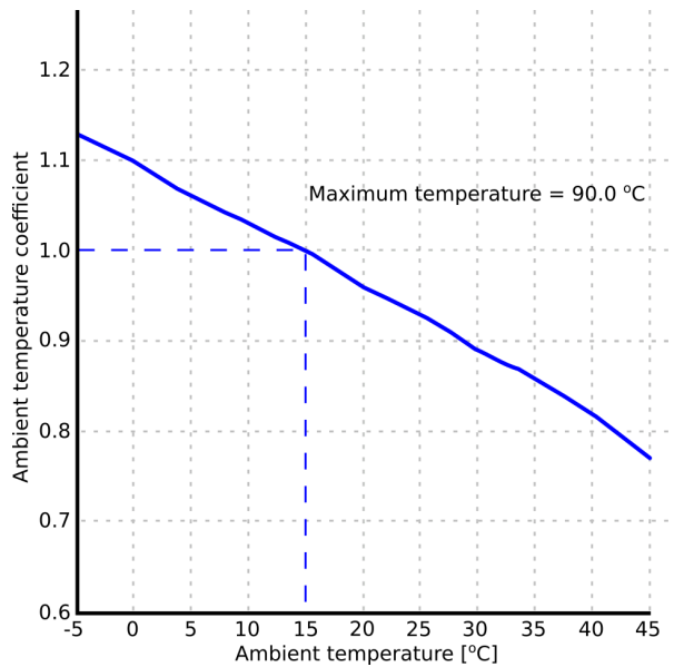
Figure. 4.4.19 - 164. Set correction curve for ambient temperature.
