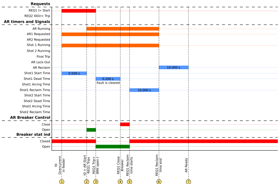
Figure. 4.5.5 - 195. Signal status graph of the transient overcurrent auto-recloser cycle.
