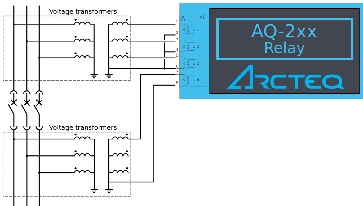
Figure. 4.5.8 - 207. Example connection of the synchrocheck function (3LN+U4 mode, SYN1 in use, UL1 as reference voltage).
