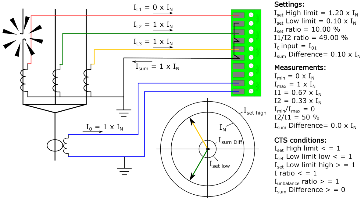
Figure. 4.6.1 - 229. Broken primary phase current wiring.
