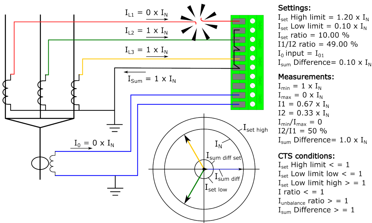
Figure. 4.6.1 - 228. Broken secondary phase current wiring.
