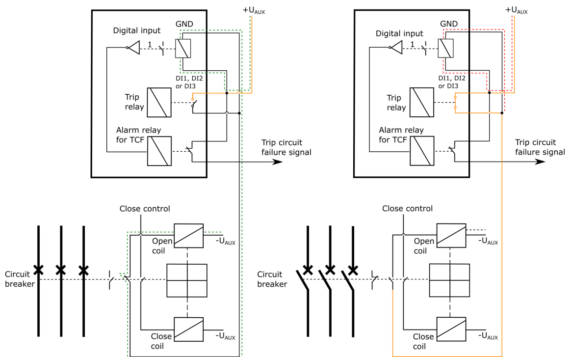
Figure. 6.4 - 248. Trip circuit supervision with one DI and one latched output contact.
