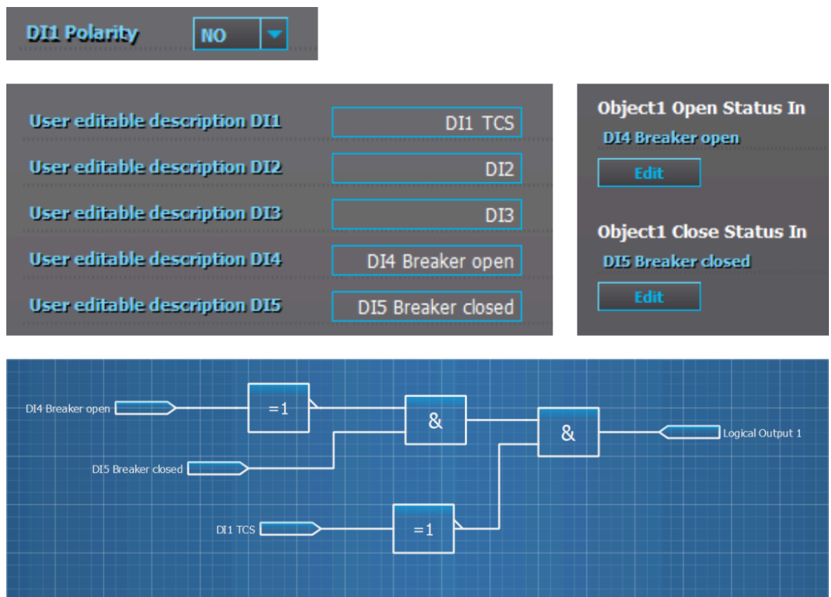
Figure. 6.4 - 249. Example block scheme.
