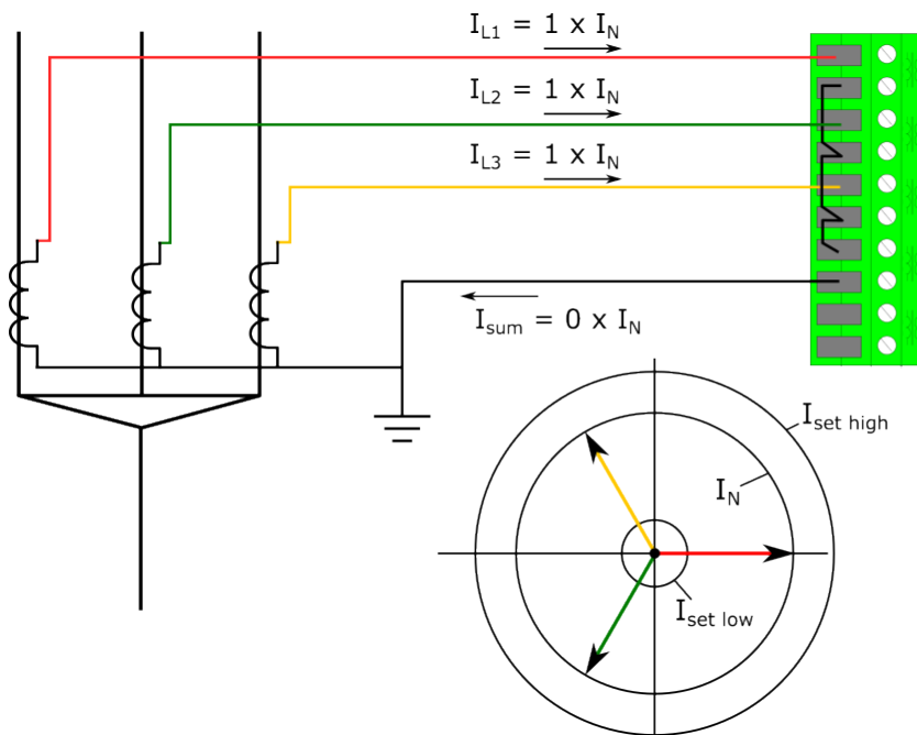
Figure. 4.6.1 - 222. All works properly, no faults.
