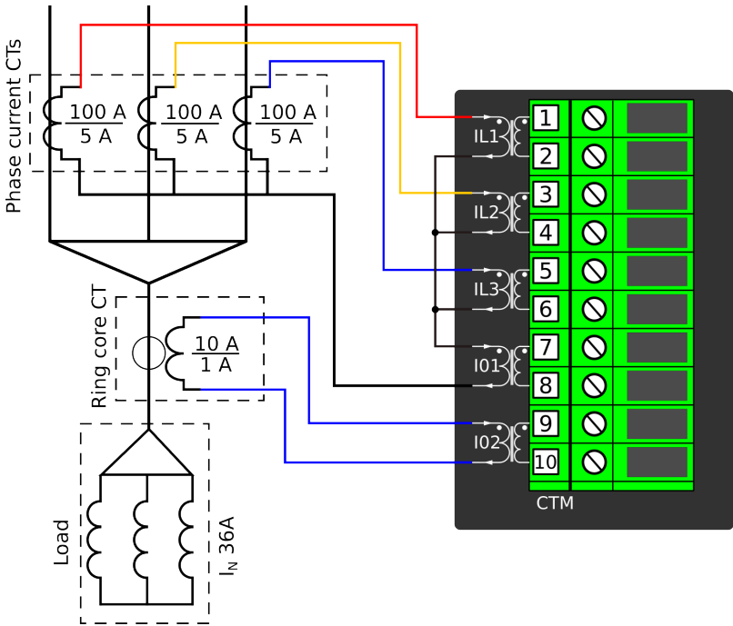
Figure. 4.2.1 - 58. Connections.
