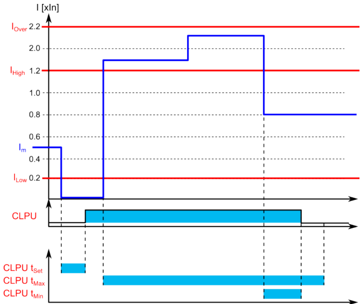
Figure. 4.5.6 - 200. Example of timers and pick-up parameters (normal CLPU situation).
