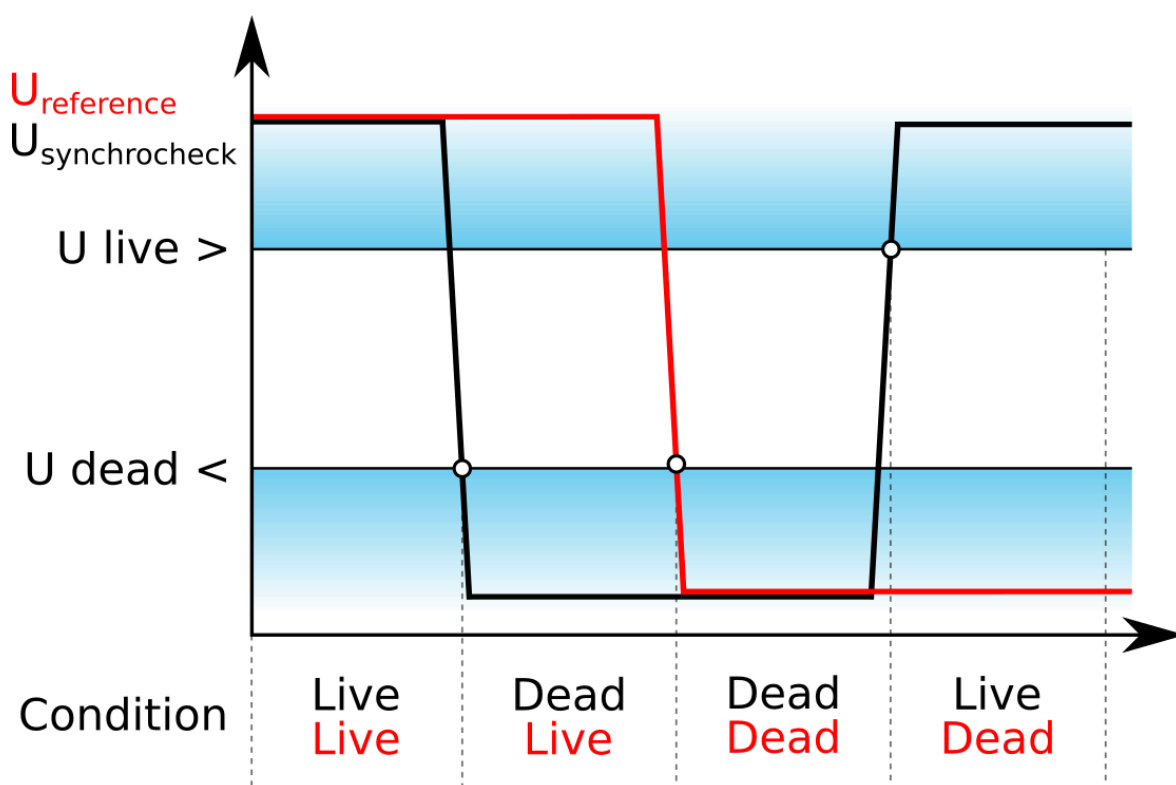
Figure. 4.5.8 - 214. System states.
