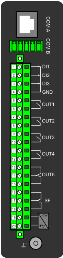
Figure. 7.2 - 251. CPU module.
