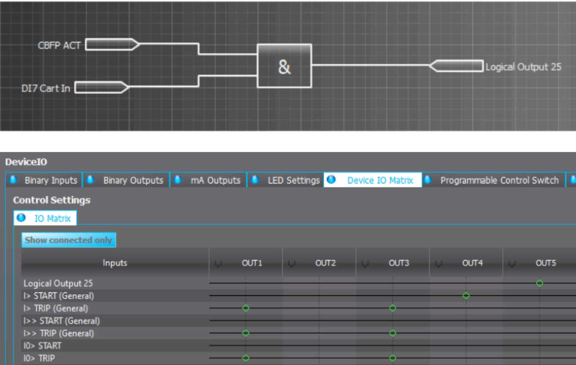
Figure. 4.5.11 - 217. Logic output example. Logical output is connected to an output relay in matrix.
