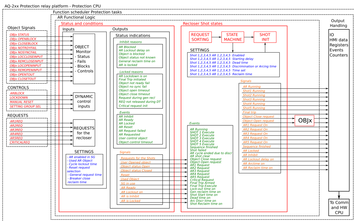
Figure. 4.5.5 - 197. Simplified function block diagram of the auto-recloser function.
