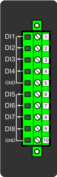
Figure. 7.5.1 - 254. Digital input module (DI8) with eight add-on digital inputs.
