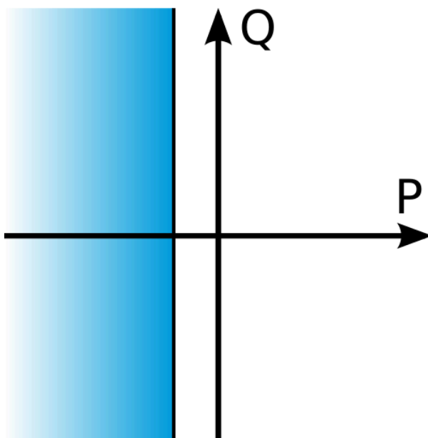
Figure. 4.4.18 - 158. Operating characteristics of reverse power protection.
