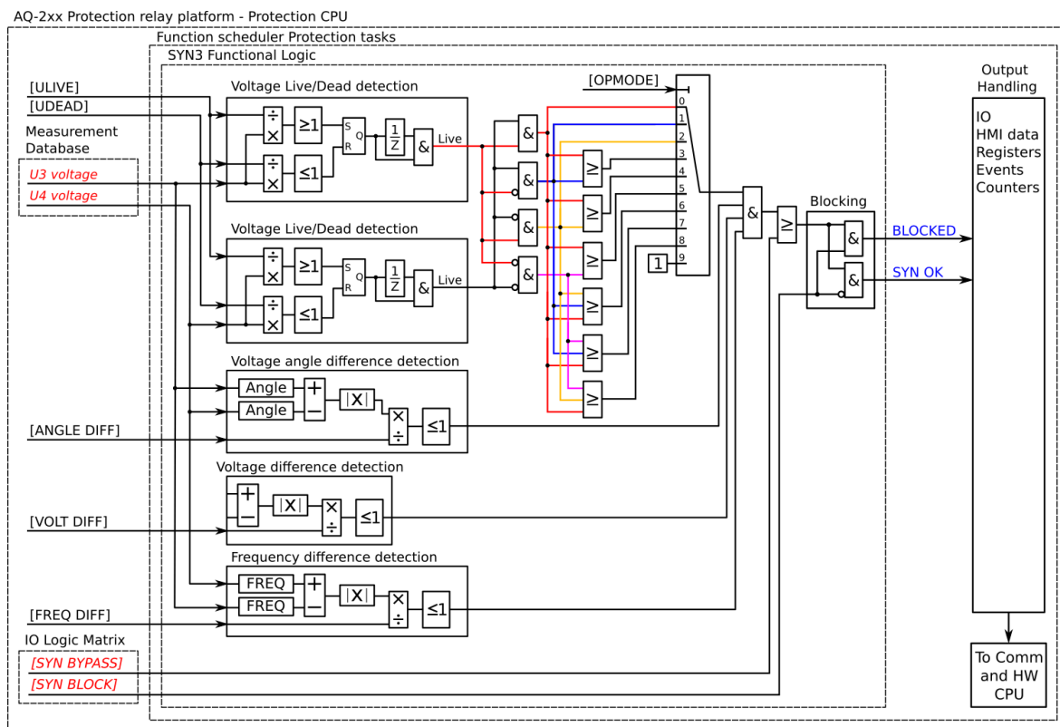
Figure. 4.5.8 - 216. Simplified function block diagram of the SYN3 function.
