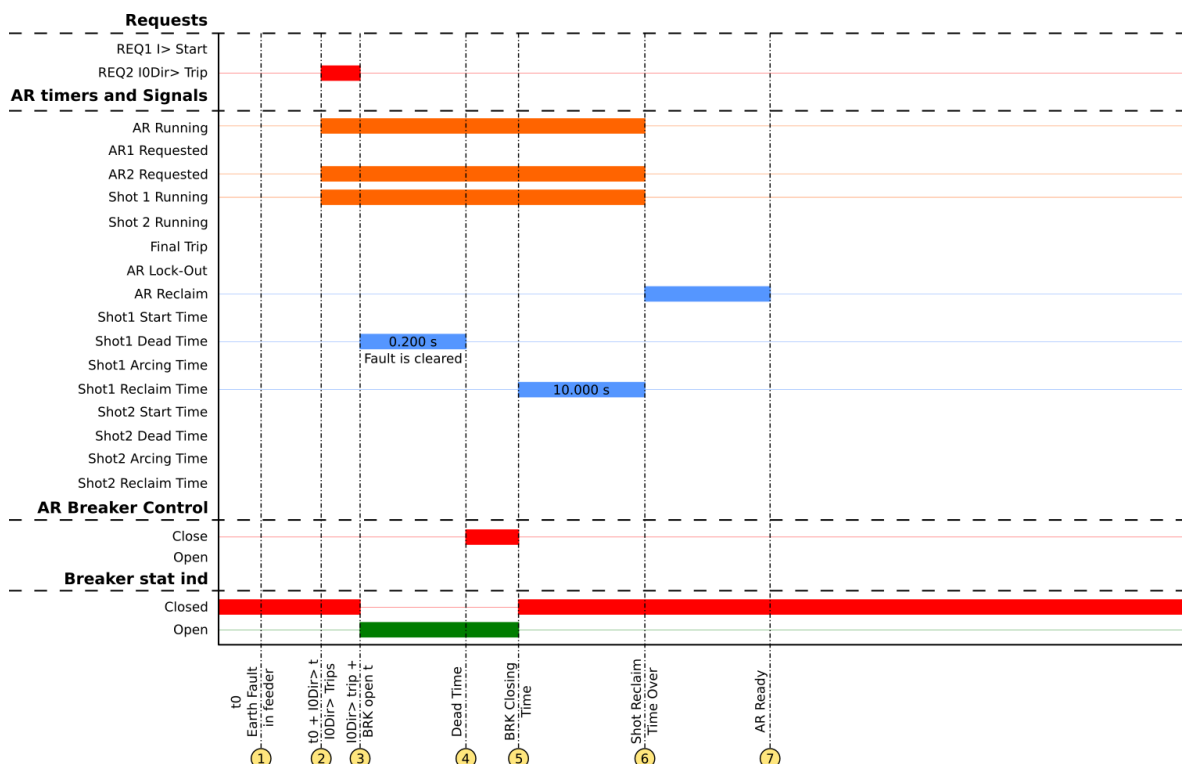
Figure. 4.5.5 - 189. Signal status graph of the transient earth fault auto-recloser cycle.
