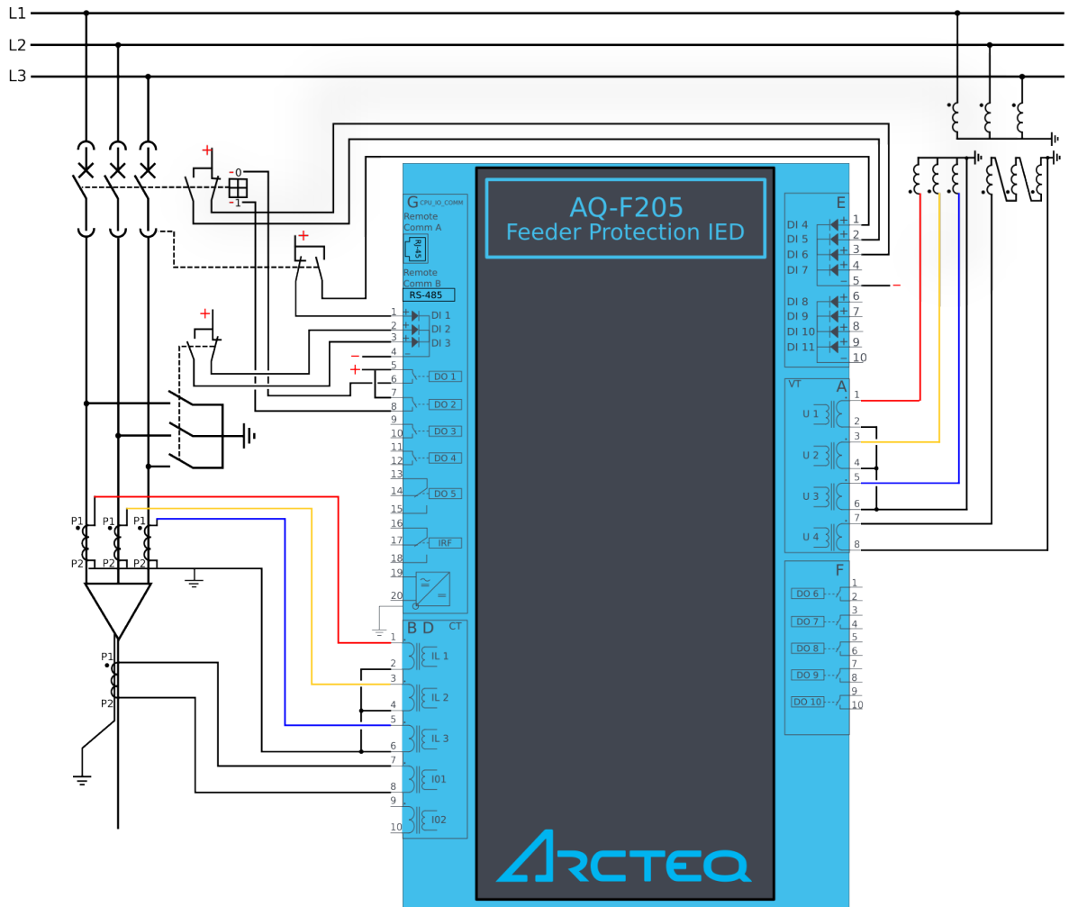
Figure. 6.2 - 243. Application example and its connections.
