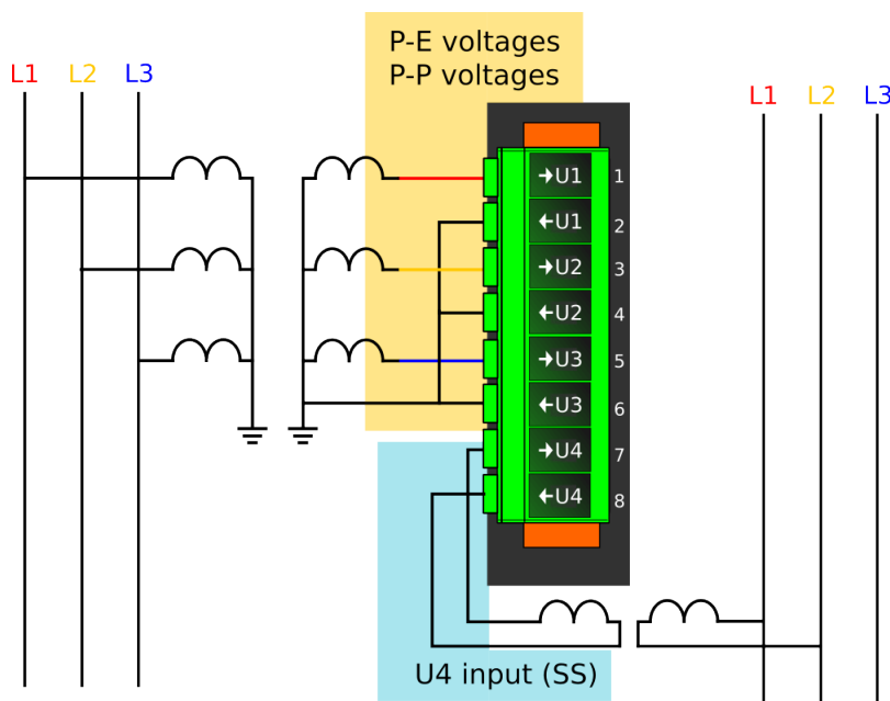
Figure. 4.4.10 - 129. Selectable measurement magnitudes with 3LN+U4 VT connection.
