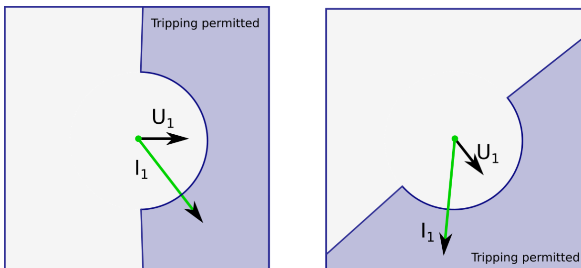
Figure. 4.4.4 - 94. Angle tracking of the I_{dir} function (3LN/3LL + U_0 mode).
