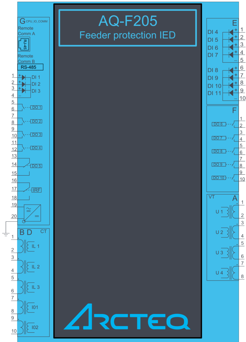
Figure. 6.1 - 241. AQ-F205 connections. AQ-F205 has fixed hardware with digital input and output cards always included.
