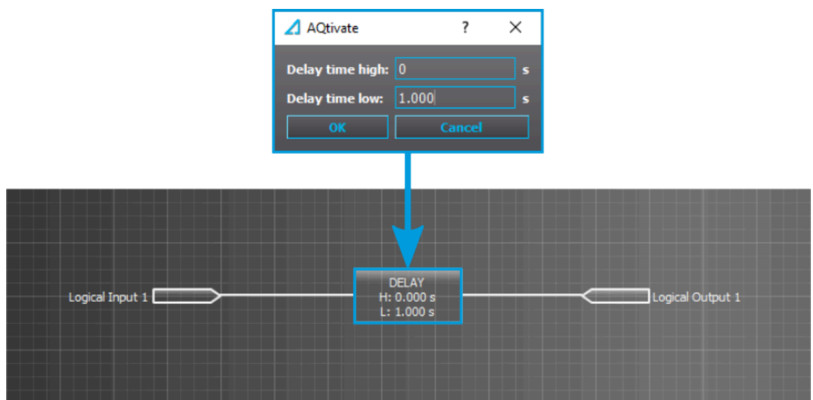
Figure. 4.5.12 - 219. Extending a logical input pulse.
