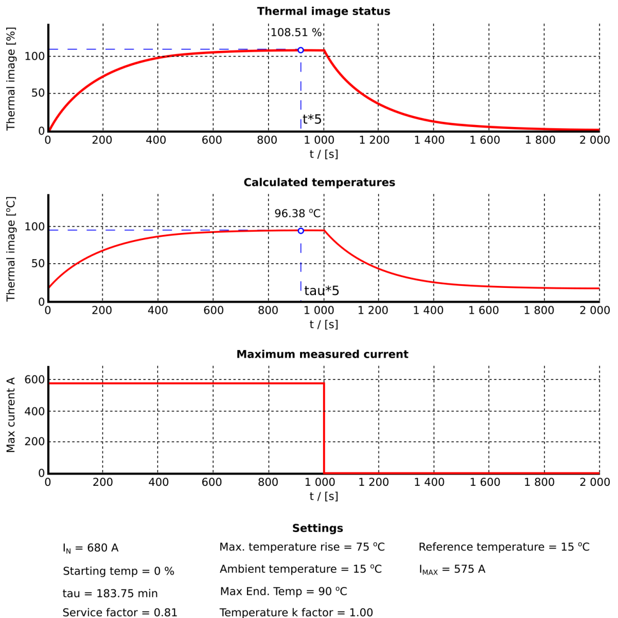
Figure. 4.4.19 - 170. Thermal image response with nominal currents and fine-tuned k_{\text{SF}} correction factor.
