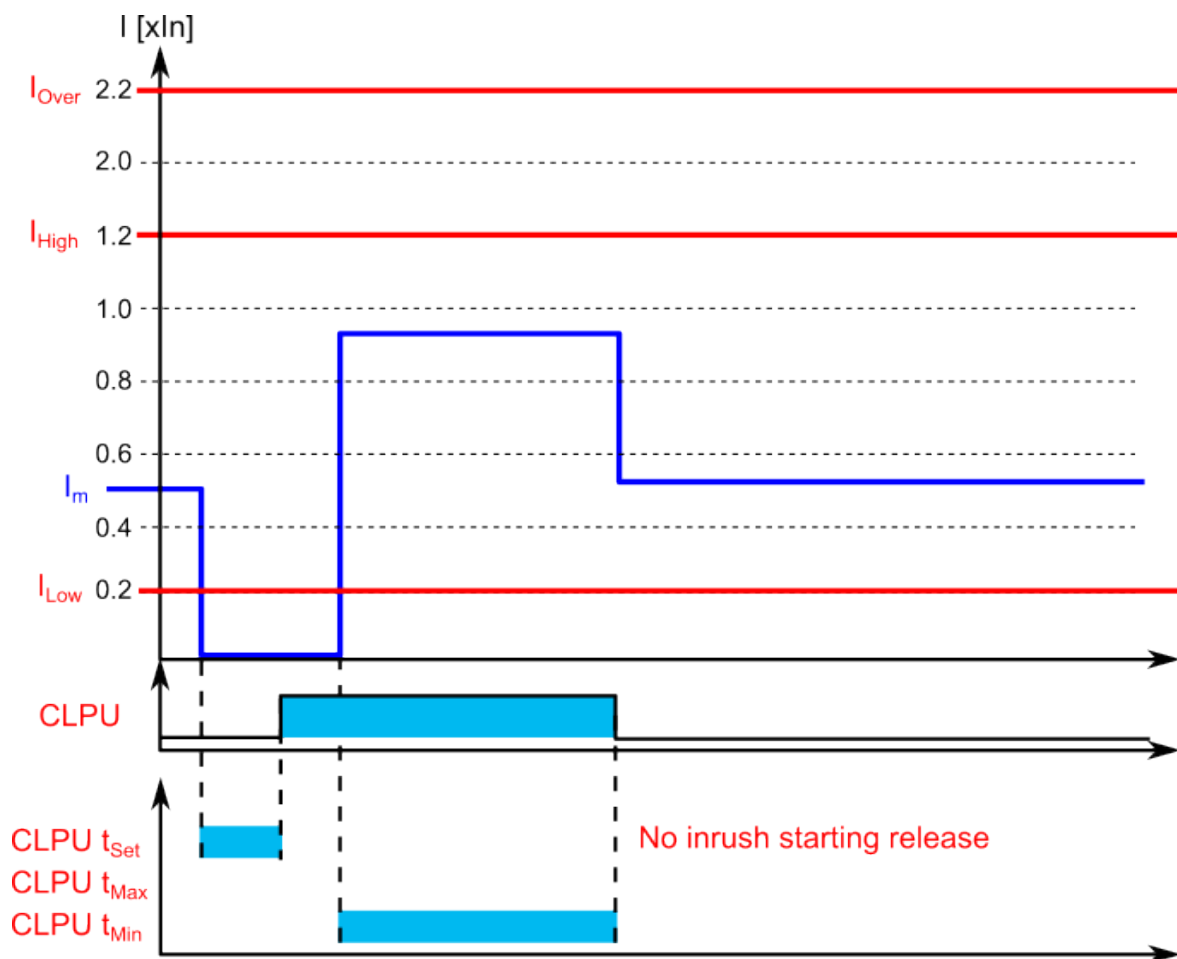
Figure. 4.5.6 - 204. Example of timers and pick-up parameters (no inrush current detected in the starting).
