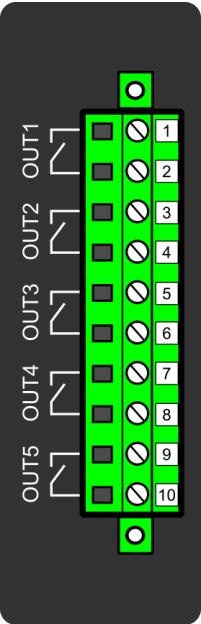
Figure. 7.5.2 - 256. Digital output module (DO5) with five add-on digital outputs.
