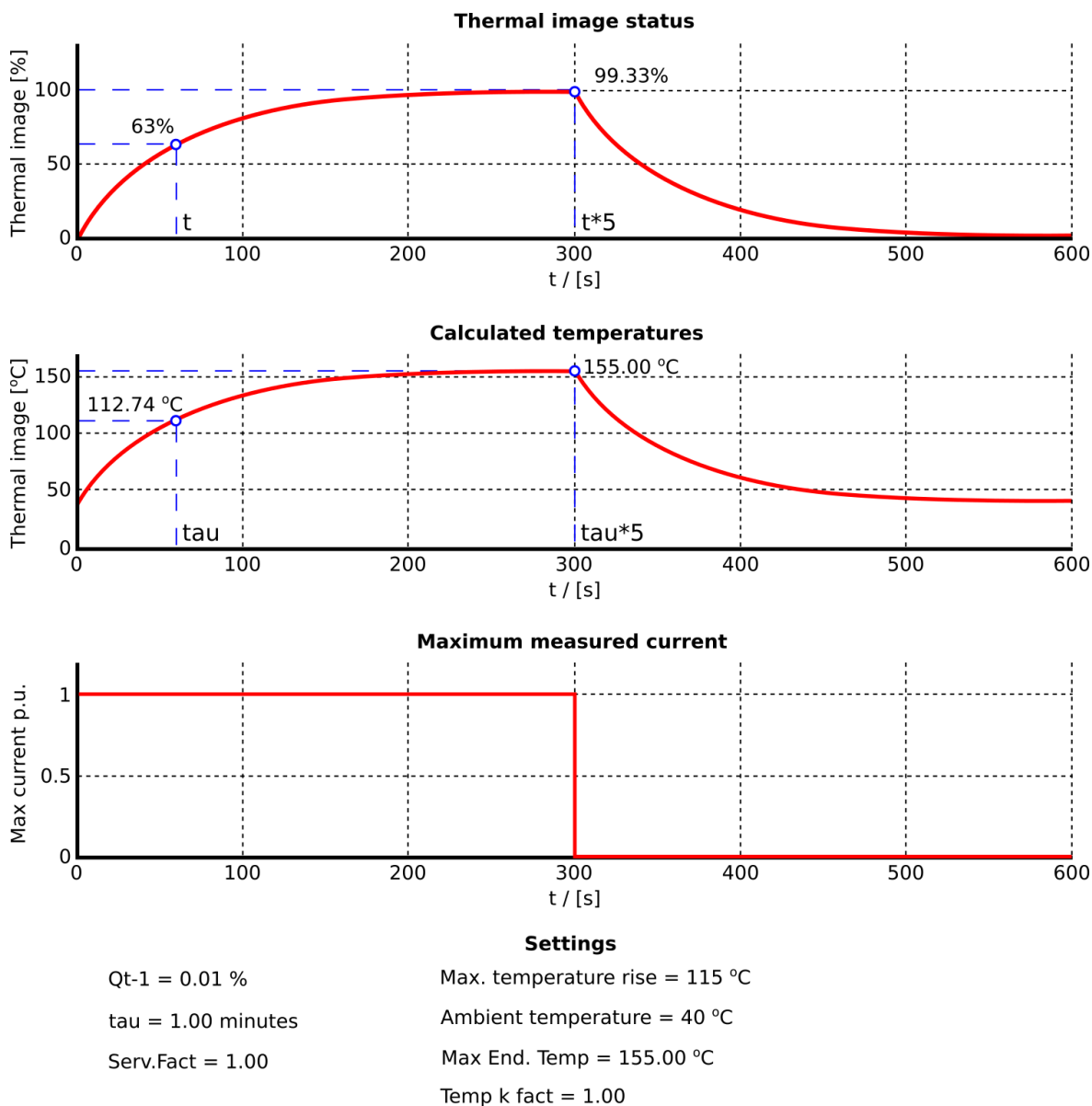
Figure. 4.4.19 - 160. Example of thermal image calculation with nominal conditions.
