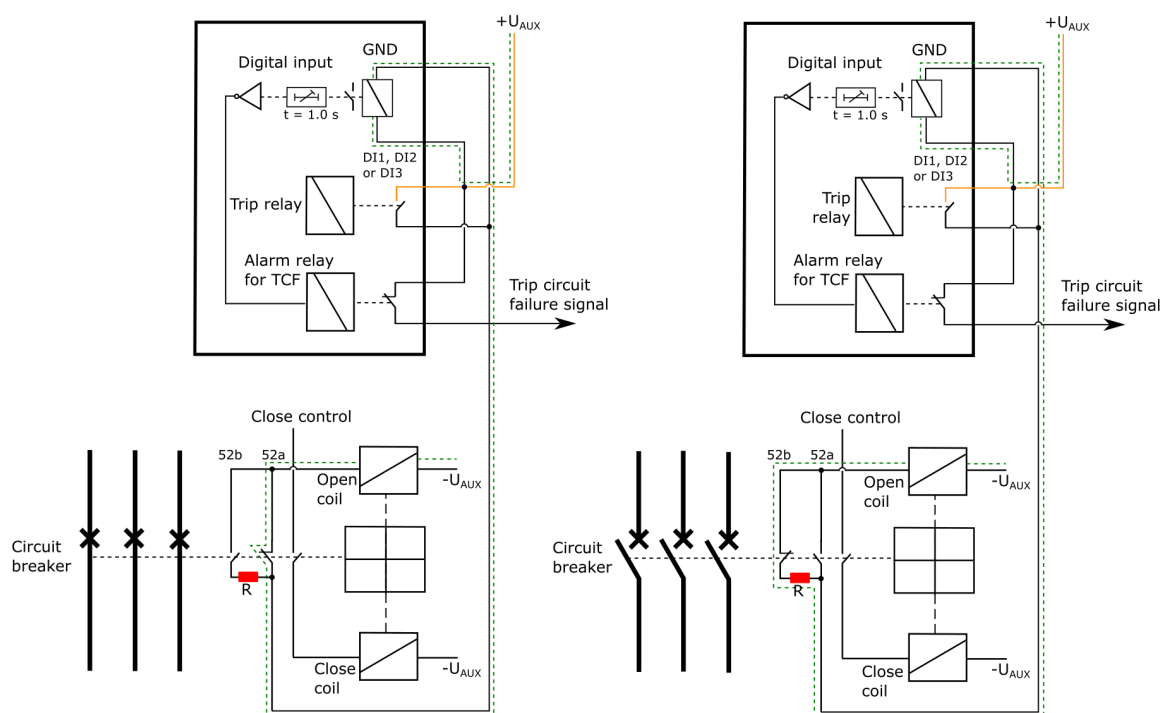
Figure. 6.4 - 245. Trip circuit supervision with one DI and one non-latched trip output.
