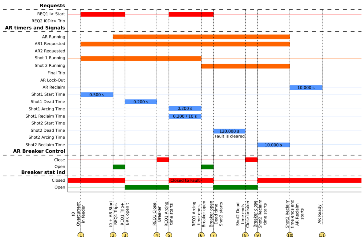
Figure. 4.5.5 - 193. Signal status graph of the semi-permanent overcurrent auto-recloser cycle.
