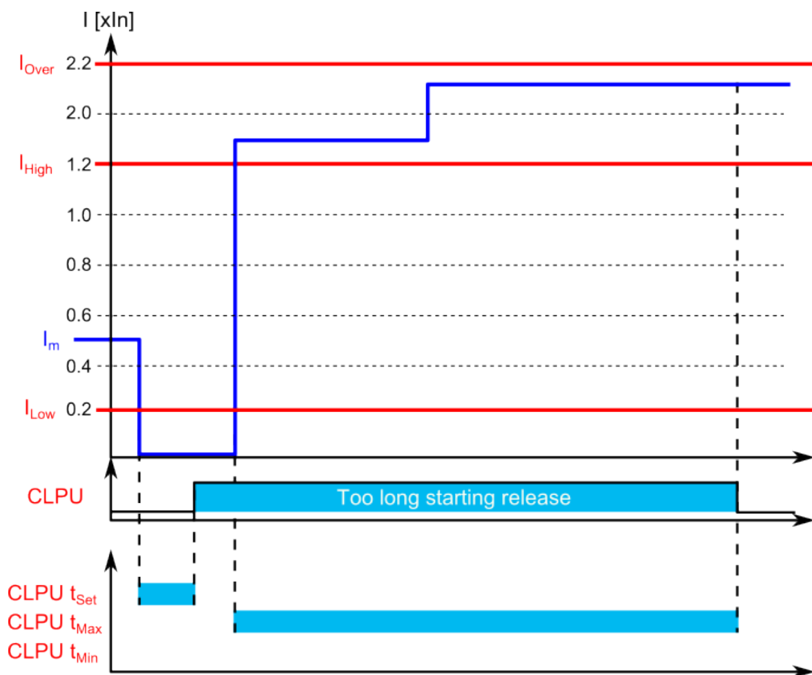
Figure. 4.5.6 - 203. Example of timers and pick-up parameters (activated pick-up and instant release due to too long starting).
