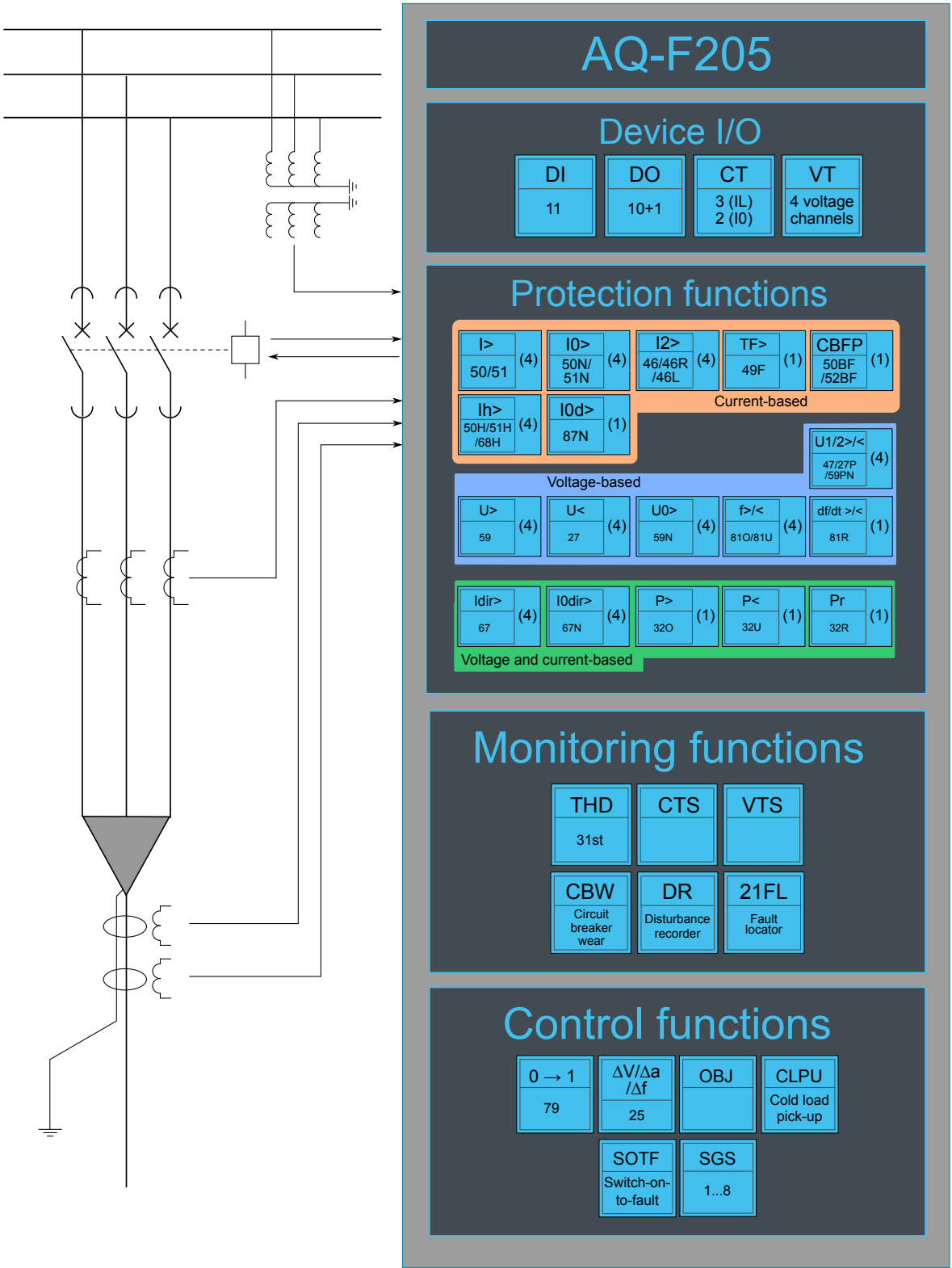
Figure. 6.1 - 242. AQ-F205 application example with function block diagram.
