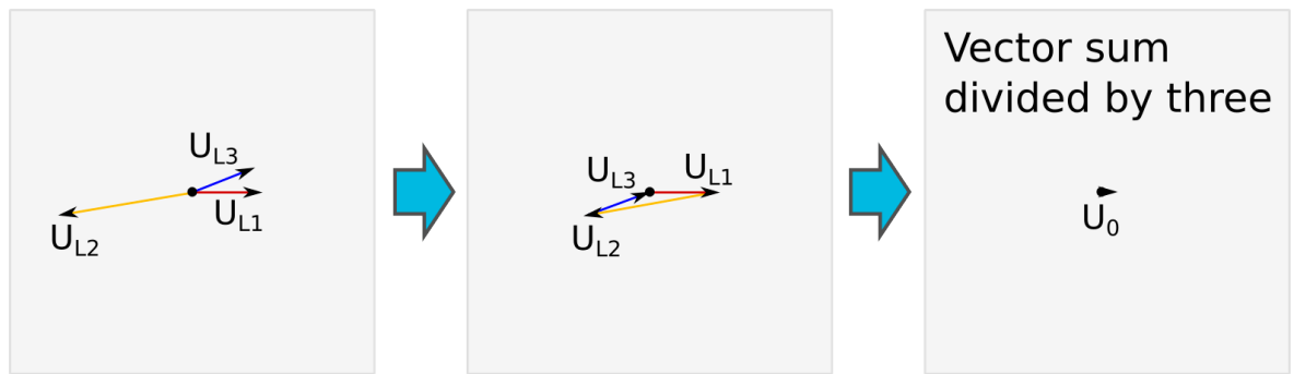
Figure. 4.4.12 - 139. Close-distance short-circuit between phases 1 and 3.
