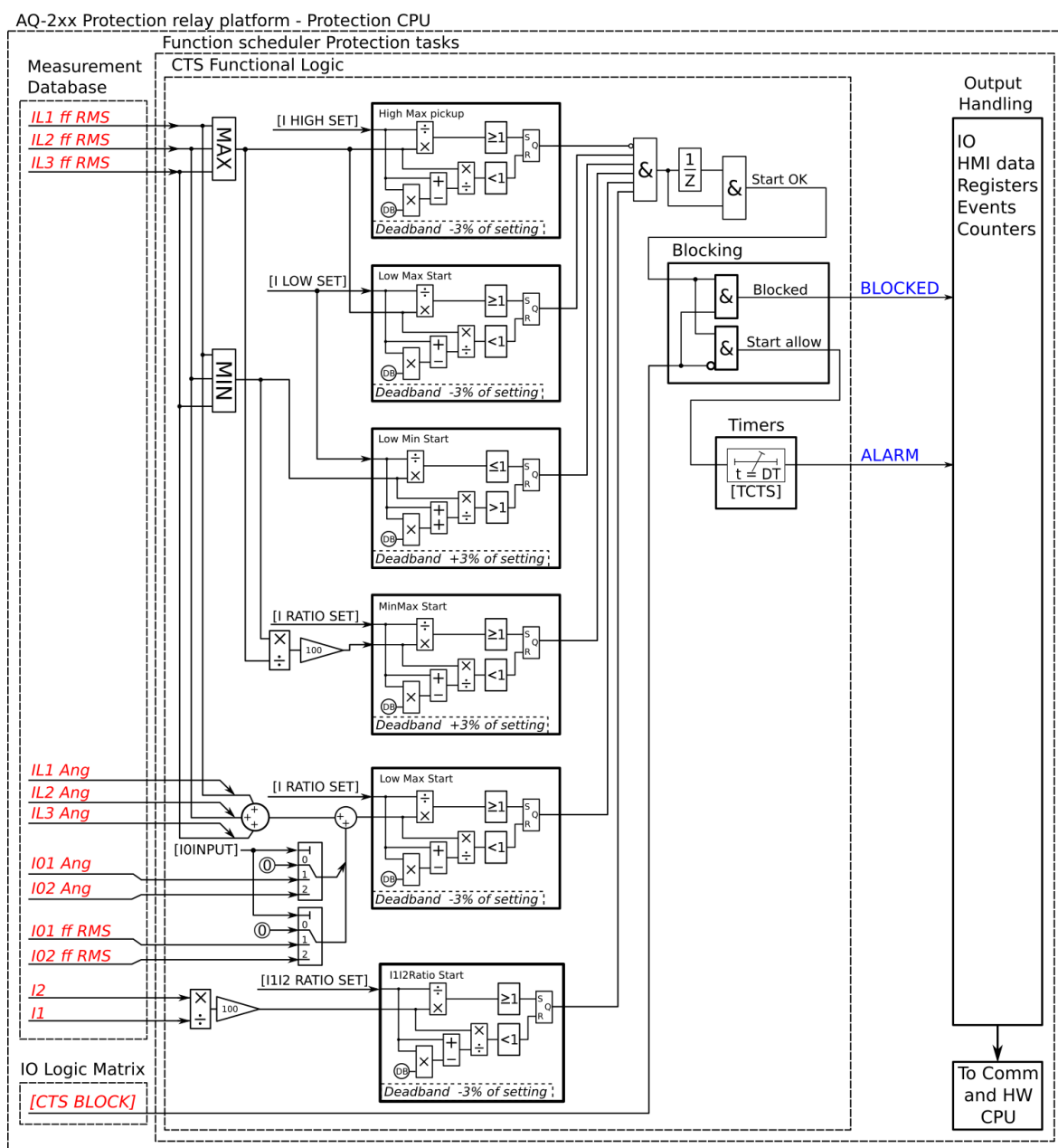
Figure. 4.6.1 - 221. Simplified function block diagram of the CTS function.
