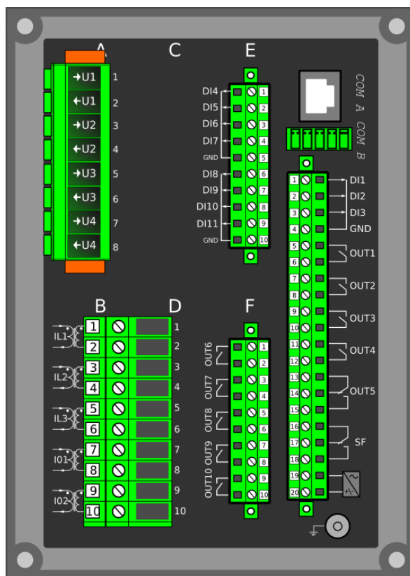
Figure. 7.1 - 250. Modular construction of AQ-F205.
