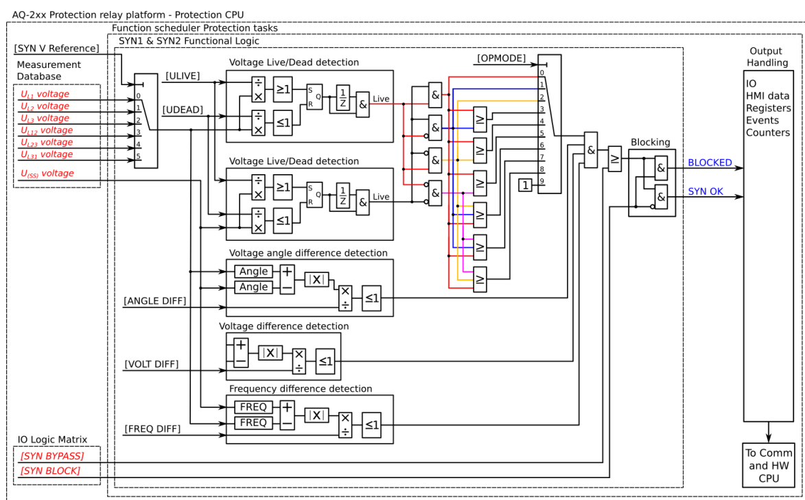
Figure. 4.5.8 - 215. Simplified function block diagram of the SYN1 and SYN2 function.
