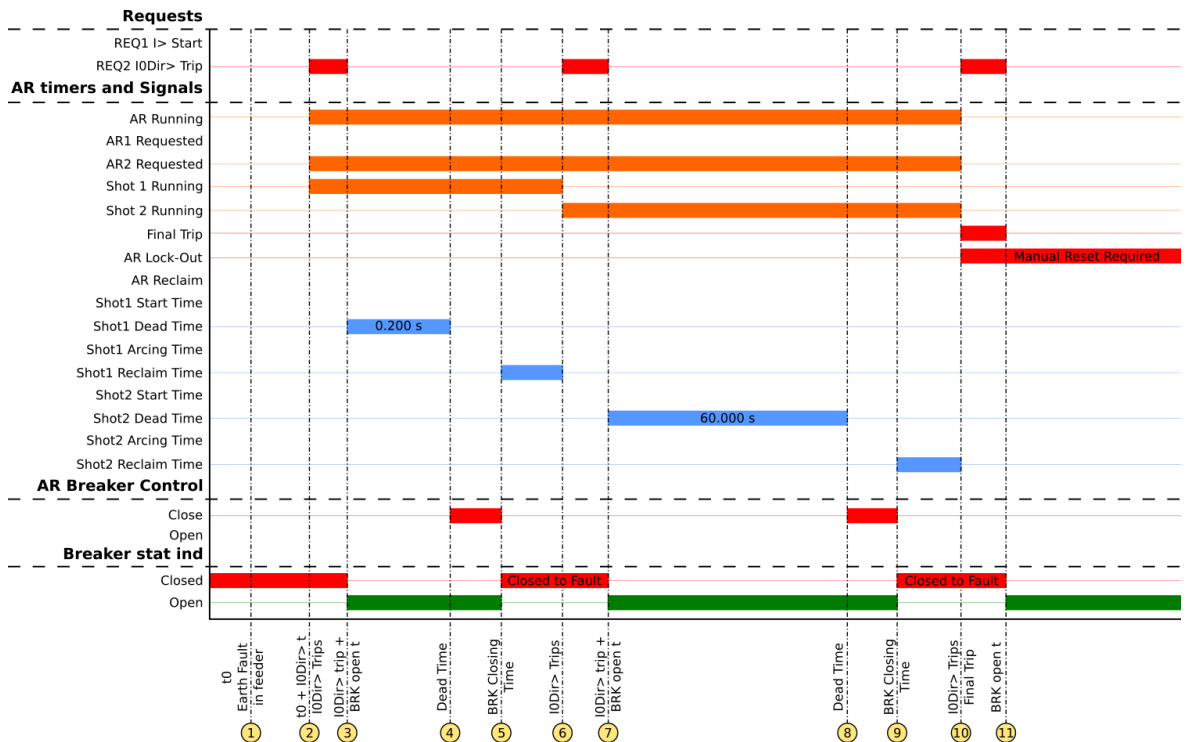
Figure. 4.5.5 - 185. Signal status graph of the permanent earth fault auto-recloser cycle.
