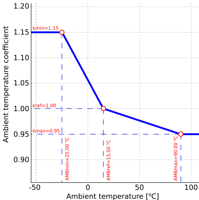
Figure. 4.4.19 - 161. Ambient temperature coefficient calculation (a three-point linear approximation and a settable correction curve).
