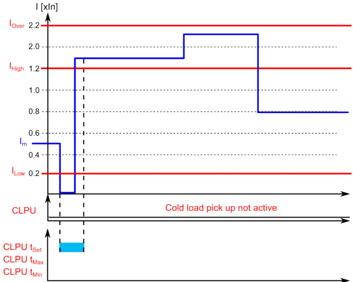
Figure. 4.5.6 - 201. Example of timers and pick-up parameters (no cold load pick-up, I_{low} too short).
