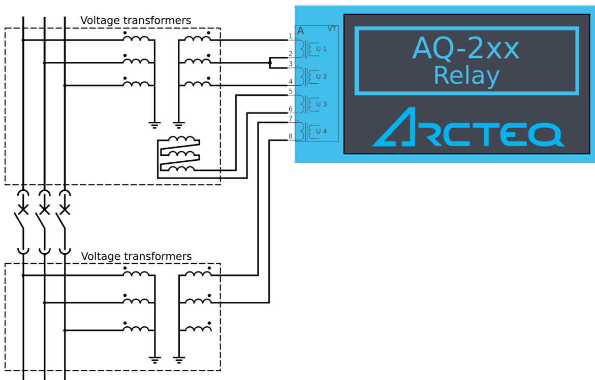
Figure. 4.5.8 - 208. Example connection of the synchrocheck function (2LL+U0+U4 mode, SYN1 in use, UL12 as reference voltage).
