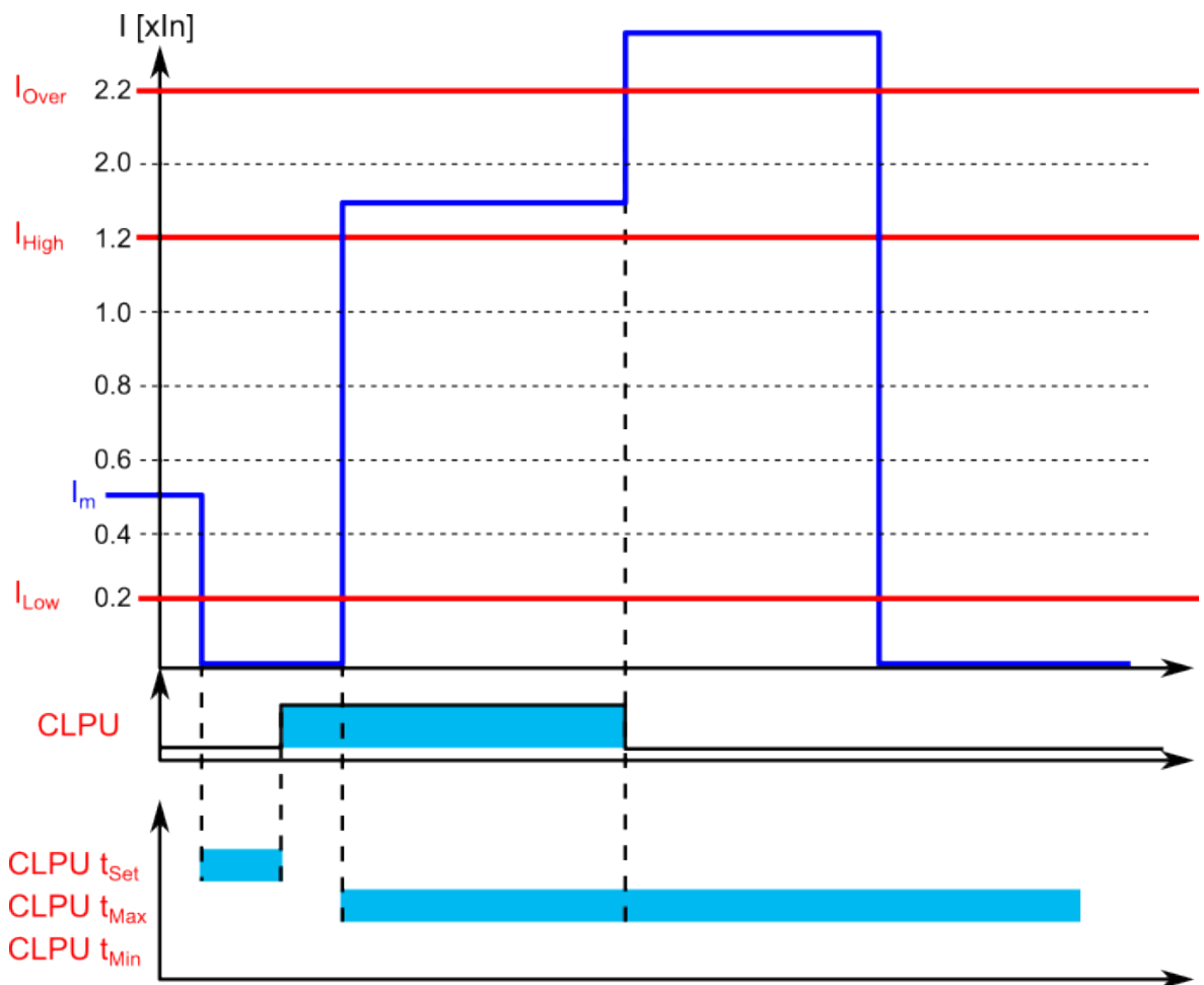
Figure. 4.5.6 - 202. Example of timers and pick-up parameters (activated pick-up and instant release due to overcurrent).
