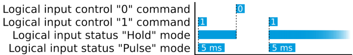
Figure. 4.5.12 - 218. Operation of logical input in "Hold" and "Pulse" modes.
