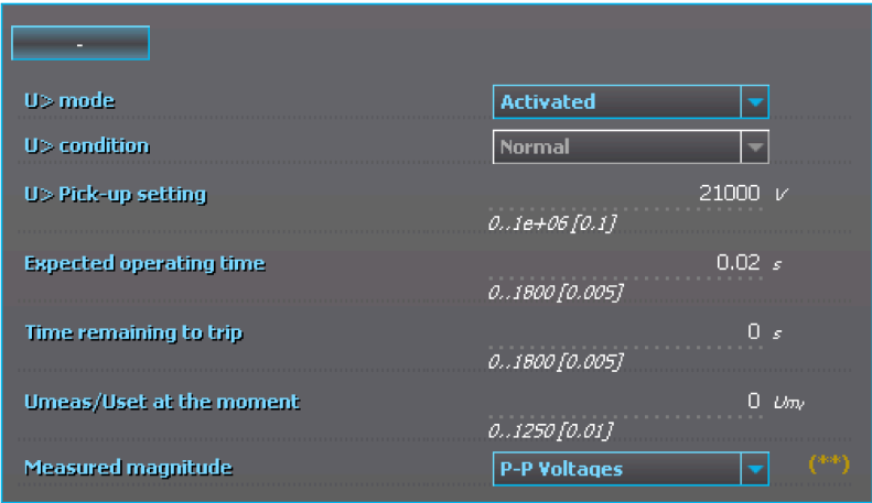
Figure. 4.2.2 - 70. Selecting the measured magnitude.
