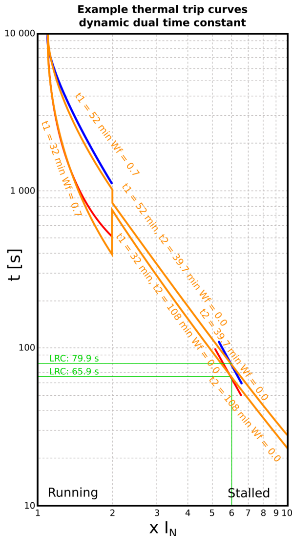
Figure. 4.4.17 - 158. Comparing dual time constant thermal replica tripping curves to given motor thermal characteristics.
