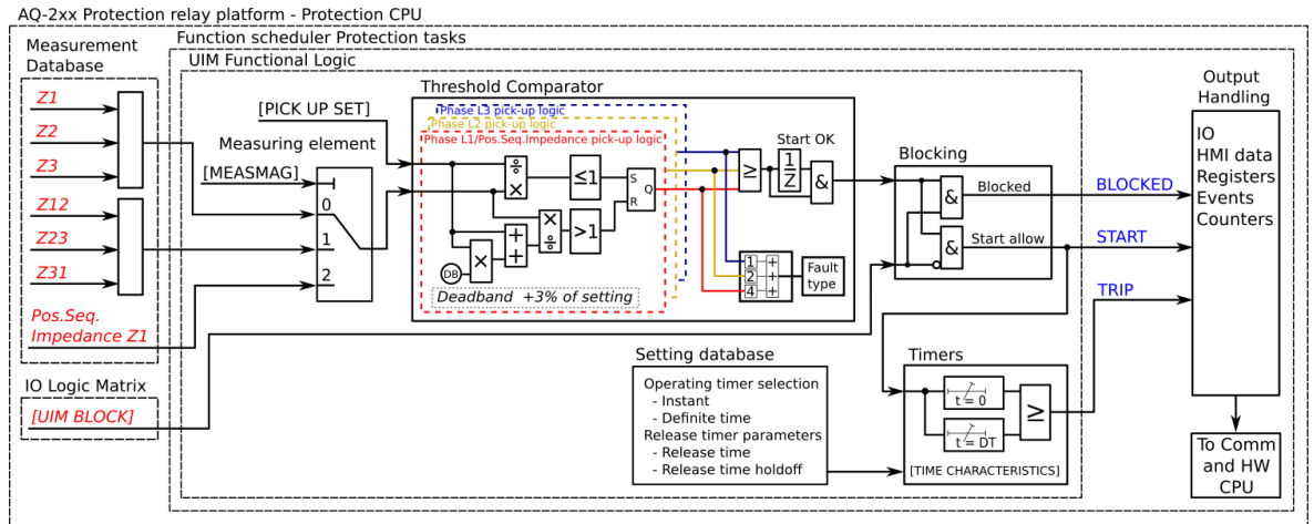
Figure. 4.4.22 - 182. Simplified function block diagram of the Z< function.
