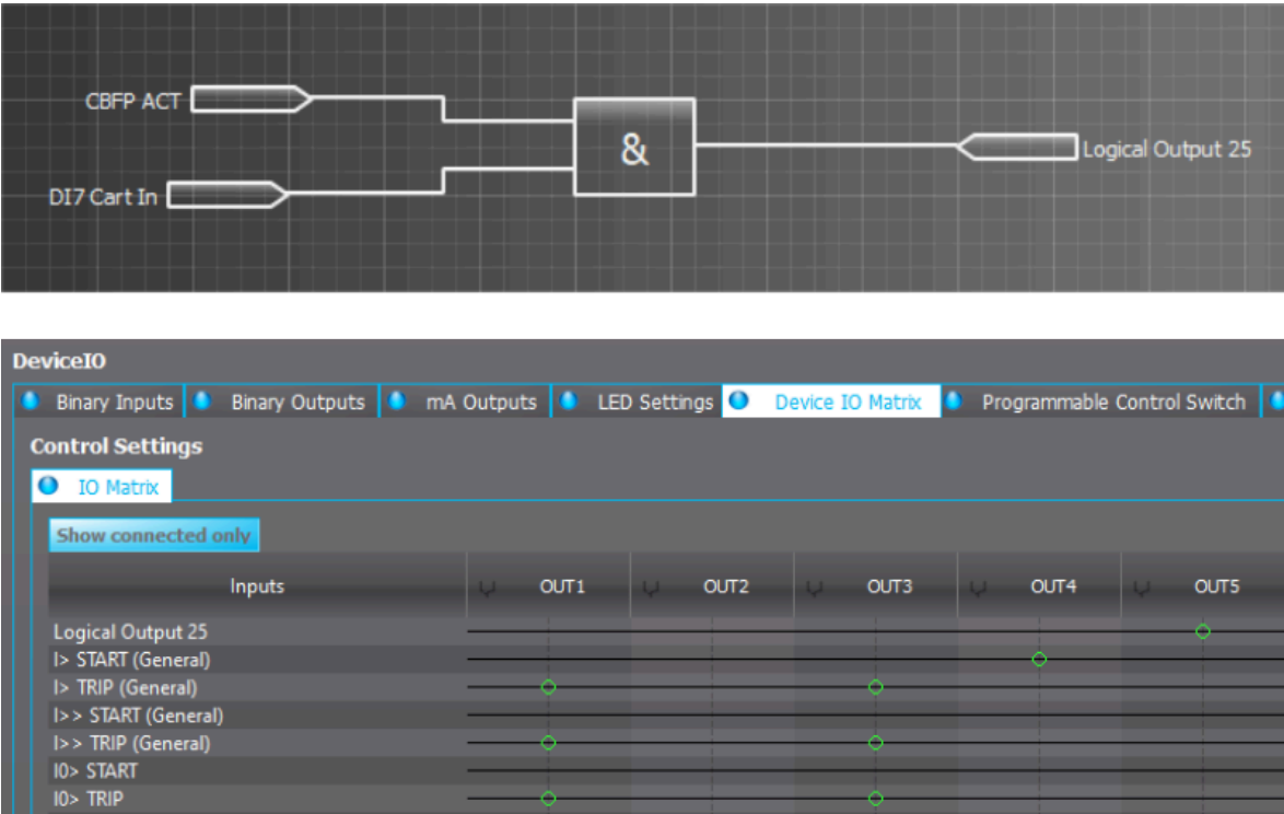
Figure. 4.5.10 - 208. Logic output example. Logical output is connected to an output relay in matrix.
