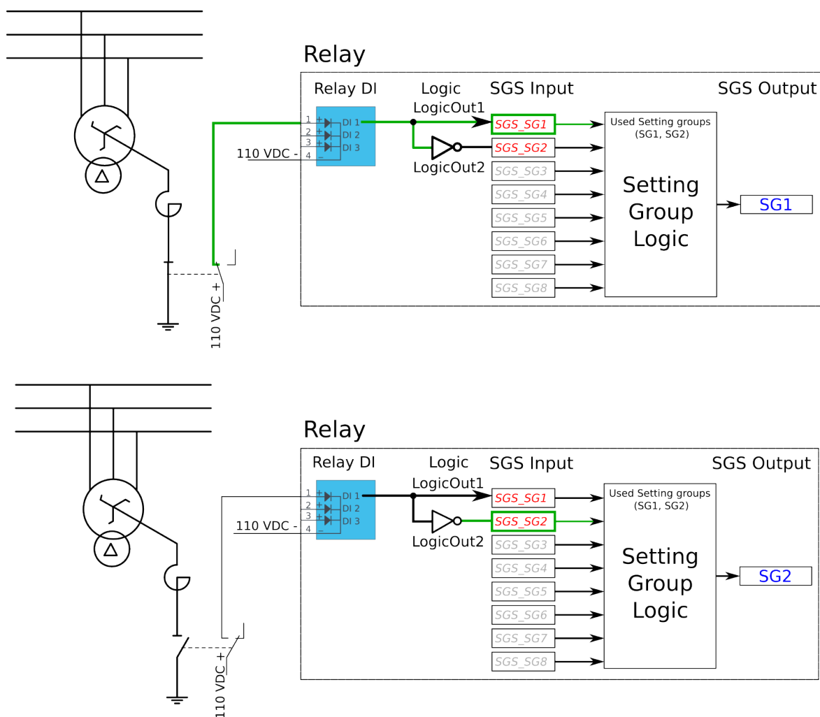
Figure. 4.5.2 - 188. Setting group control – one-wire connection from Petersen coil status.
