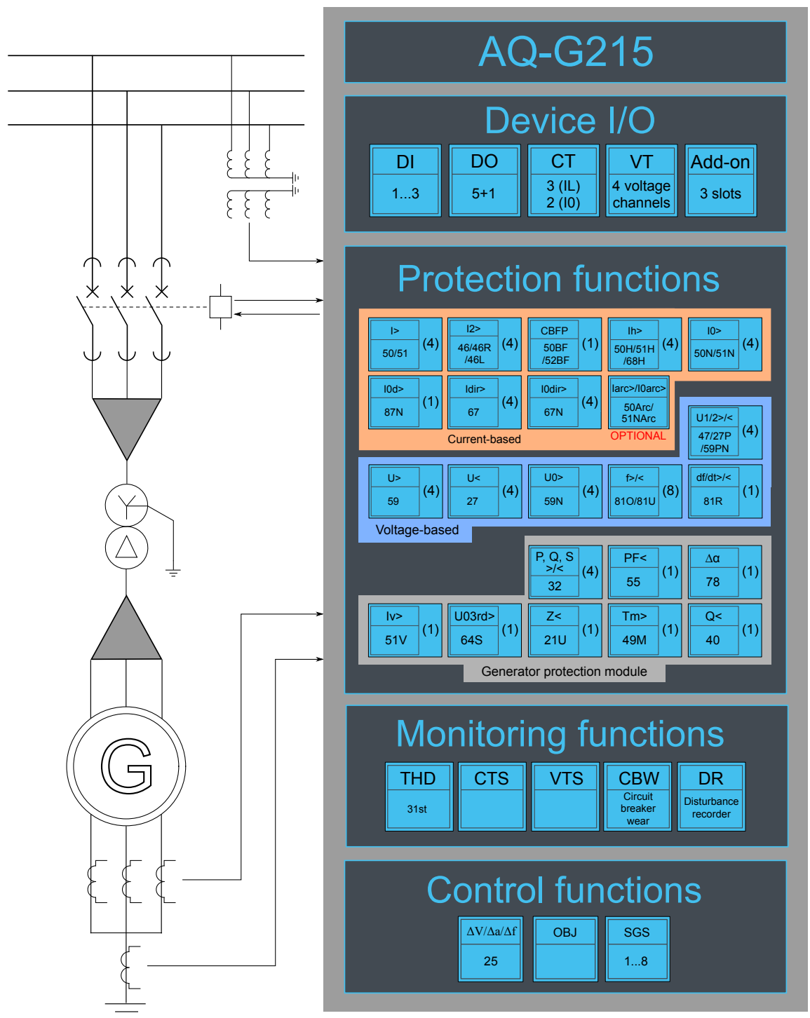
Figure. 6.1 - 234. AQ-G215 application example with function block diagram.
