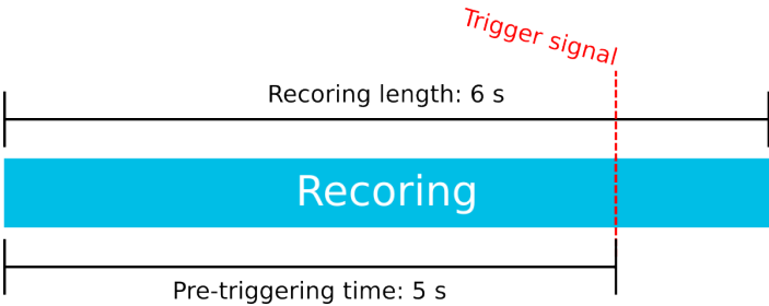
Figure. 4.6.5 - 229. Effects of recording length and pre-triggering time signals. This example is based on the settings shown above.
