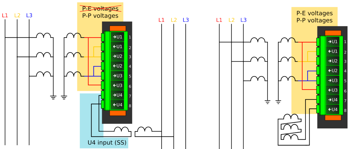
Figure. 4.4.10 - 123. Selectable measurement magnitudes with 3LL+U4 VT connection (P-E voltages not available without residual voltage).
