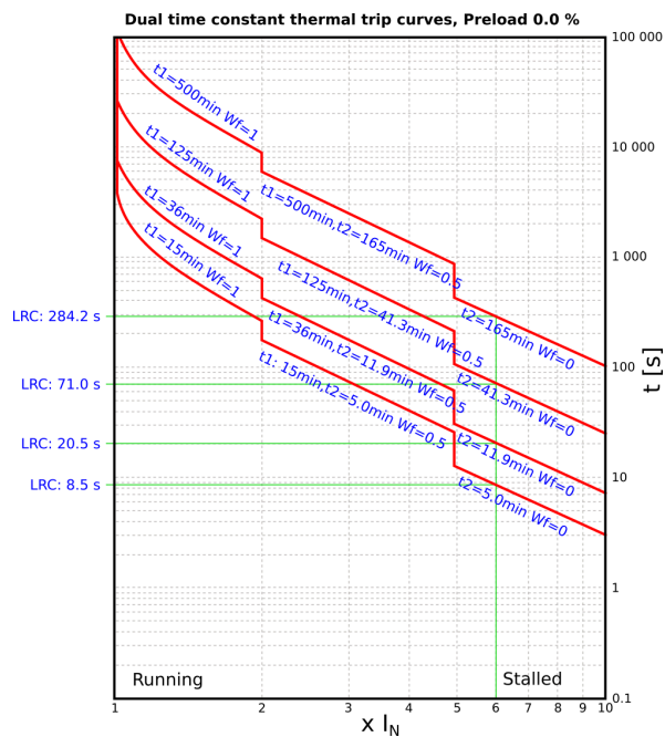
Figure. 4.4.17 - 161. Thermal tripping curves with dual dynamic time constants and correction factor, pre-load 0% (cold)
