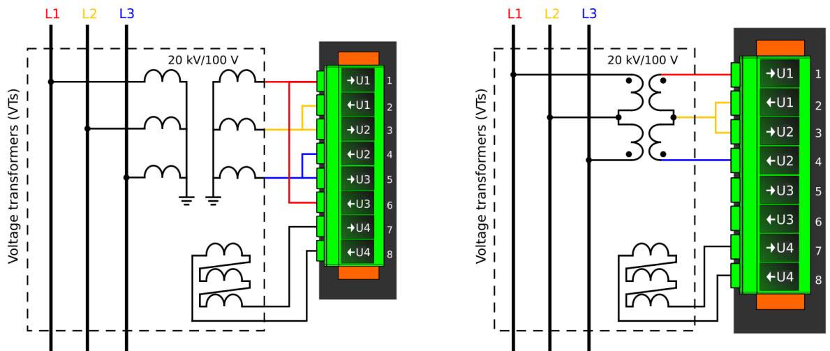
Figure. 4.2.2 - 72. Example connections for voltage line-to-line measurement.
