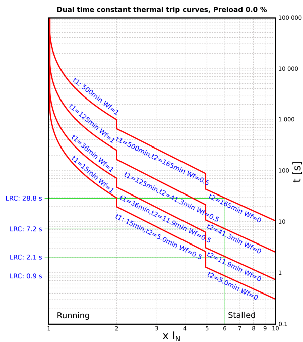
Figure. 4.4.17 - 162. Thermal tripping curves with dual dynamic time constants and correction factor, pre-load 90% (hot).
