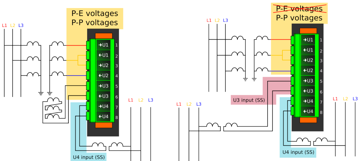
Figure. 4.4.10 - 124. Selectable measurement magnitudes with 2LL+U4 VT connection (P-E voltages not available without residual voltage).
