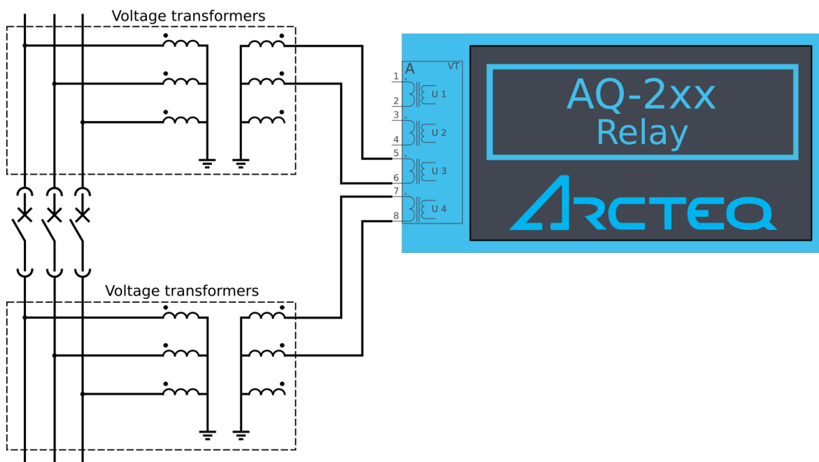
Figure. 4.5.5 - 196. Example connection of the synchrocheck function (2LL+U3+U4 mode, SYN3 in use, UL12 as reference voltage).
