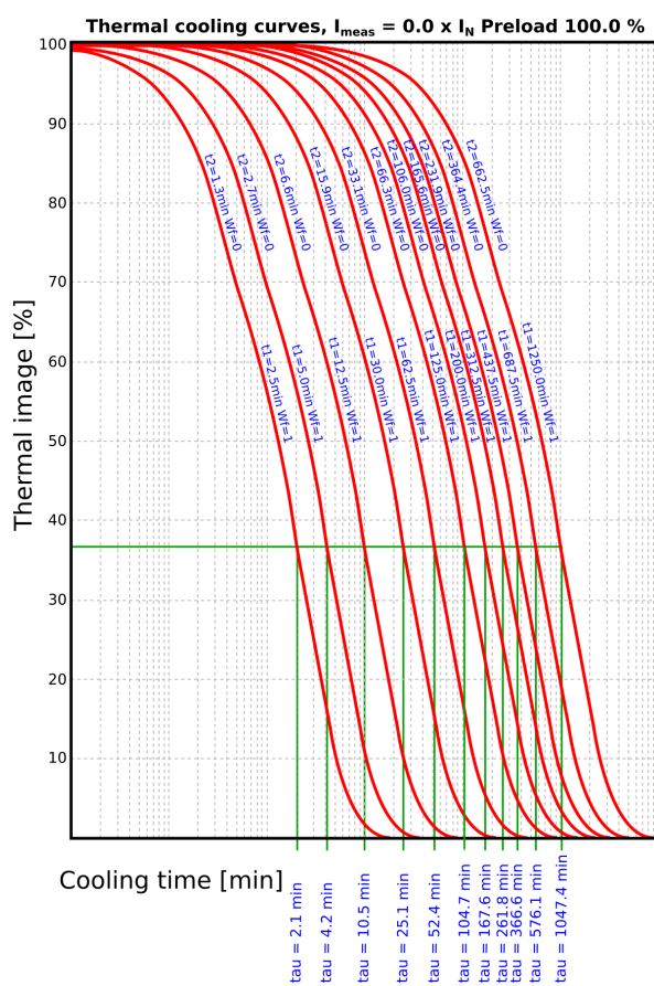
Figure. 4.4.17 - 164. Thermal cooling curves, dynamic dual time constant.
