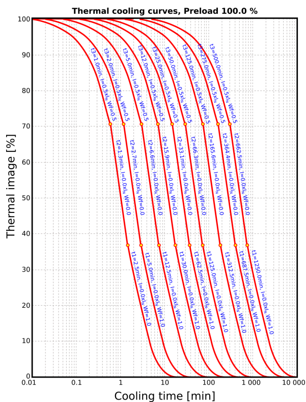
Figure. 4.4.17 - 165. Thermal cooling curves, dynamic triple time constant (motor is running without load in the first part with dedicated time constant).
