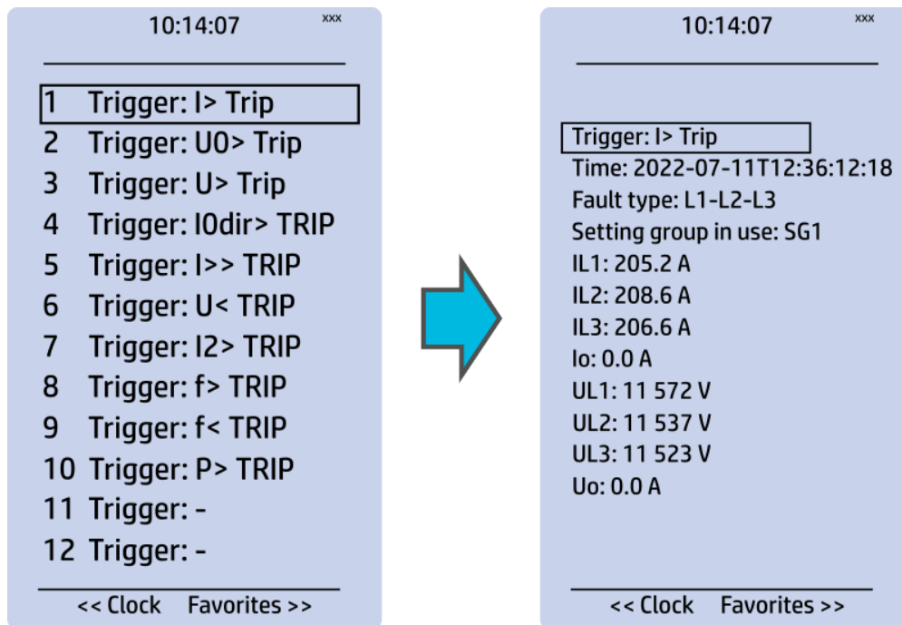
Figure. 4.6.8 - 231. 12 latest recordings can be accessed from HMI if "Fault registers" view has been enabled in "Carousel designer" tool.
