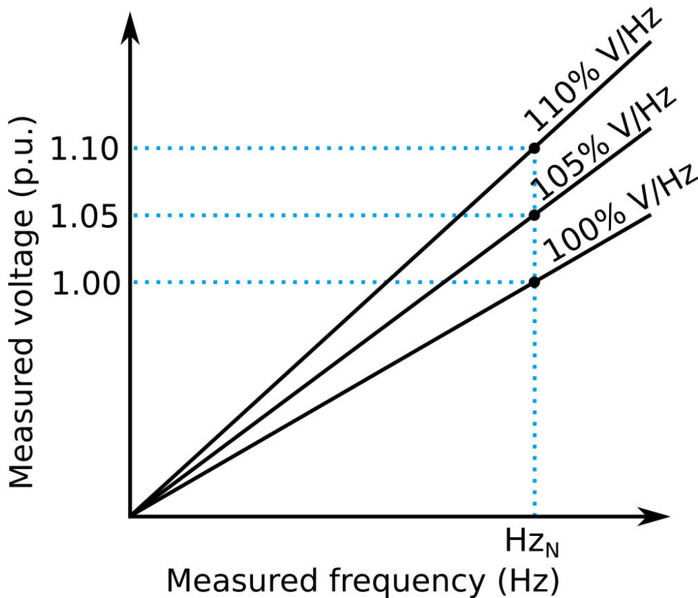
Figure. 4.4.21 - 177. Effect of pick-up settings and the measured frequency to the overvoltage function's pick-up level.
