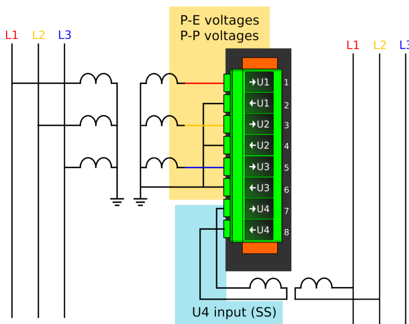
Figure. 4.4.9 - 118. Selectable measurement magnitudes with 3LN+U4 VT connection.
