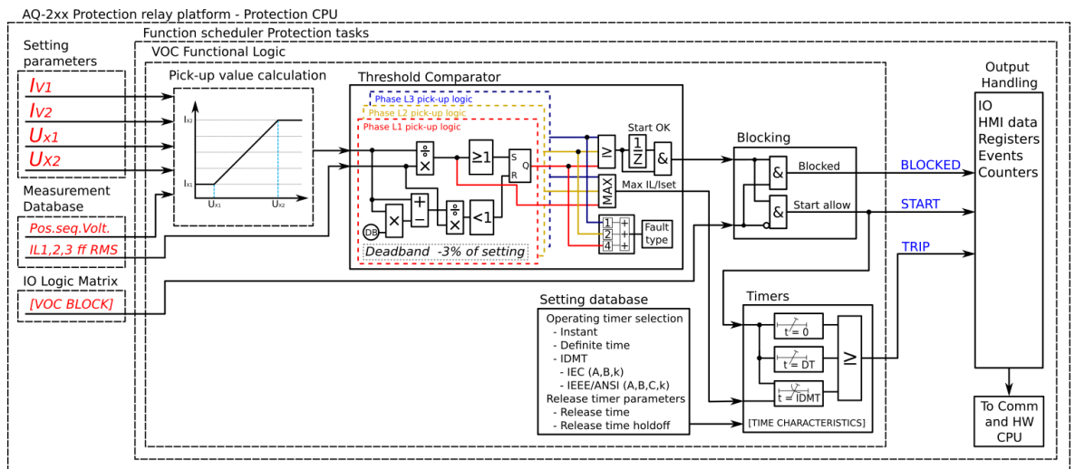
Figure. 4.4.20 - 176. Simplified function block diagram of the I_{v>} function.
