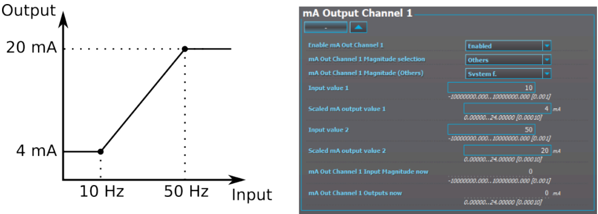
Figure. 4.5.6 - 204. Example of the effects of mA output channel settings.
