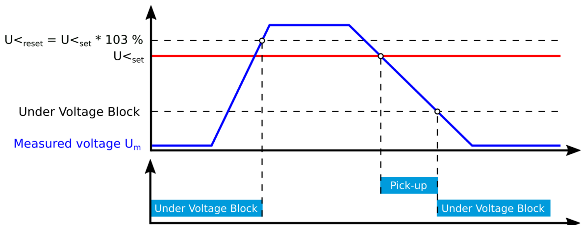
Figure. 4.4.10 - 125. Example of the block setting operation.
