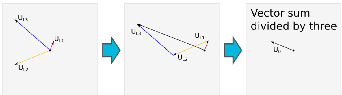
Figure. 4.4.11 - 127. Earth fault in isolated network.
