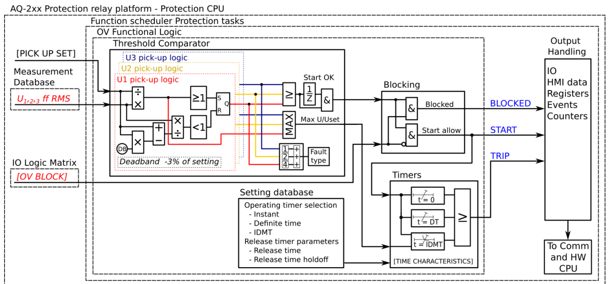
Figure. 4.4.9 - 117. Simplified function block diagram of the U> function.
