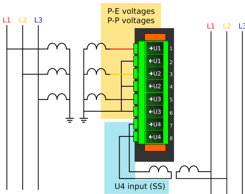
Figure. 4.4.10 - 122. Selectable measurement magnitudes with 3LN+U4 VT connection.
