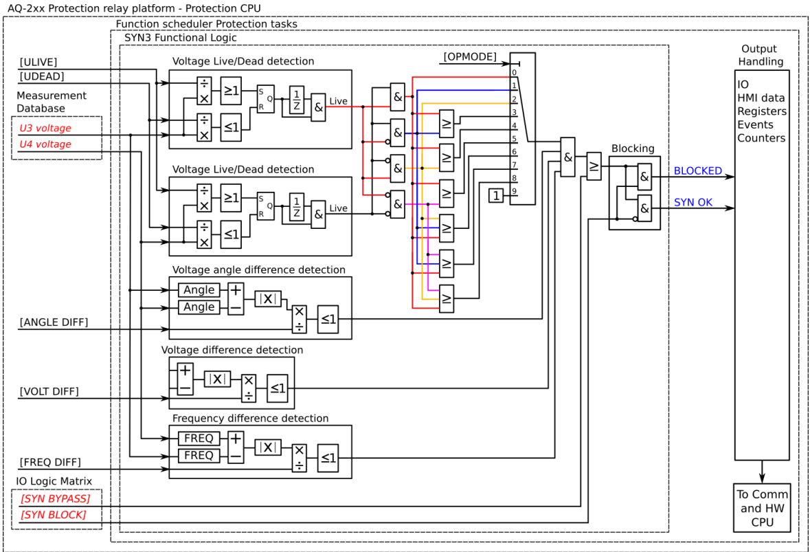
Figure. 4.5.5 - 203. Simplified function block diagram of the SYN3 function.
