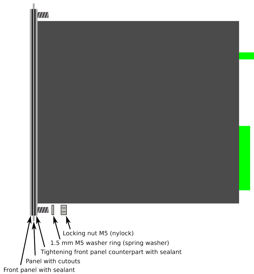
Figure. 7.6 - 262. Device installation.
