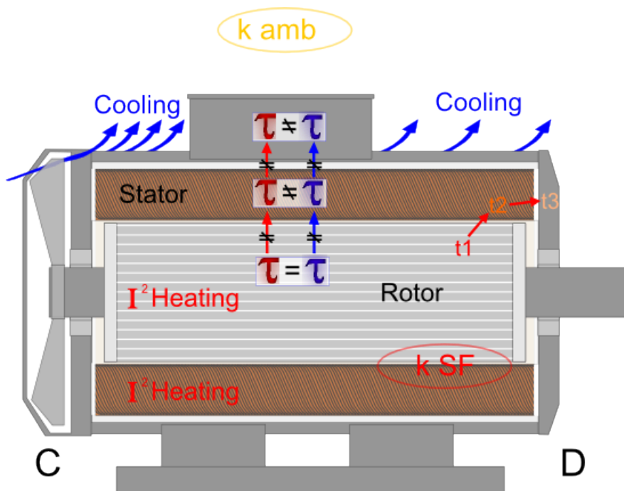
Figure. 4.4.17 - 152. Simplified motor construction and time constants.
