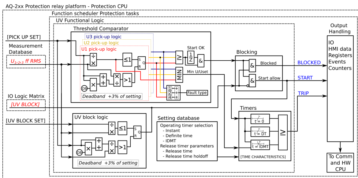
Figure. 4.4.10 - 121. Simplified function block diagram of the U< function.
