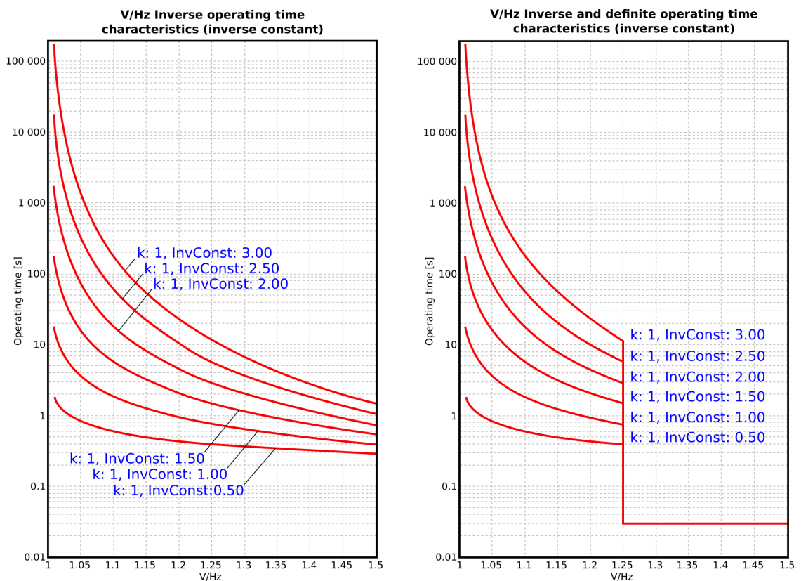
Figure. 4.4.21 - 180. Inverse (above) and inverse and DT (below) time characteristics with the inverse constant setting effect.
