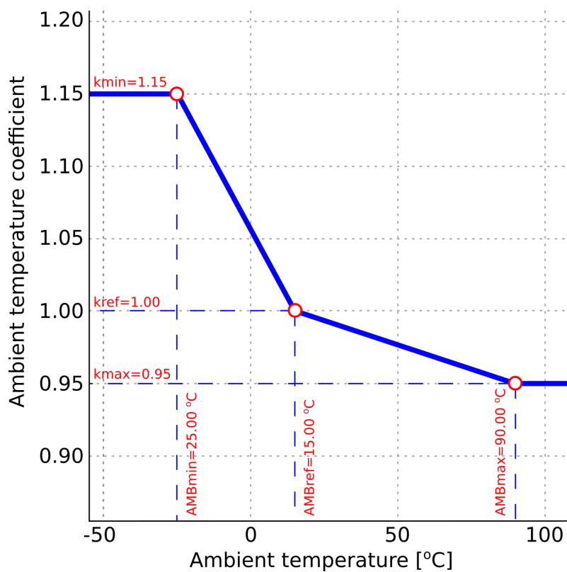
Figure. 4.4.17 - 149. Ambient temperature coefficient calculation (linear approximation, three points).
