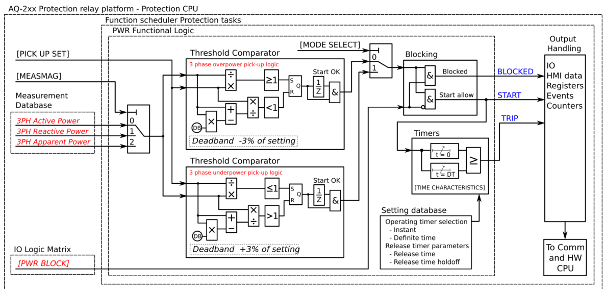
Figure. 4.4.15 - 143. Simplified function block diagram of the power protection function.
