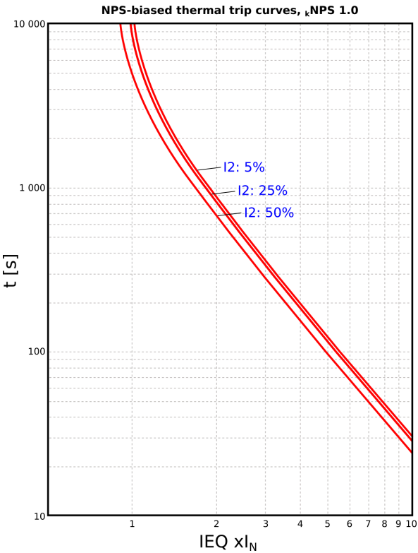
Figure. 4.4.17 - 166. NPS-biased thermal trip curves with k_{NPS} value of 1.
