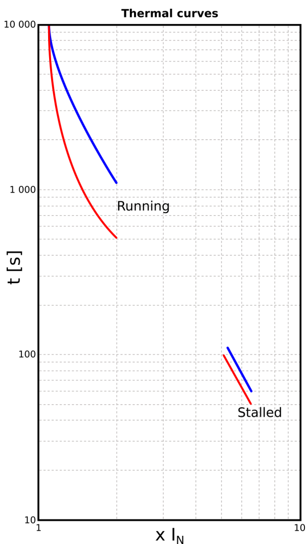
Figure. 4.4.17 - 156. Example of thermal limit curves in a motor.
