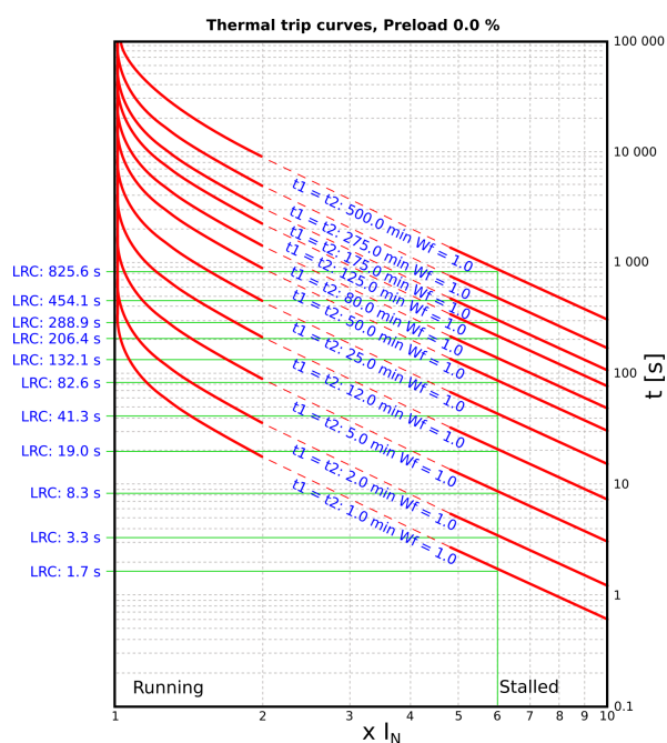
Figure. 4.4.17 - 159. Thermal tripping curves with single time constant, pre-load 0% (cold).
