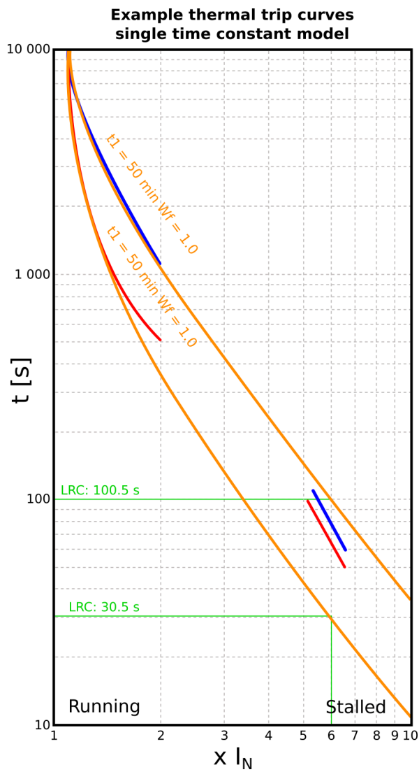
Figure. 4.4.17 - 157. Comparing single time constant thermal replica tripping curves to given motor thermal characteristics.
