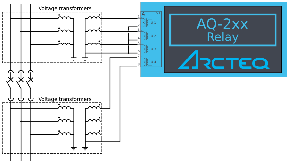
Figure. 4.5.5 - 194. Example connection of the synchrocheck function (3LN+U4 mode, SYN1 in use, UL1 as reference voltage).
