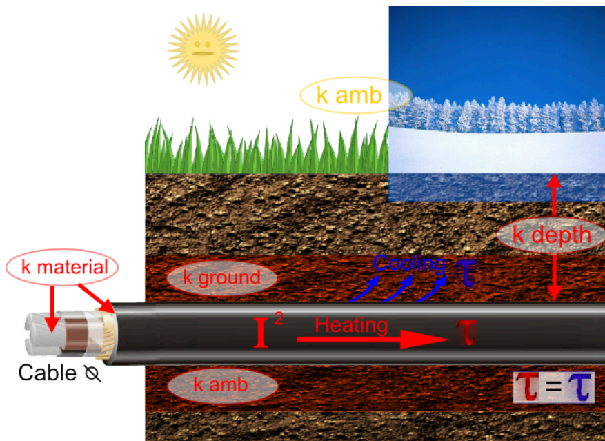
Figure. 4.4.17 - 151. Factors affecting the cooling and current-carrying capacity of a cable.
