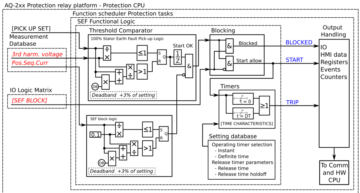
Figure. 4.4.19 - 174. Simplified function block diagram of the U03rd> function.
