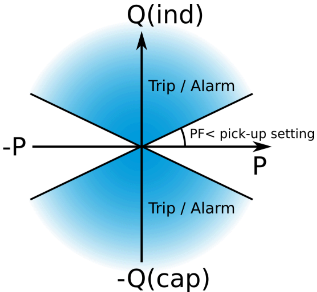
Figure. 4.4.16 - 144. Operating characteristics of power factor protection.
