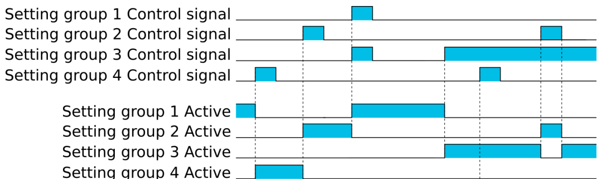
Figure. 4.5.2 - 187. Example sequences of group changing (control with pulse only, or with both pulses and static signals).
