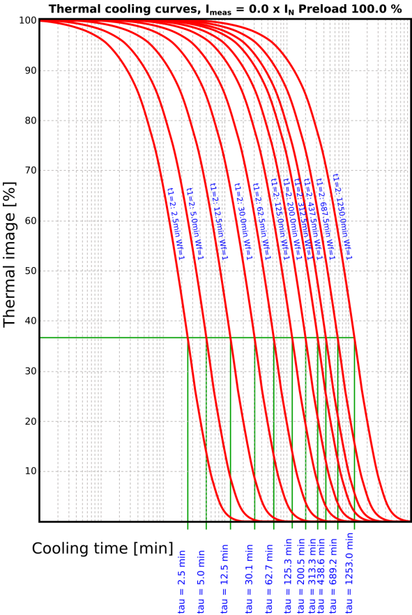
Figure. 4.4.17 - 163. Thermal cooling curves, single cooling time constant.
