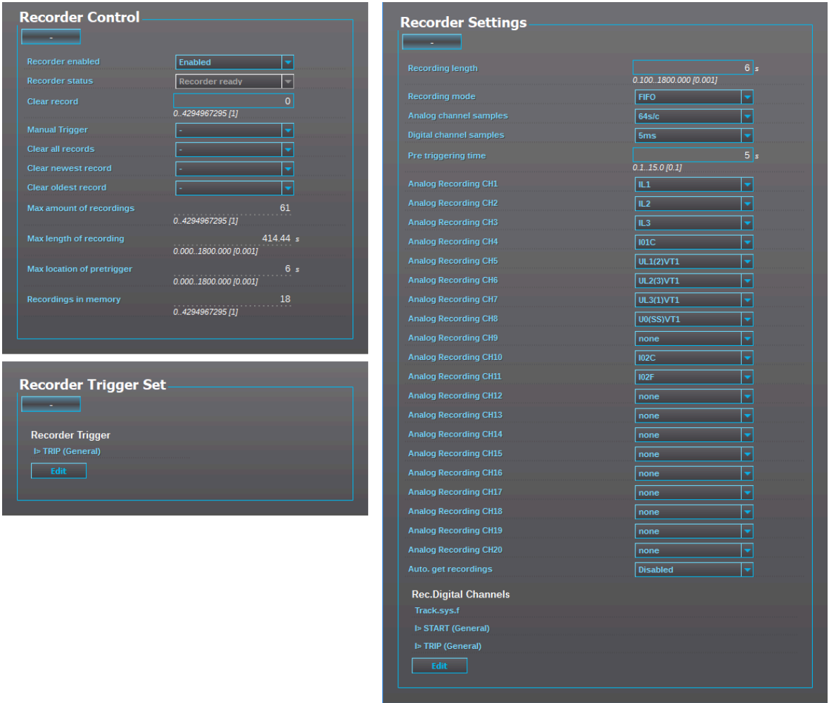
Figure. 4.6.5 - 228. Disturbance recorder settings.
