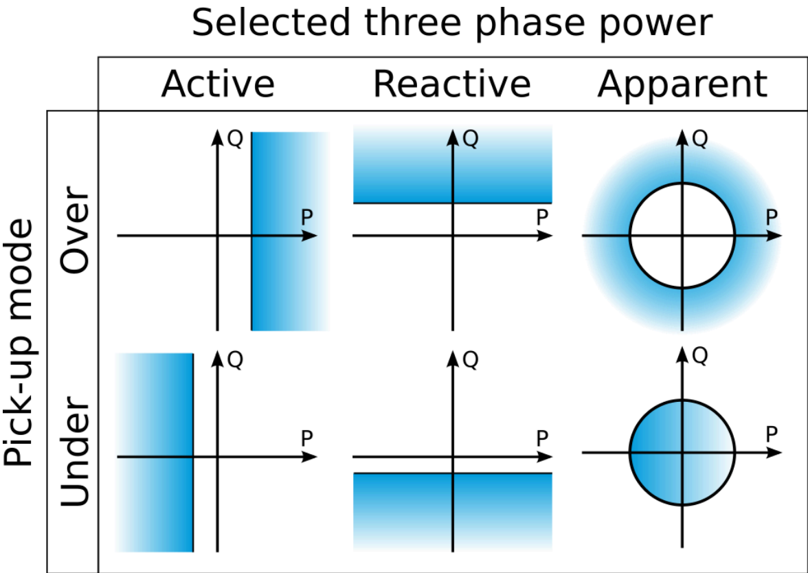
Figure. 4.4.15 - 142. PQ diagram of the pick-up areas in various modes.
