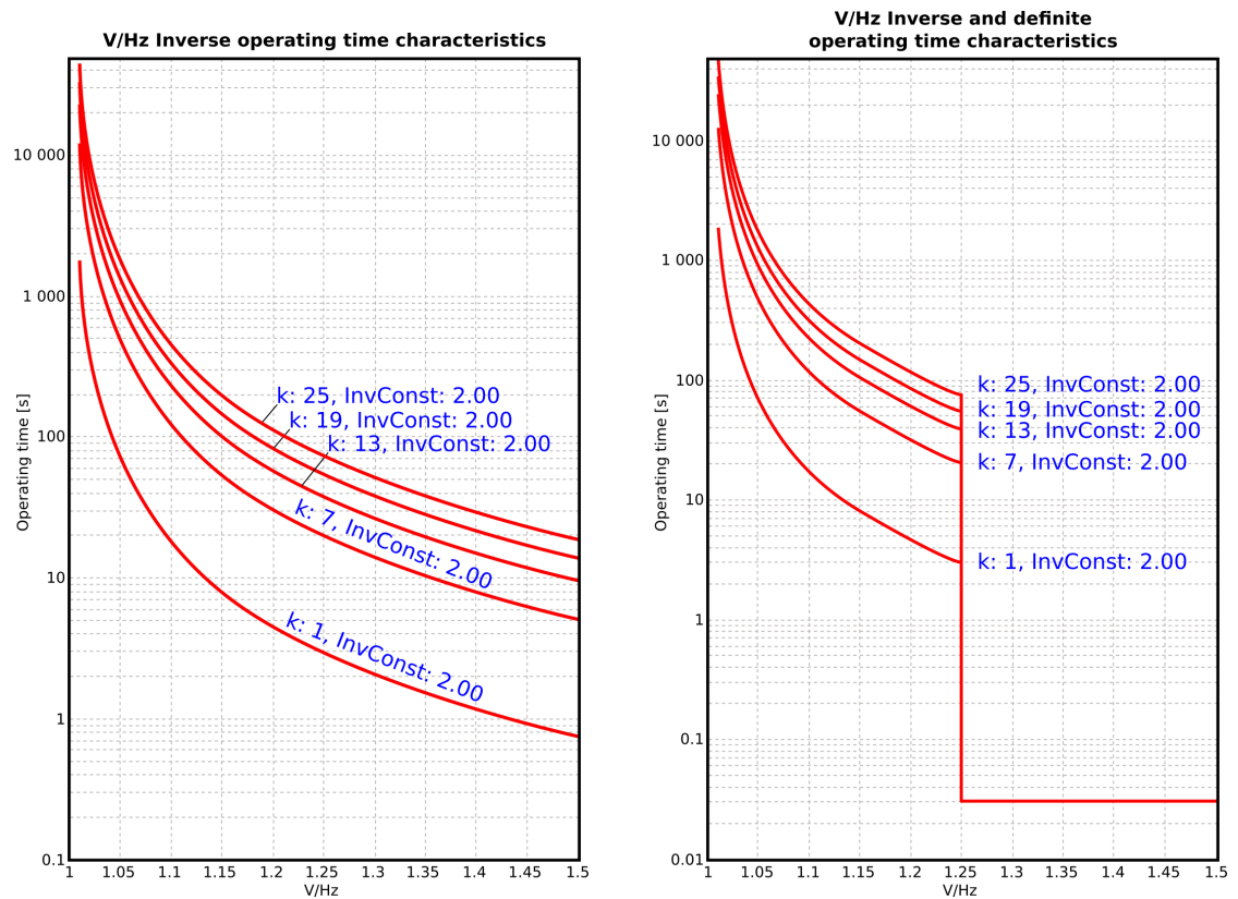
Figure. 4.4.21 - 179. Inverse (above) and inverse and DT (below) time characteristics with the TimeDial k setting effect.
