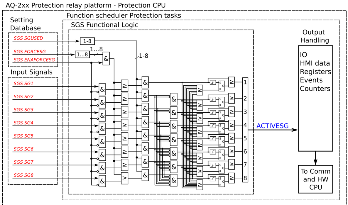
Figure. 4.5.2 - 186. Simplified function block diagram of the setting group selection function.
