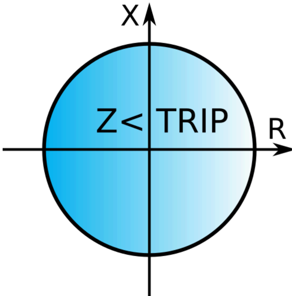
Figure. 4.4.22 - 181. Operating characteristics of underimpedance protection.
