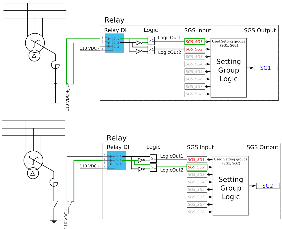
Figure. 4.5.2 - 190. Setting group control – two-wire connection from Petersen coil status with additional logic.
