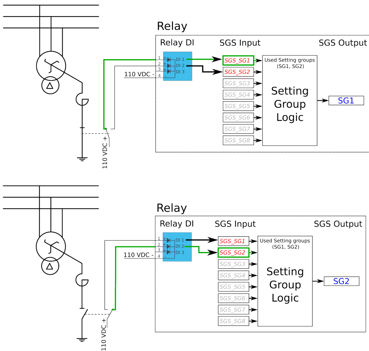
Figure. 4.5.2 - 189. Setting group control – two-wire connection from Petersen coil status.
