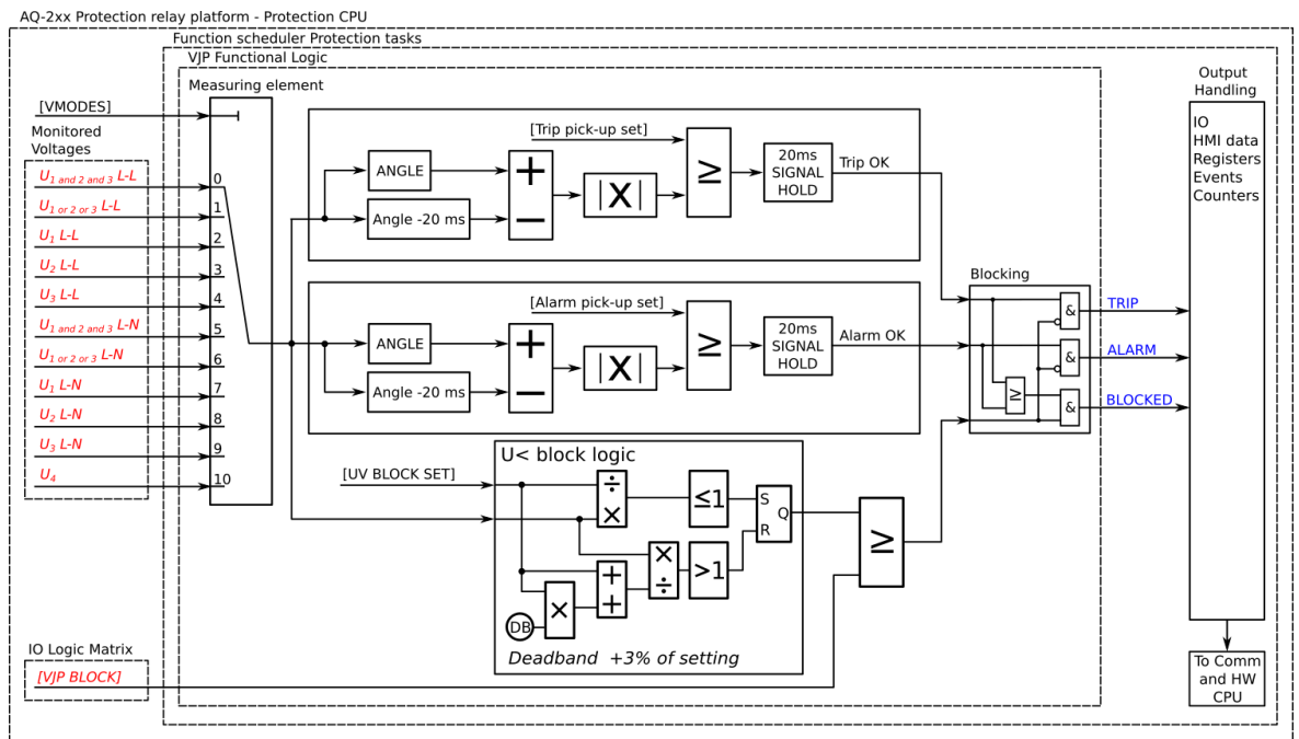
Figure. 4.5.7 - 205. Simplified function block diagram of the \Delta\phi function.
