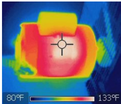
Figure. 4.4.17 - 153. Running motor's temperature with thermal image camera.
