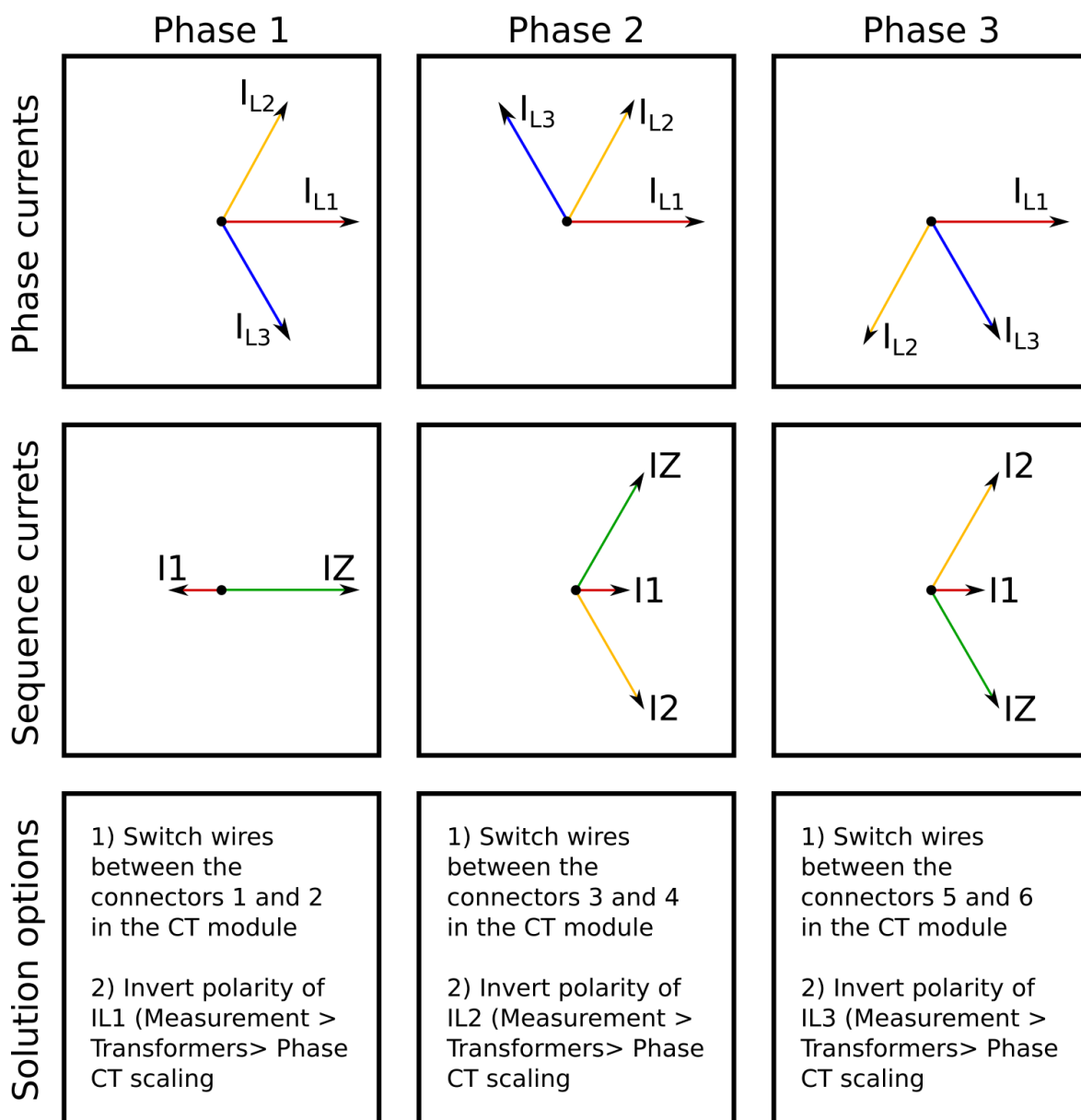
Figure. 4.2.1 - 66. Common phase polarity problems.
