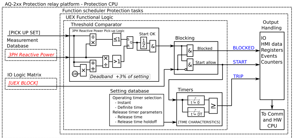
Figure. 4.4.18 - 172. Simplified function block diagram of the Q< function.
