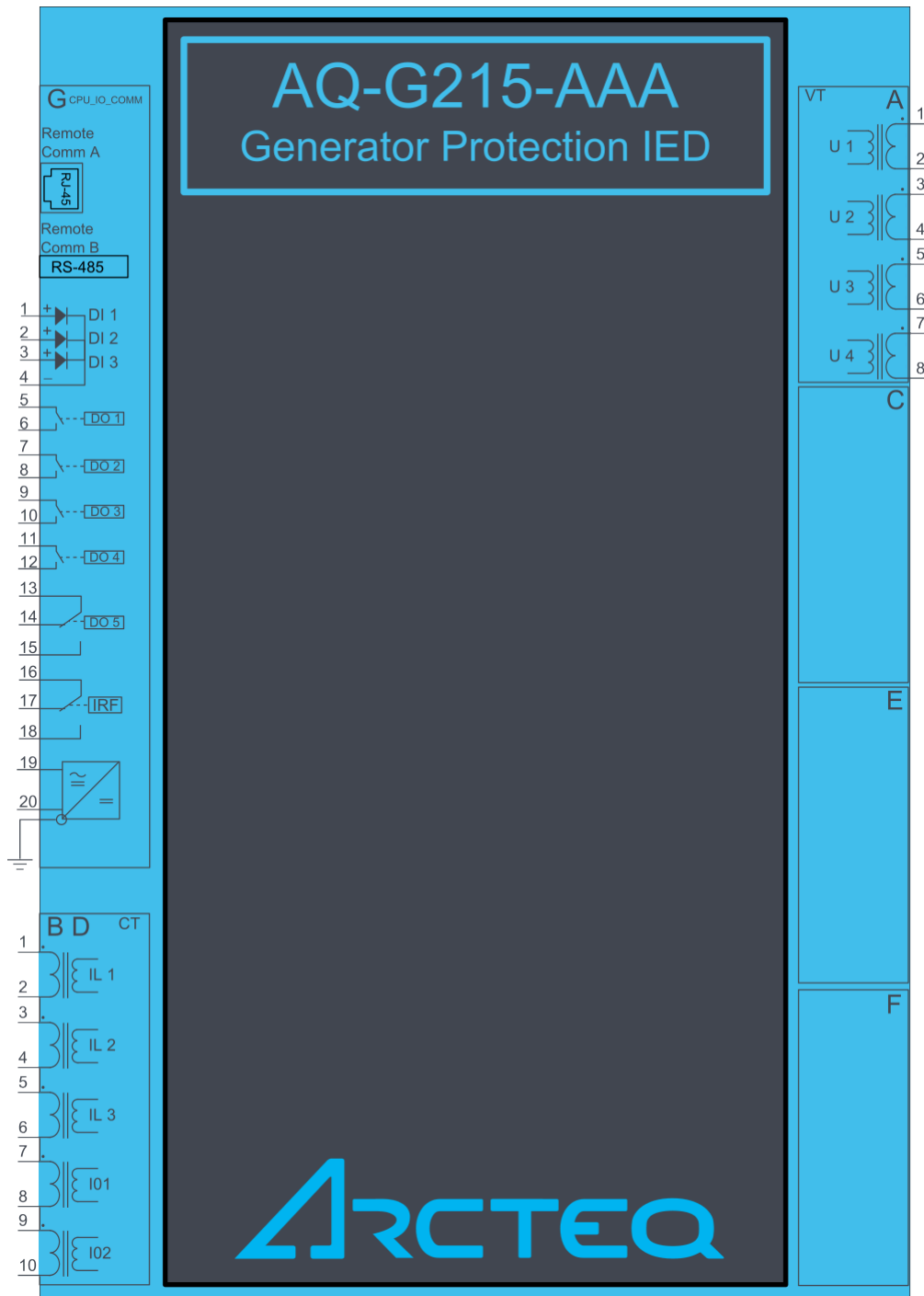
Figure. 6.1 - 232. AQ-G215 variant without add-on modules.
