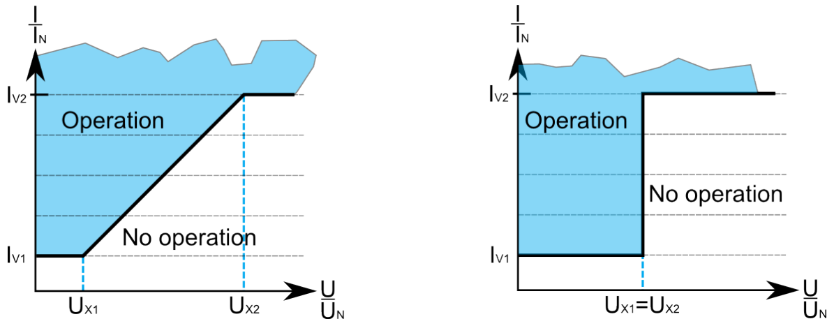
Figure. 4.4.20 - 175. Pick-up levels in the two modes.
