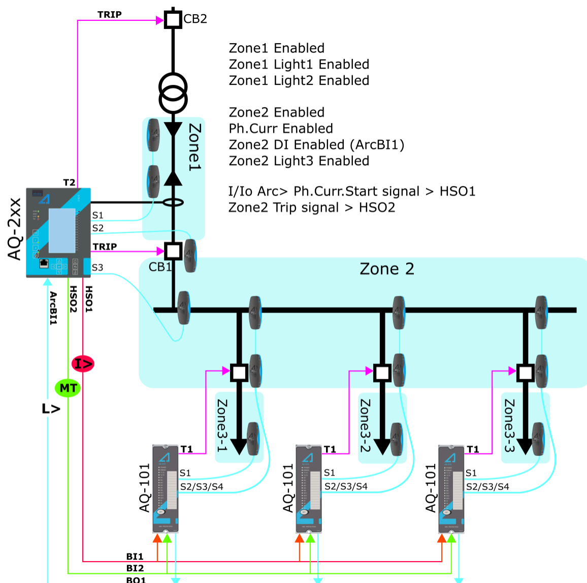
Figure. 4.4.25 - 184. Scheme IA1 (with AQ-101 arc protection relays).
