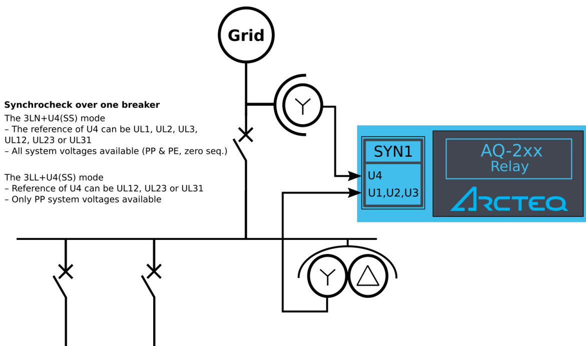
Figure. 4.5.5 - 197. Example application (synchrocheck over one breaker, with 3LL and 3LN VT connections).
