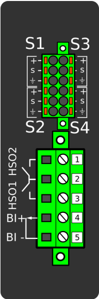
Figure. 7.5.3 - 250. Arc protection module.
