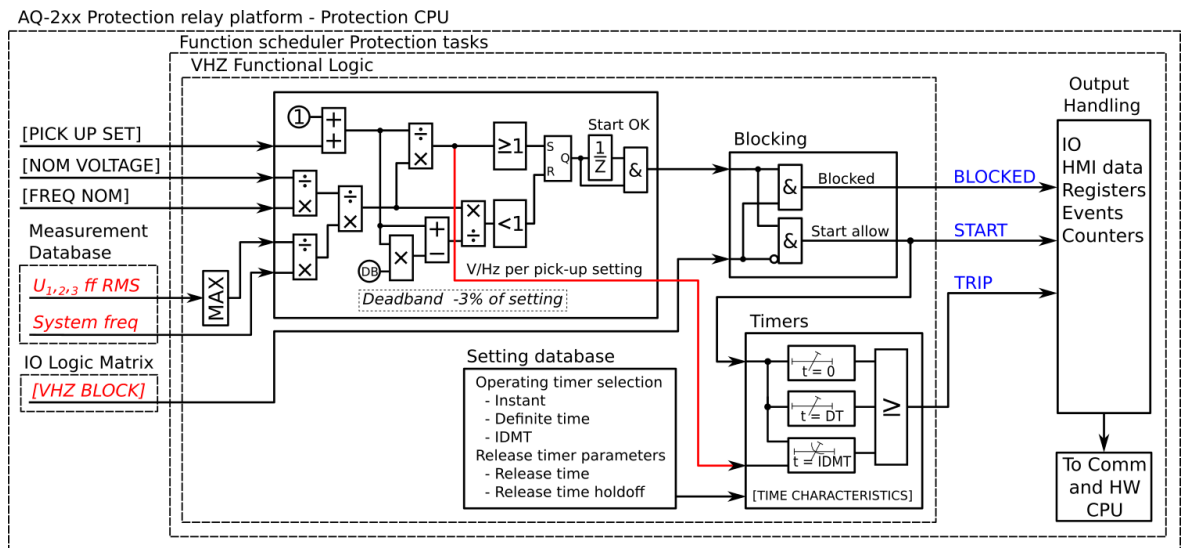
Figure. 4.4.21 - 178. Simplified function block diagram of the V/Hz> function.
