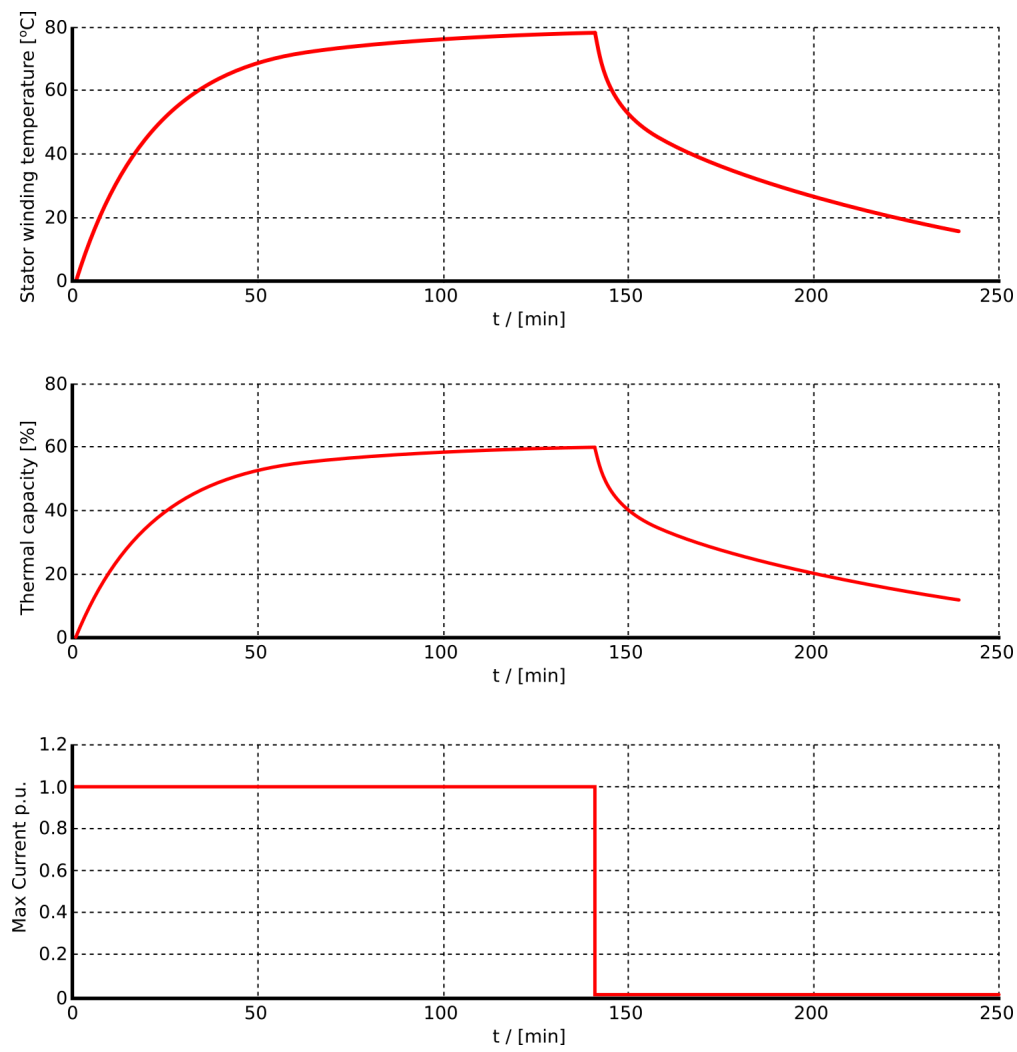
Figure. 4.4.17 - 154. Measured motor temperature in heating/cooling test.
