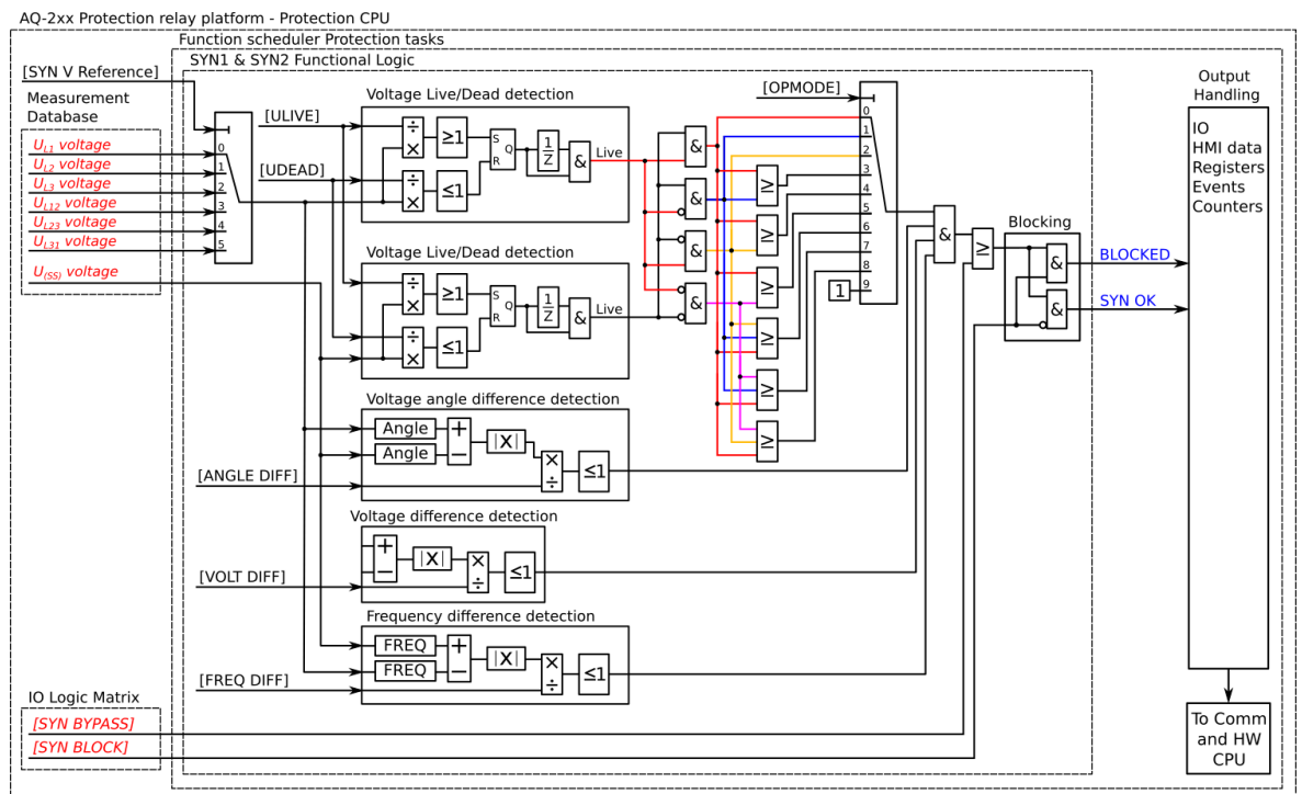
Figure. 4.5.5 - 202. Simplified function block diagram of the SYN1 and SYN2 function.
