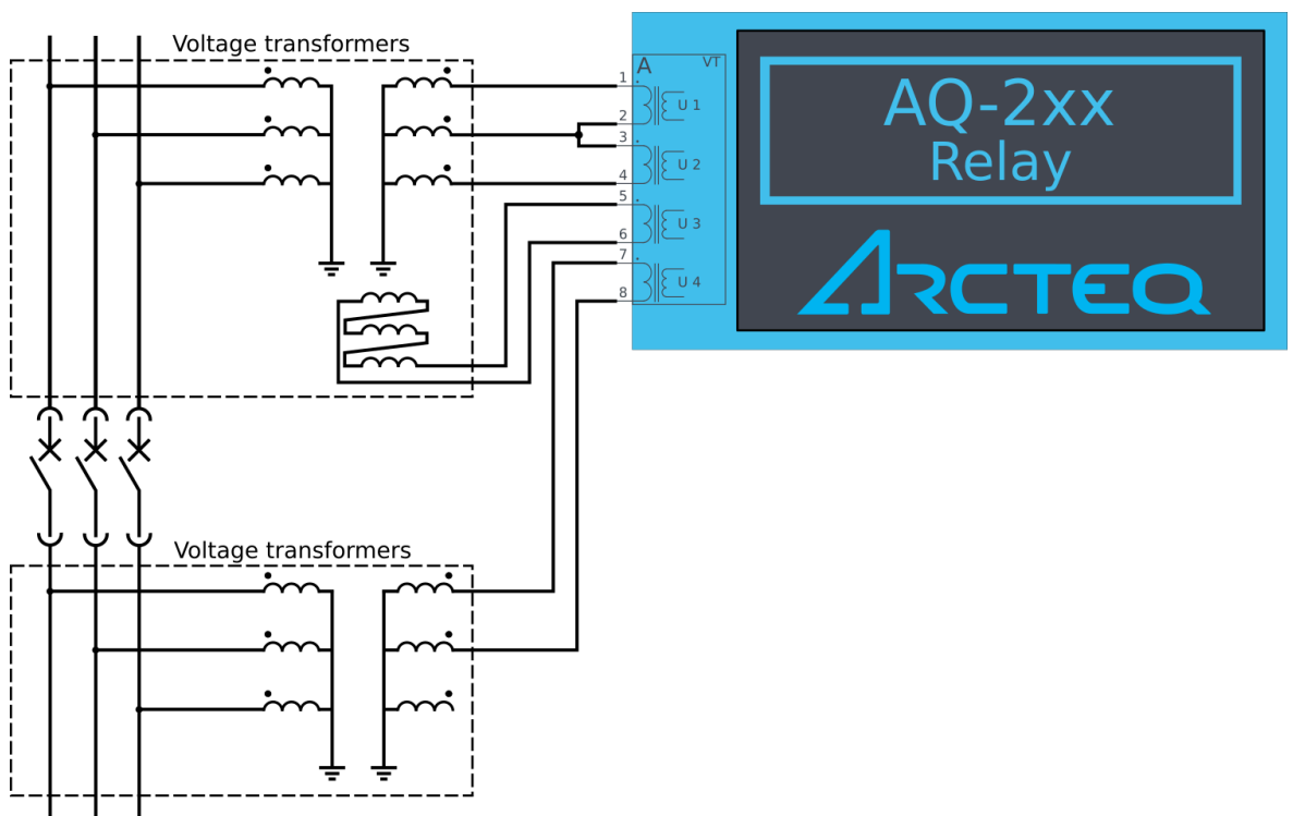
Figure. 4.5.5 - 195. Example connection of the synchrocheck function (2LL+U0+U4 mode, SYN1 in use, UL12 as reference voltage).
