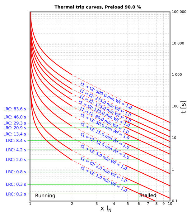
Figure. 4.4.17 - 160. Thermal tripping curves with single time constant, pre-load 90% (hot).
