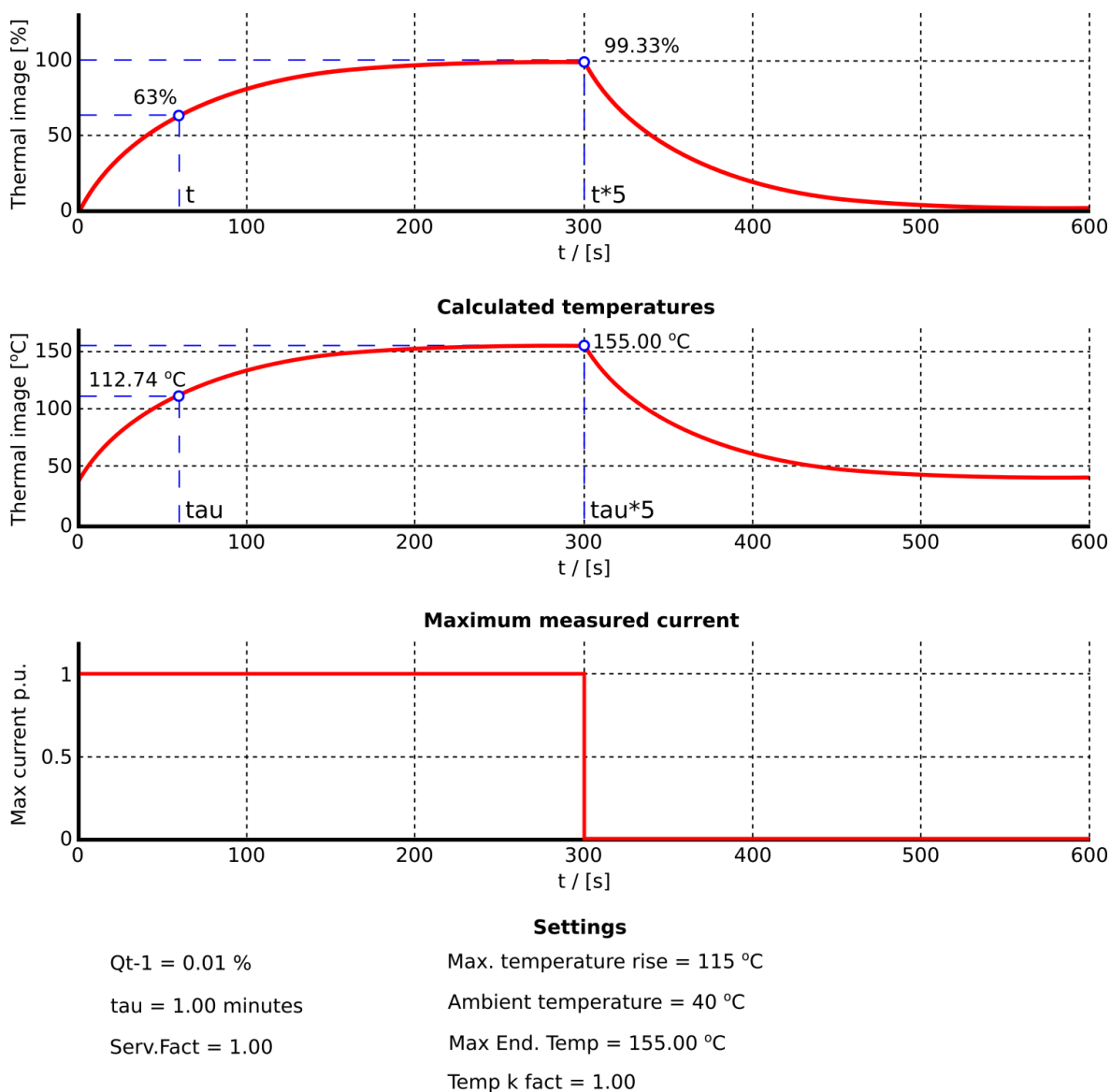
Figure. 4.4.17 - 148. Thermal image calculation with nominal conditions: single time constant thermal replica.
