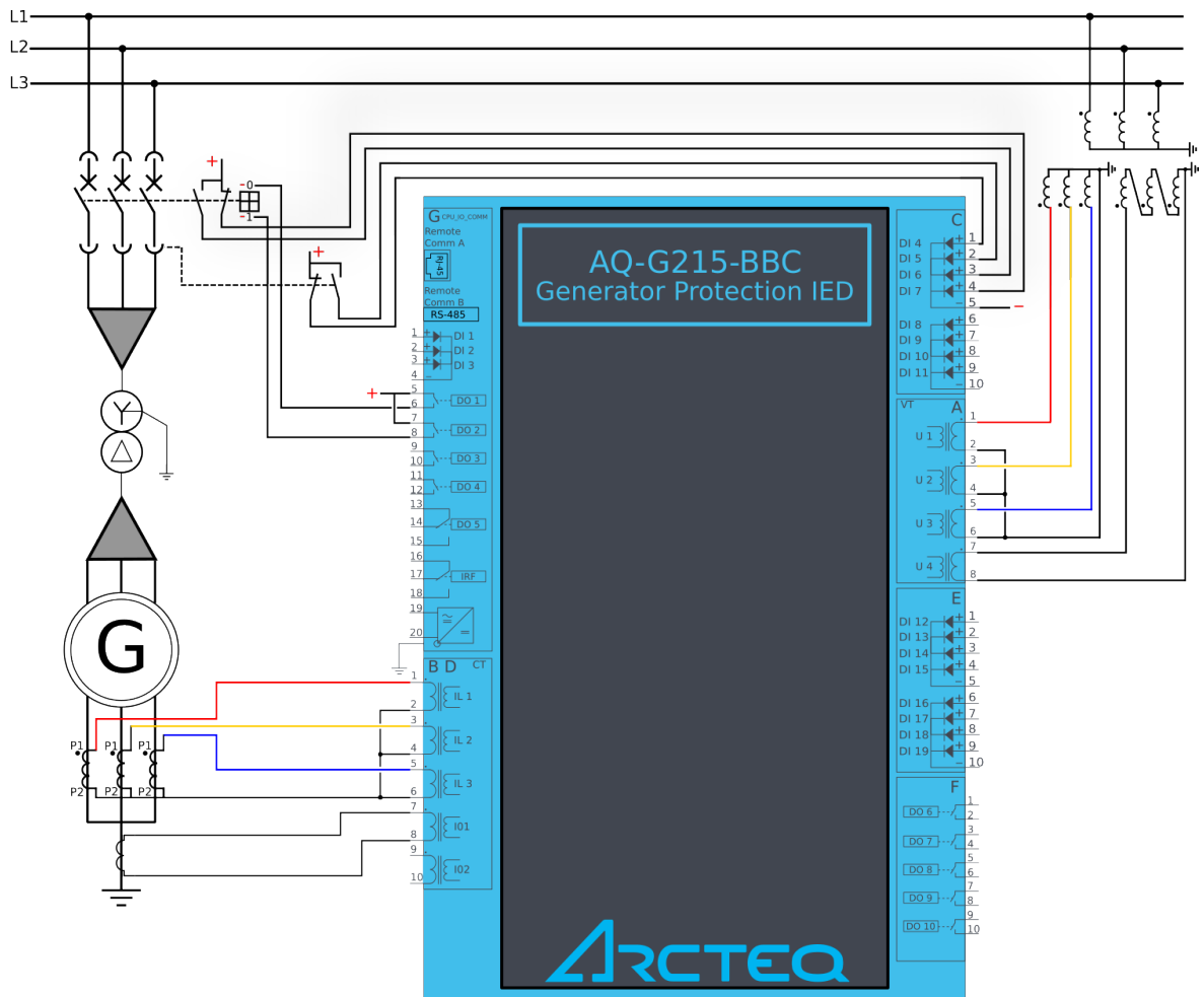
Figure. 6.2 - 235. Application example and its connections.
