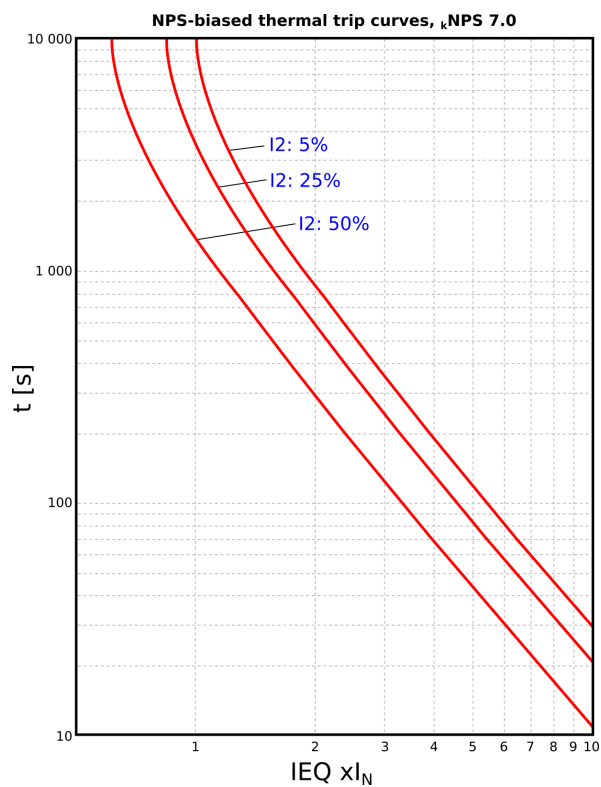
Figure. 4.4.17 - 168. NPS-biased thermal trip curves with k_{NPS} value of 7.
