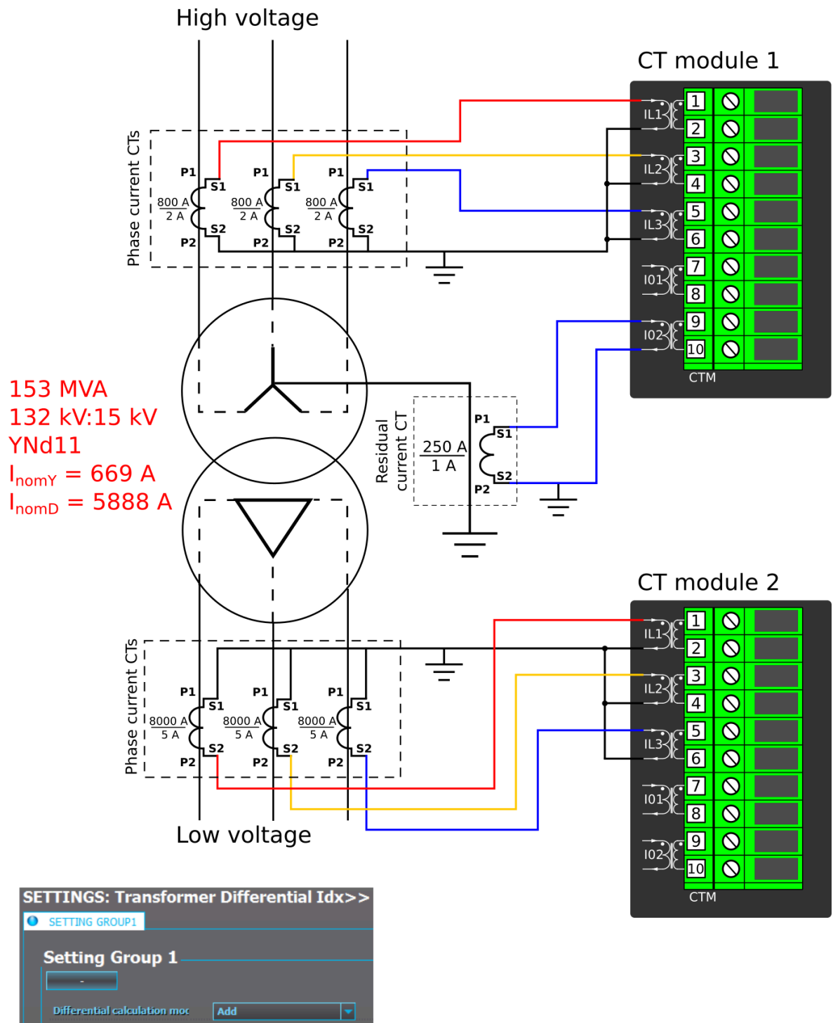
Figure. 4.2.1 - 8. Connections (application 2).
