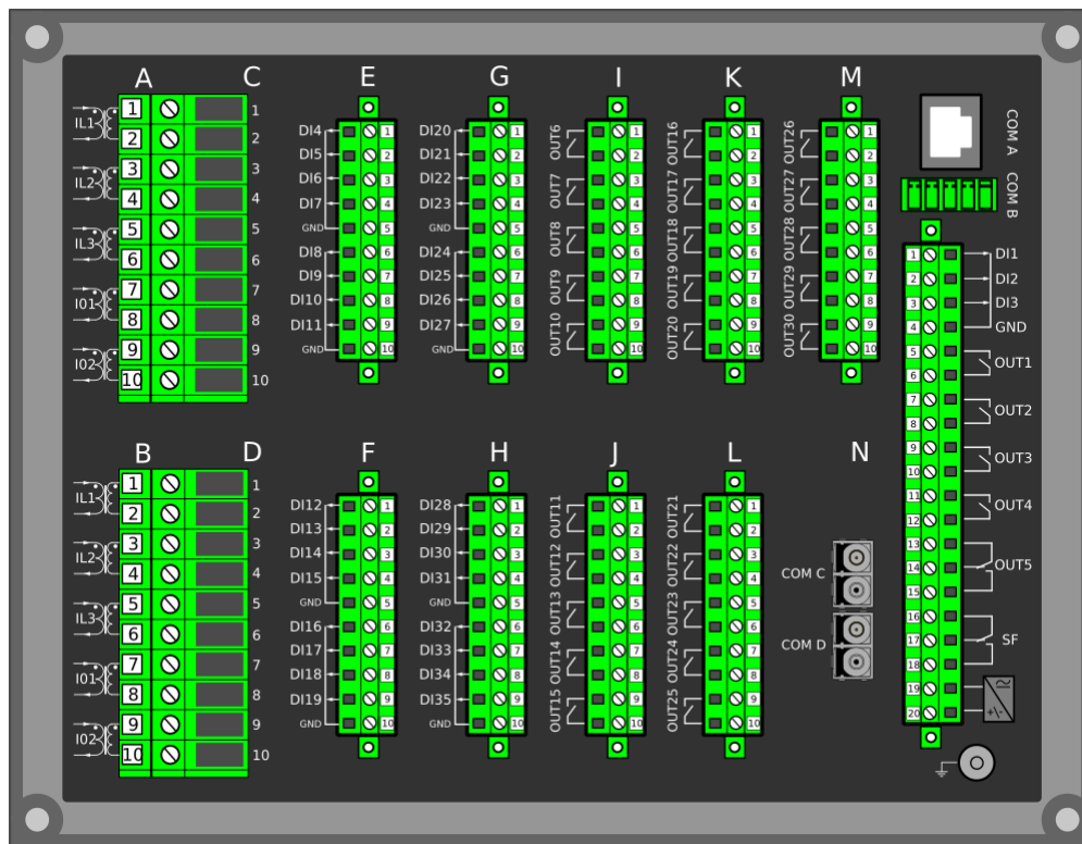
Figure. 7.1 - 117. Modular construction of AQ-X256-XXXXXXX-BBBBCCCCCJ
