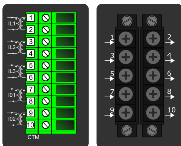
Figure. 7.3 - 120. Module connections with standard and ring lug terminals.
