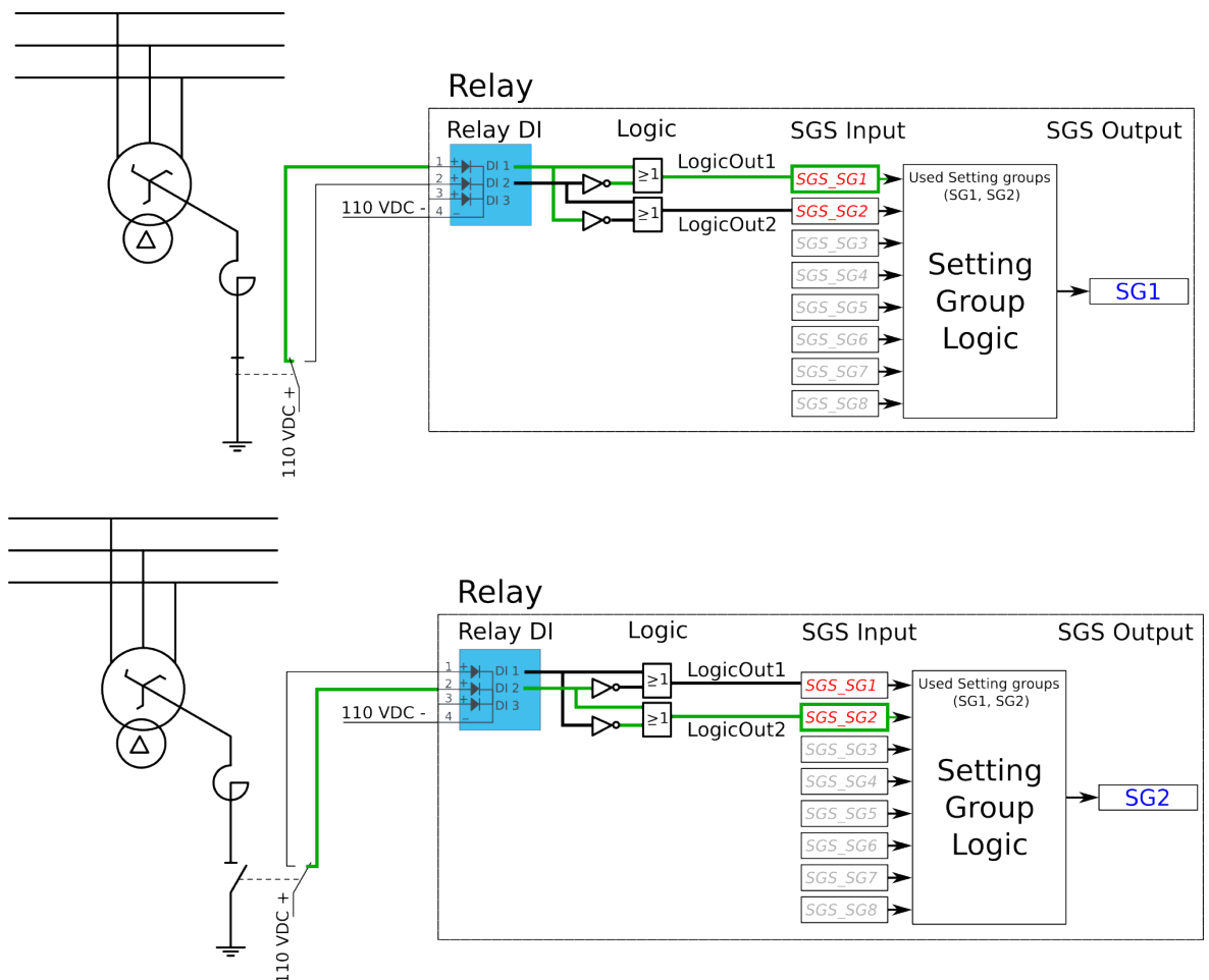
Figure. 4.5.2 - 75. Setting group control – two-wire connection from Petersen coil status with additional logic.
