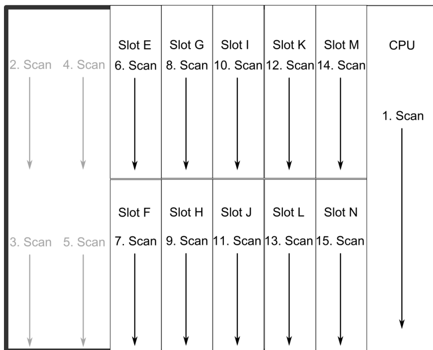
Figure. 7.1 - 118. AQ-X255 hardware scanning and I/O naming principles.
