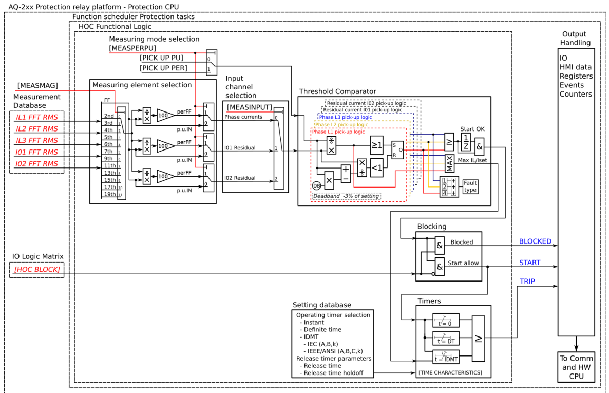
Figure. 4.4.5 - 23. Simplified function block diagram of the Ih> function.
