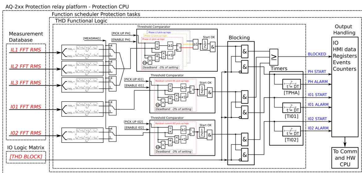
Figure. 4.6.3 - 99. Simplified function block diagram of the total harmonic distortion monitor function.
