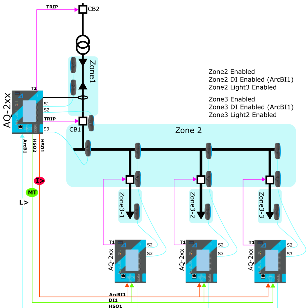
Figure. 4.4.12 - 70. Scheme IA1 (with AQ-200 protection relays).
