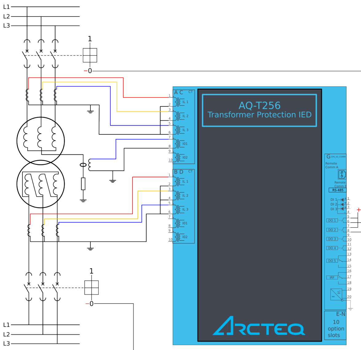
Figure. 6.2 - 110. Application example and its connections.
