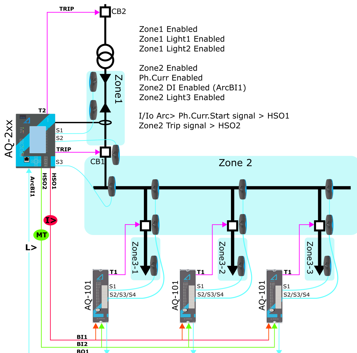
Figure. 4.4.12 - 69. Scheme IA1 (with AQ-101 arc protection relays).
