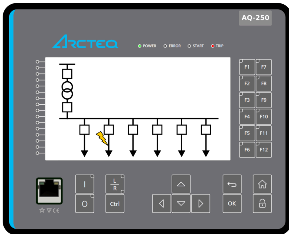
Figure. 5.6 - 106. Example mimic where sensor activation location is indicated with a symbol.
