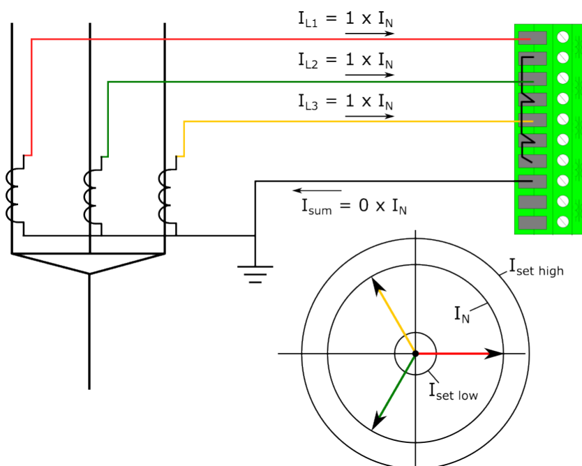
Figure. 4.6.1 - 87. All works properly, no faults.
