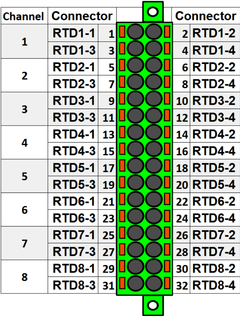
Figure. 7.4.4 - 125. RTD input module connectors.
