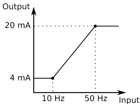
Figure. 4.5.6 - 81. Example of the effects of mA output channel settings.
