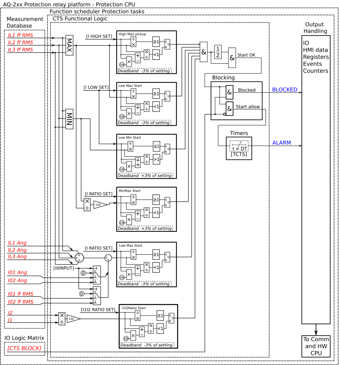
Figure. 4.6.1 - 86. Simplified function block diagram of the CTS function.
