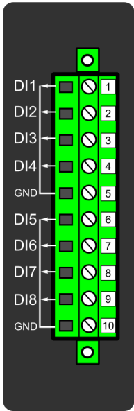
Figure. 7.4.1 - 121. Digital input module (DI8) with eight add-on digital inputs.
