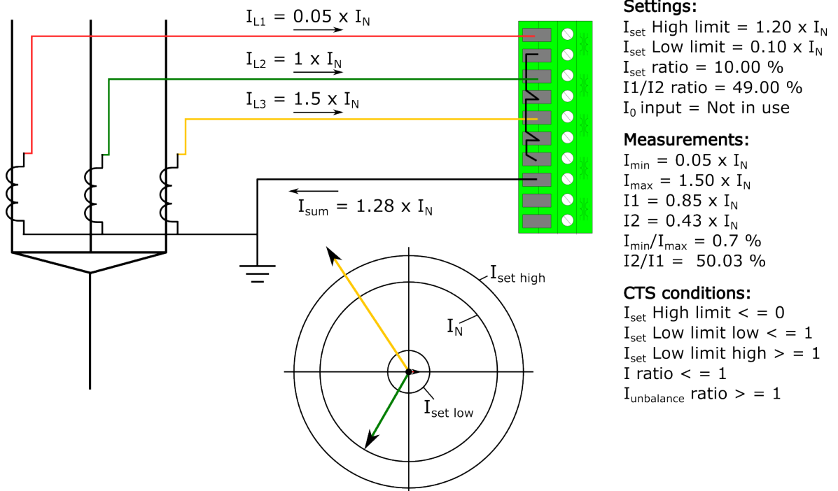
Figure. 4.6.1 - 90. No wiring fault but heavy unbalance.
