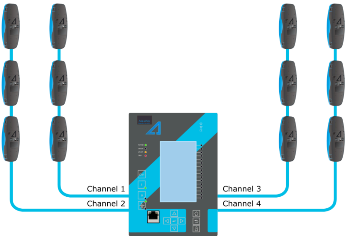
Figure. 4.4.12 - 68. Protection relay equipped with arc protection.
