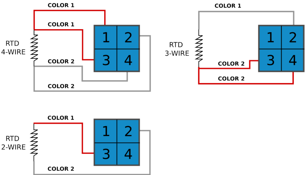
Figure. 7.4.4 - 126. RTD sensor connection types.
