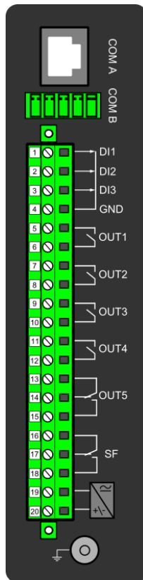
Figure. 7.2 - 119. CPU module.
