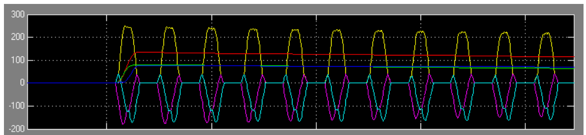
Figure. 4.4.9 - 63. Example of transformer magnetizing inrush currents.
