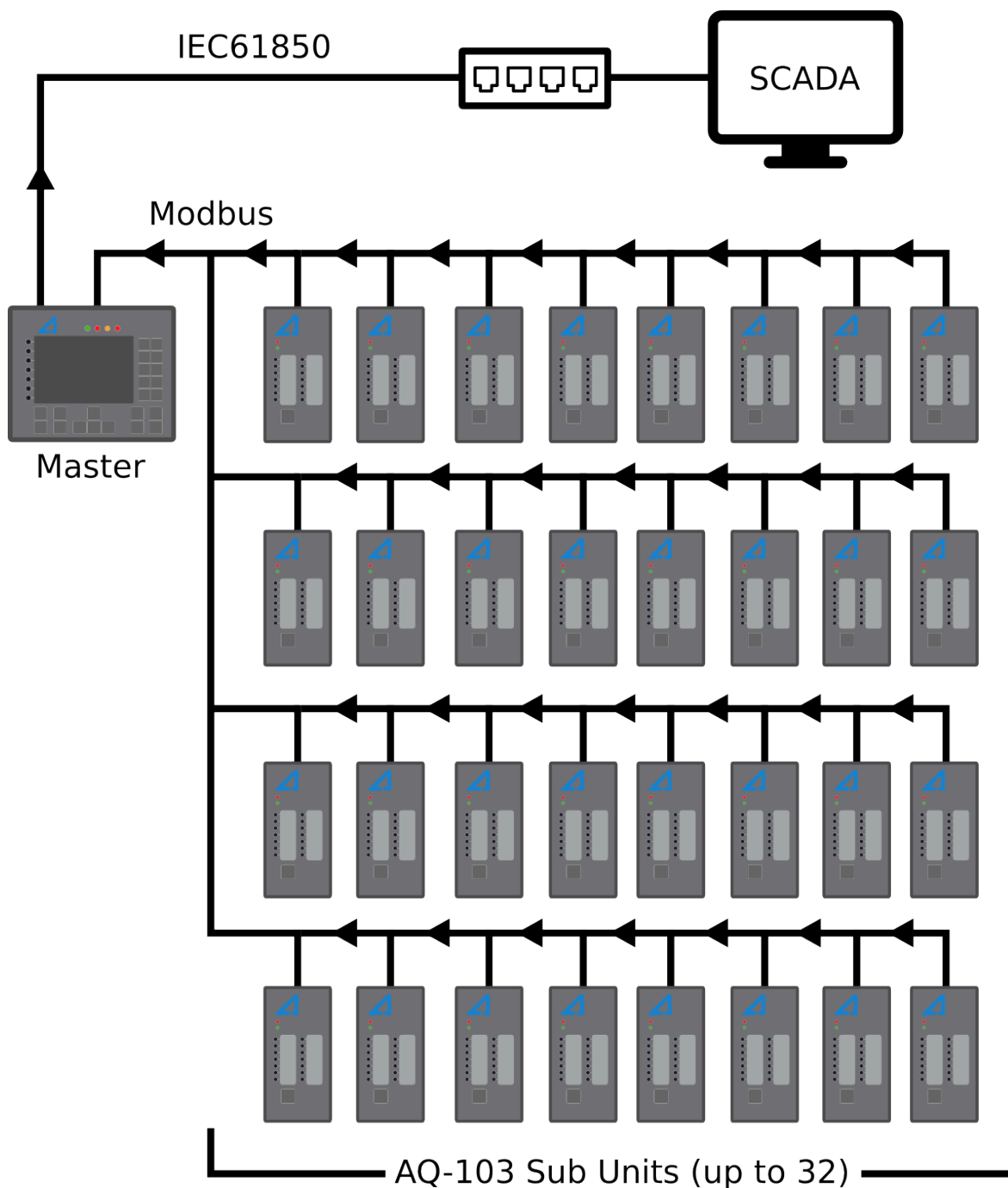
Figure. 5.6 - 104. AQ-250 device can receive signals through modbus and use them to control logic of the device, create mimics and report the values to IEC 61850.
