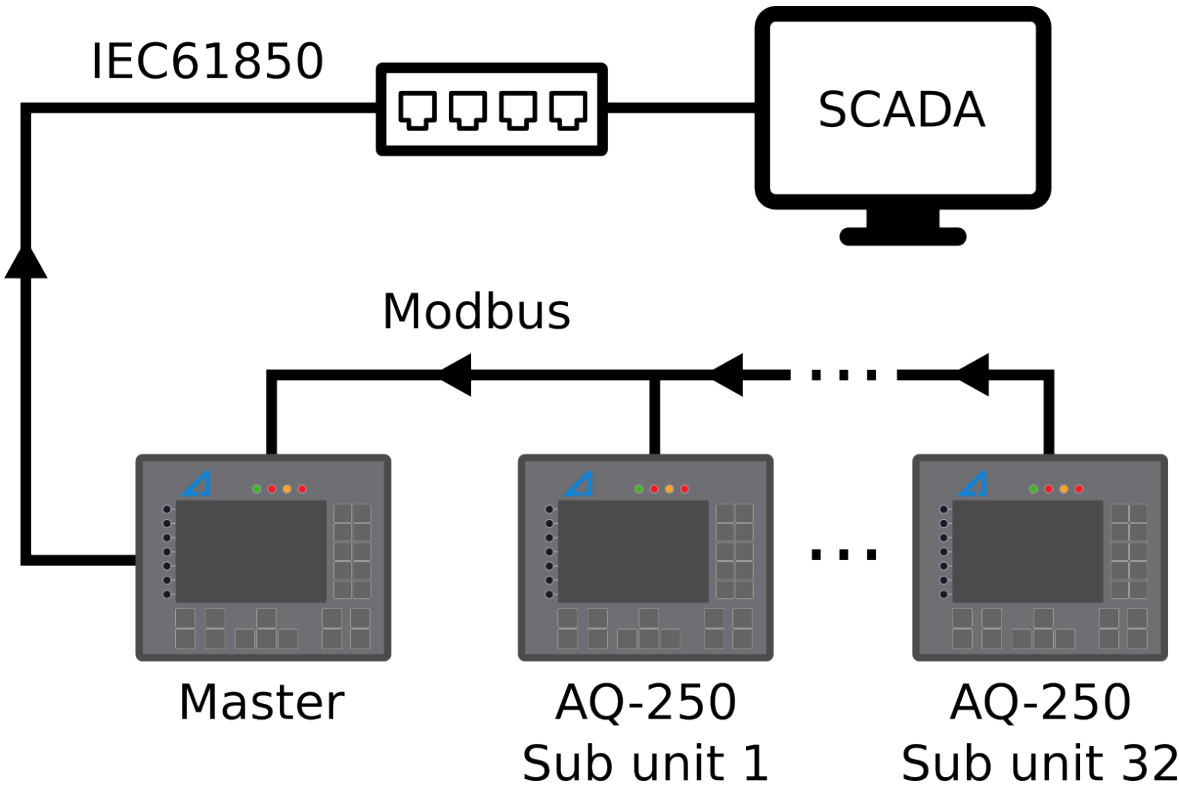
Figure. 5.6 - 103. Example setup of Modbus Gateway application.
