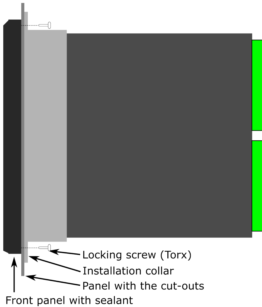
Figure. 7.5 - 136. Device installation.
