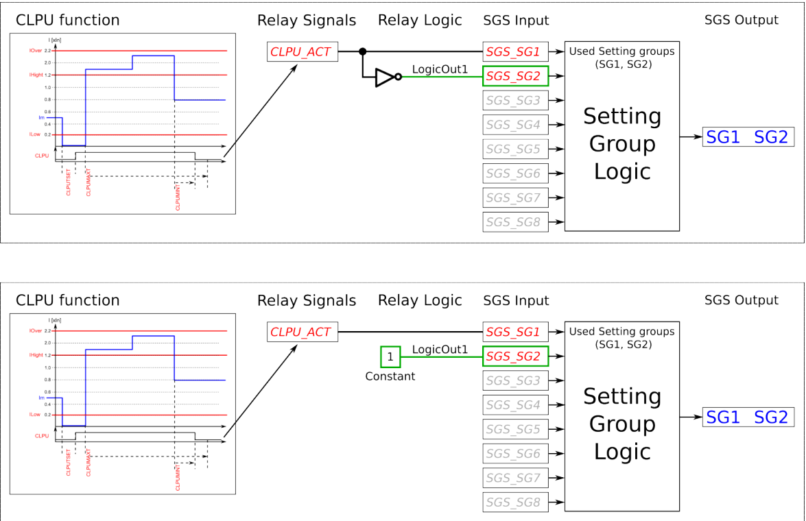
Figure. 4.5.2 - 76. Entirely application-controlled setting group change with the cold load pick-up function.
