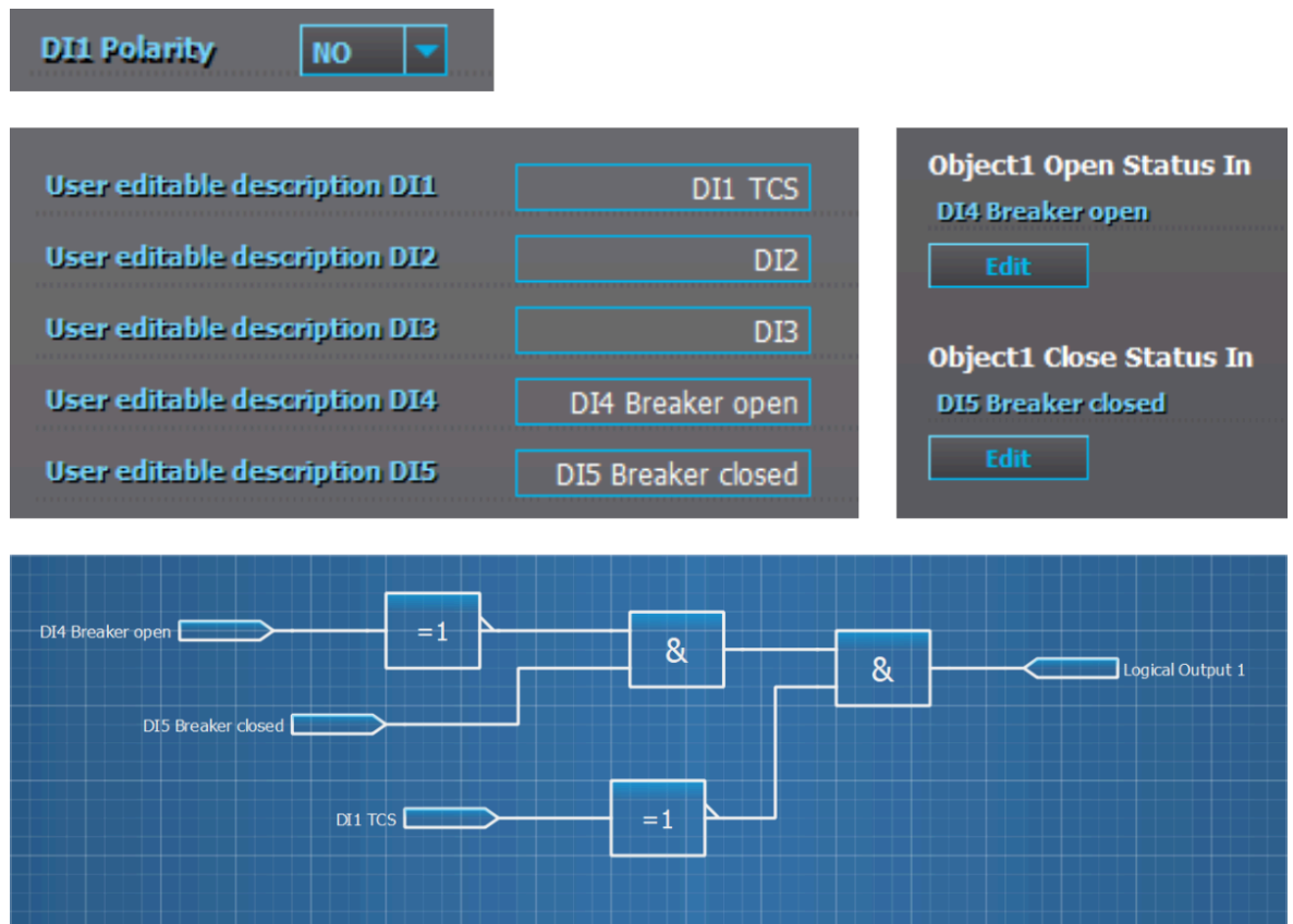
Figure. 6.3 - 115. Example block scheme.
