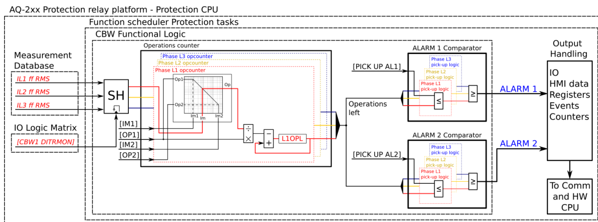
Figure. 4.6.2 - 97. Simplified function block diagram of the circuit breaker wear function.
