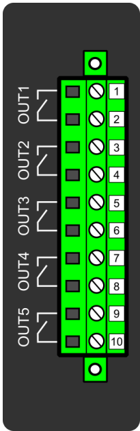
Figure. 7.4.2 - 123. Digital output module (DO5) with five add-on digital outputs.
