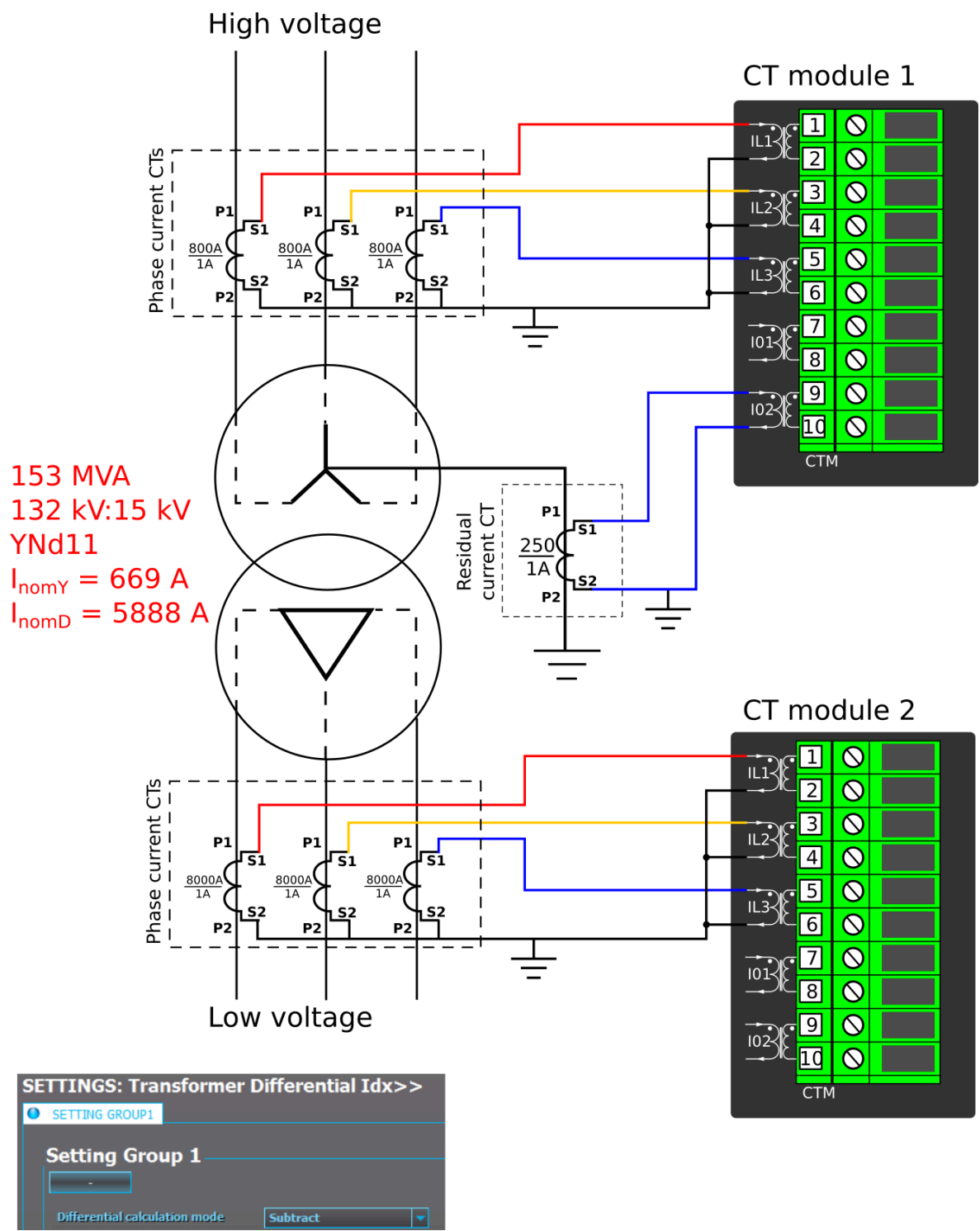
Figure. 4.2.1 - 4. Connections (application 1).
