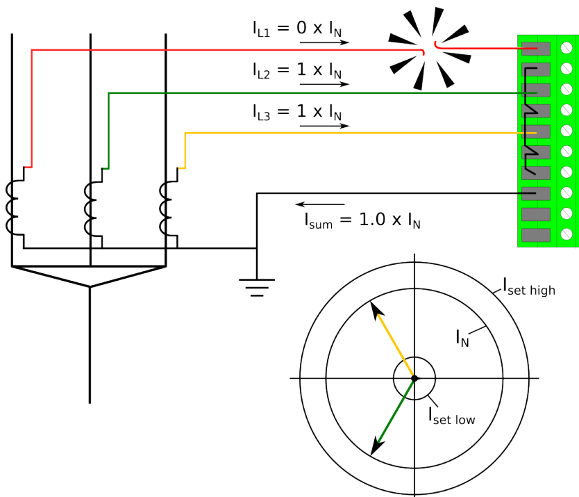
Figure. 4.6.1 - 88. Secondary circuit fault in phase L1 wiring.
