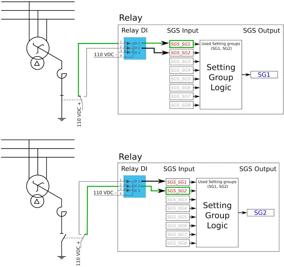
Figure. 4.5.2 - 74. Setting group control – two-wire connection from Petersen coil status.
