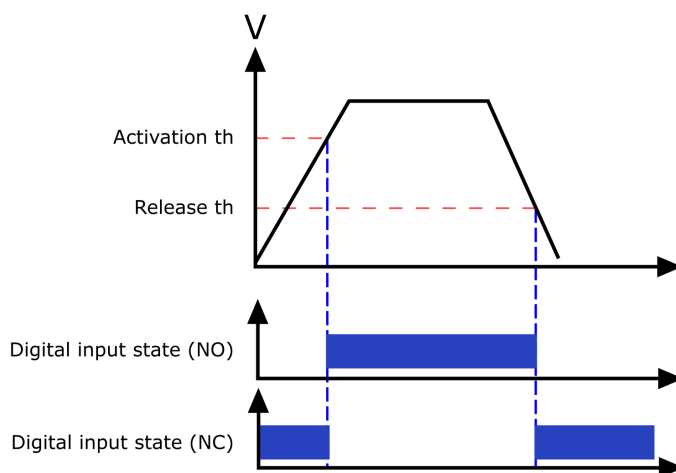
Figure. 7.4.1 - 122. Digital input state when energizing and de-energizing the digital input channels.
