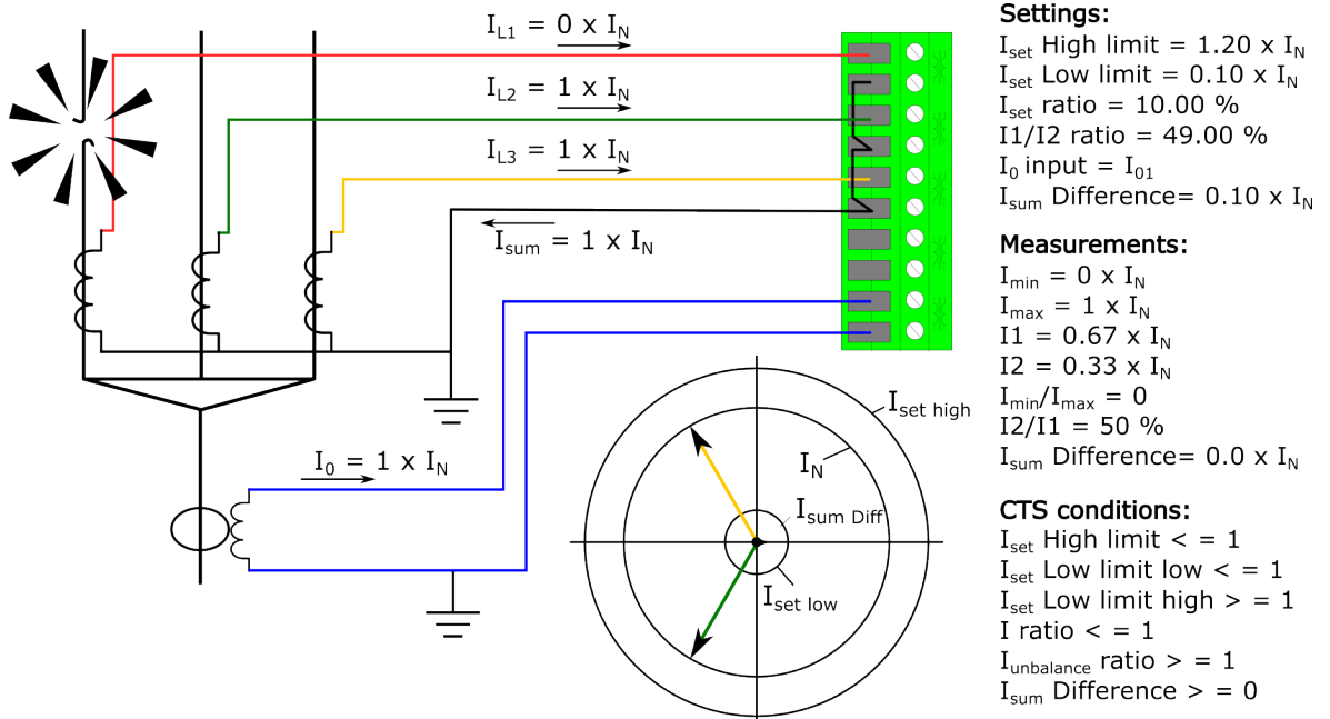
Figure. 4.6.1 - 94. Broken primary phase current wiring.
