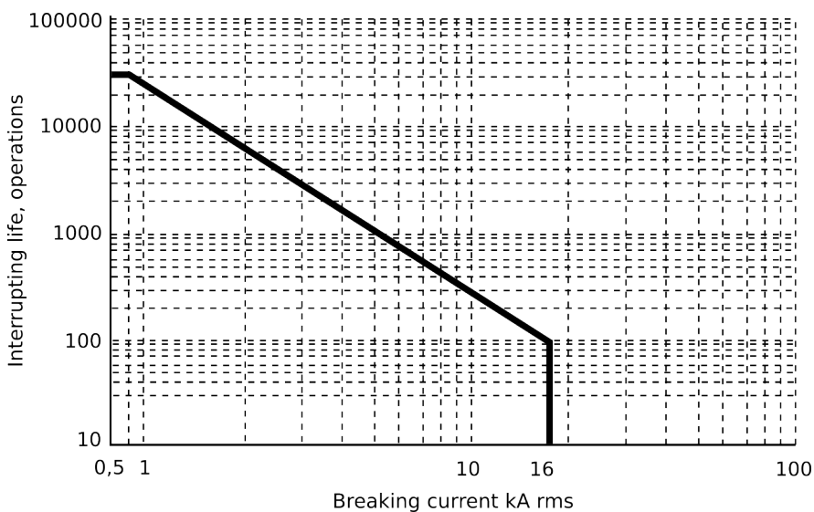
Figure. 4.6.2 - 96. Example of the circuit breaker interrupting life operations.
