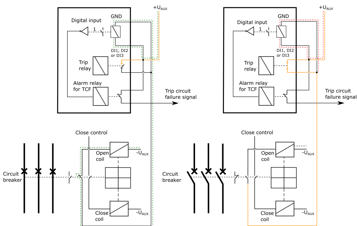
Figure. 6.3 - 114. Trip circuit supervision with one DI and one latched output contact.
