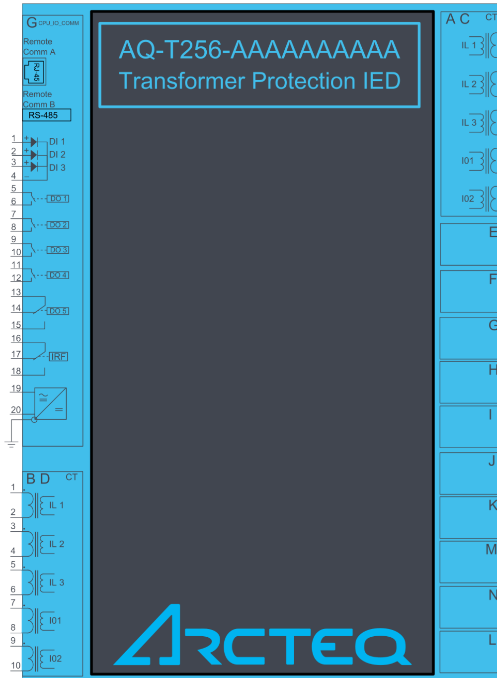
Figure. 6.1 - 107. AQ-T256 variant without add-on modules.
