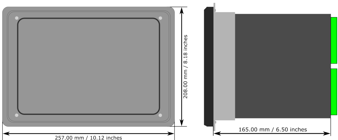
Figure. 7.5 - 135. Device dimensions.
