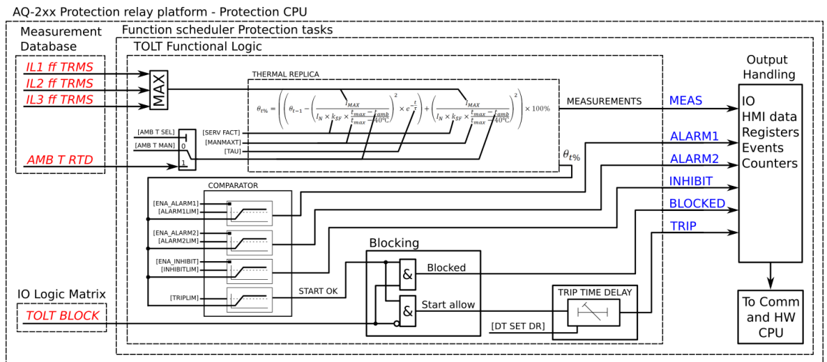
Figure. 4.4.8 - 40. Simplified function block diagram of the TT> function.
