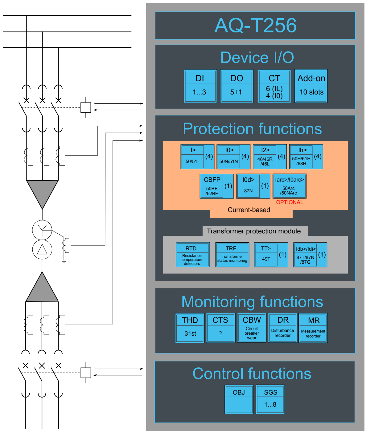
Figure. 6.1 - 109. AQ-T256 application example with function block diagram.
