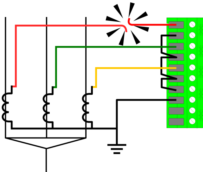
Figure. 4.6.1 - 85. Secondary circuit fault in phase L1 wiring.
