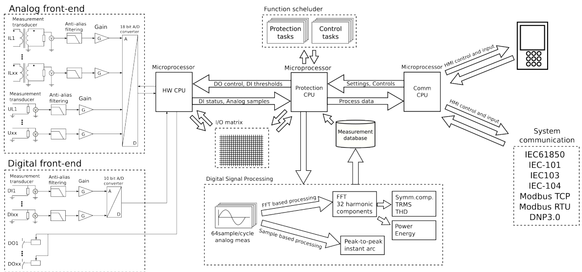
Figure. 4.4.1 - 9. Principle diagram of the protection relay platform.
