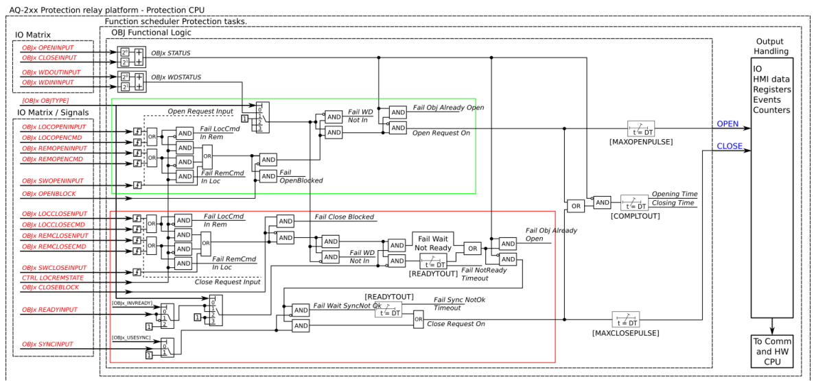
Figure. 4.5.3 - 77. Simplified function block diagram of the object control and monitoring function.
