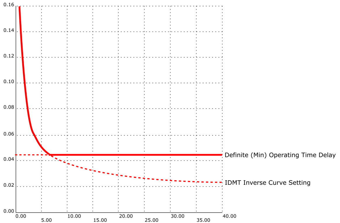
Figure. 4.4.1 - 12. Operating time delay: Definite (Min) and the minimum for tripping.
