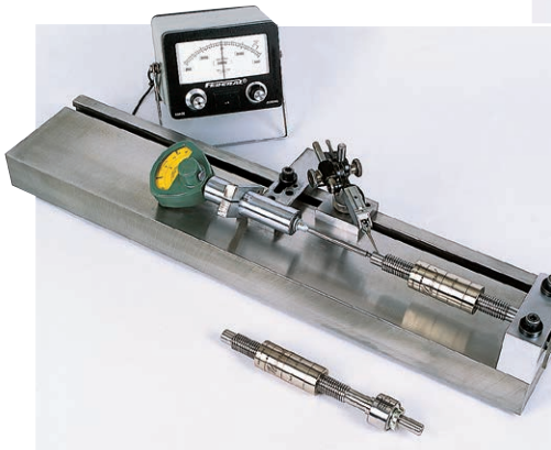
Inspection of bearing for thrust plane error.
