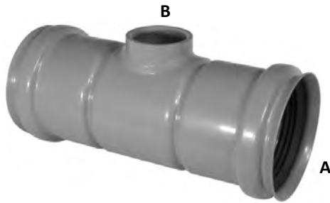
OLD GHEEN # 7225
