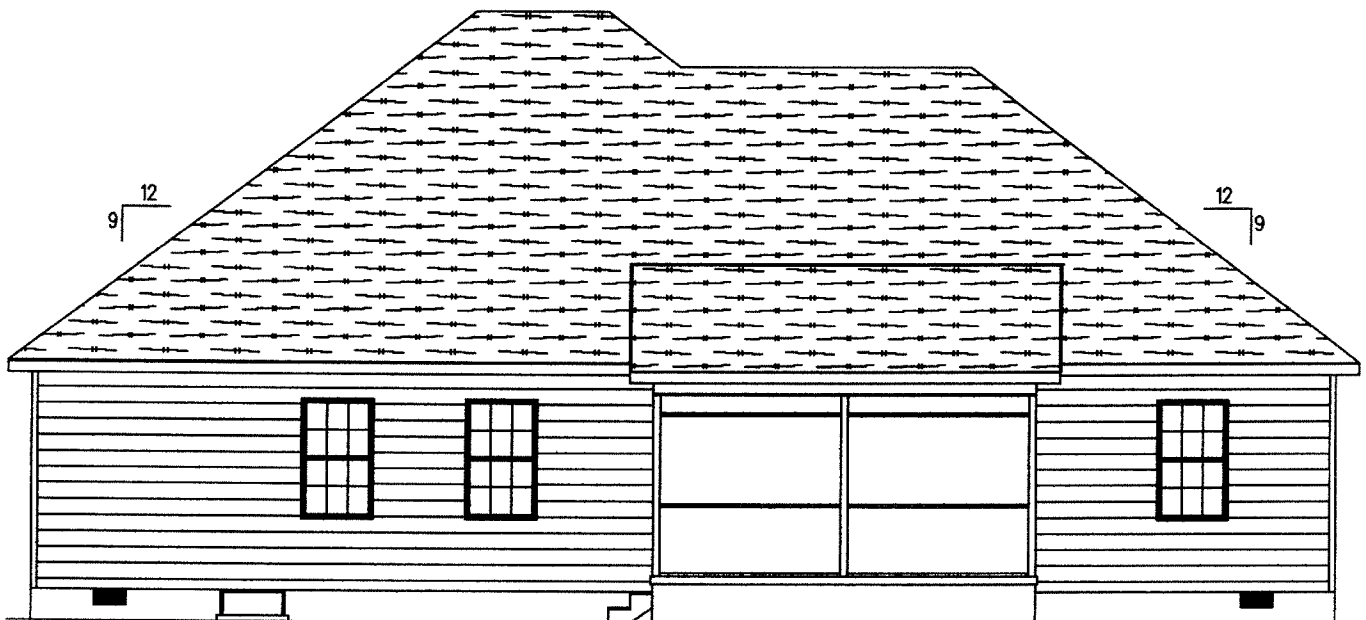
REAR ELEVATION
