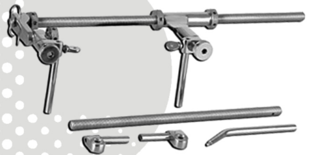
▲ LARGE DISTRACTOR FOR TIBIA & FEMUR [Catalog No. : B.120.006]
