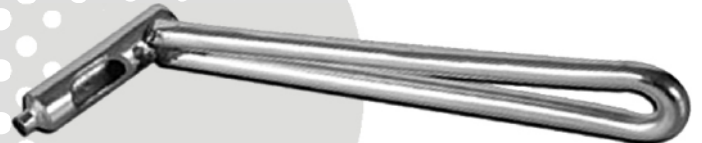
▲ DRILL SLEEVE 2.0mm [Catalog No. : B.089.023]
