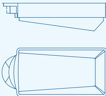
DENE B P 6 6.40 x 2.95 | Prof. 1.10/1.75 m
