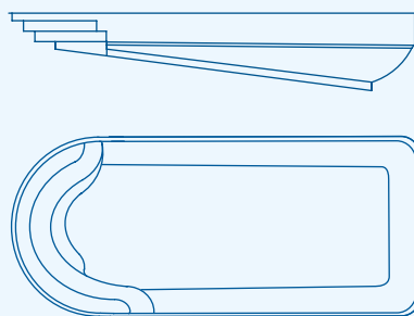
LIRA 9 9.50 x 3.80 m | Prof. 0.85/1.85 m
