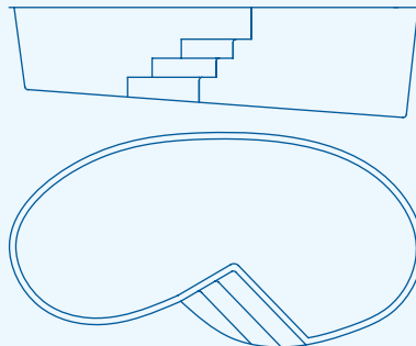
OPORTO 6.40 x 2.95/3.30 m | Prof. 1.75/1.25 m
