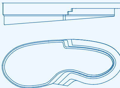
ELIPSA 1000 9.95 x 4.25/3.85 m | Prof. 1.80/1.05 m
