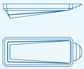
ROMAINE 11.40 x 4.20 m Prof. 2.10/0.85 m
