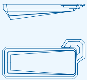
PRIVILEGE 11.40 x 5.20 m Prof. 2.10/0.85 m
