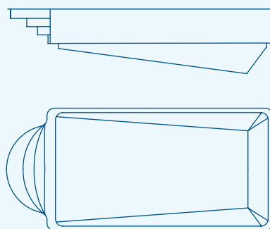
DENE B P 7 7.25 x 3.30 m | Prof. 1.10/1.70 m
