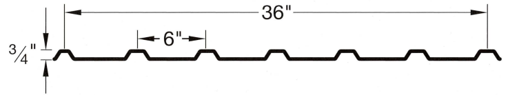
PBU Panel
