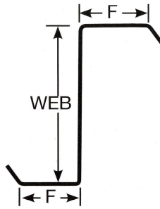
Zee Purlin
