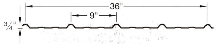
PBU Panel
