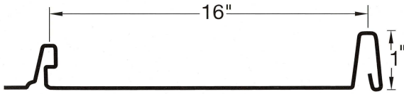
1" Nail Strip Panel
