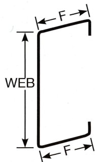
Eave Strut double broke, low side
