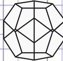
DODECAHEDRON Made of 12 Pentagons (Ether)
