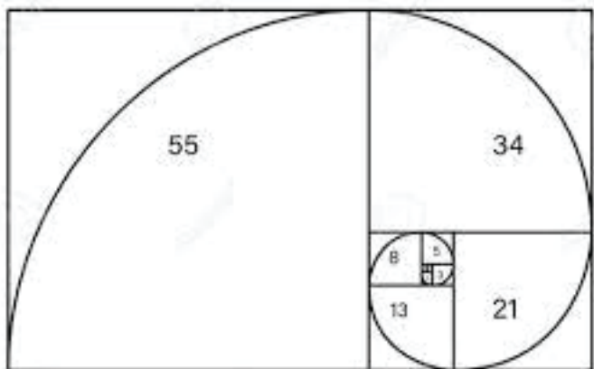
Golden Ration (above image) - a sequence of numbers 0,1,1,2,3,5,8,13,21 that are added together to make the next number.
