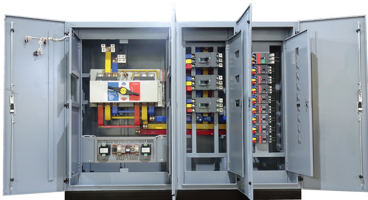
Main Distribution Panel/ Mechanical Automatic Transfer Switch (MDP/ATS)
