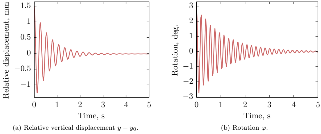
Figure 13: Dynamic simulation with perturbation of \Delta y = 1.5 mm and \Delta\varphi = 3^\circ with constraint in horizontal displacement x .
