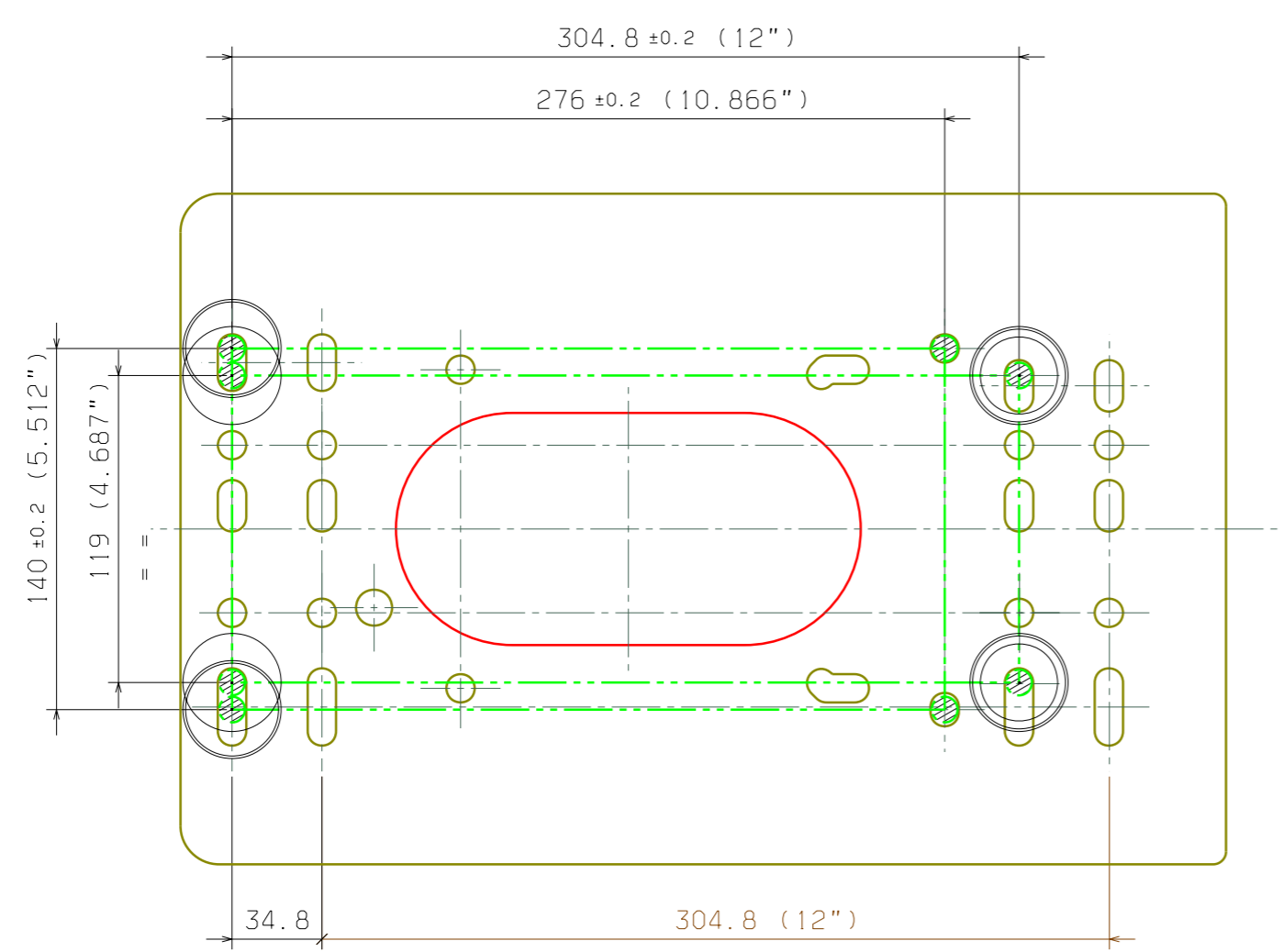
SEAT MOUNTING DIAGRAM
