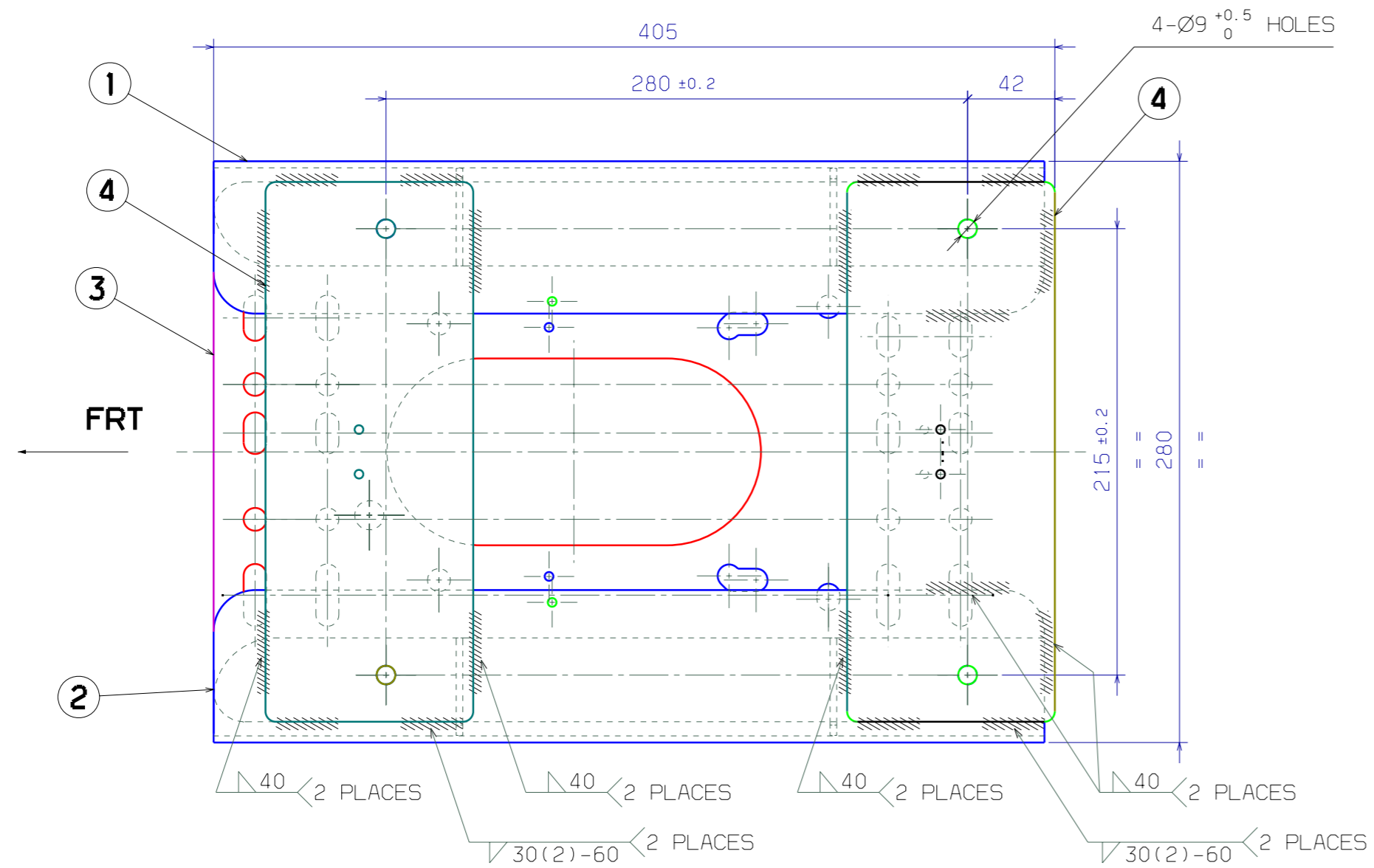
SEAT MOUNTING DIAGRAM
