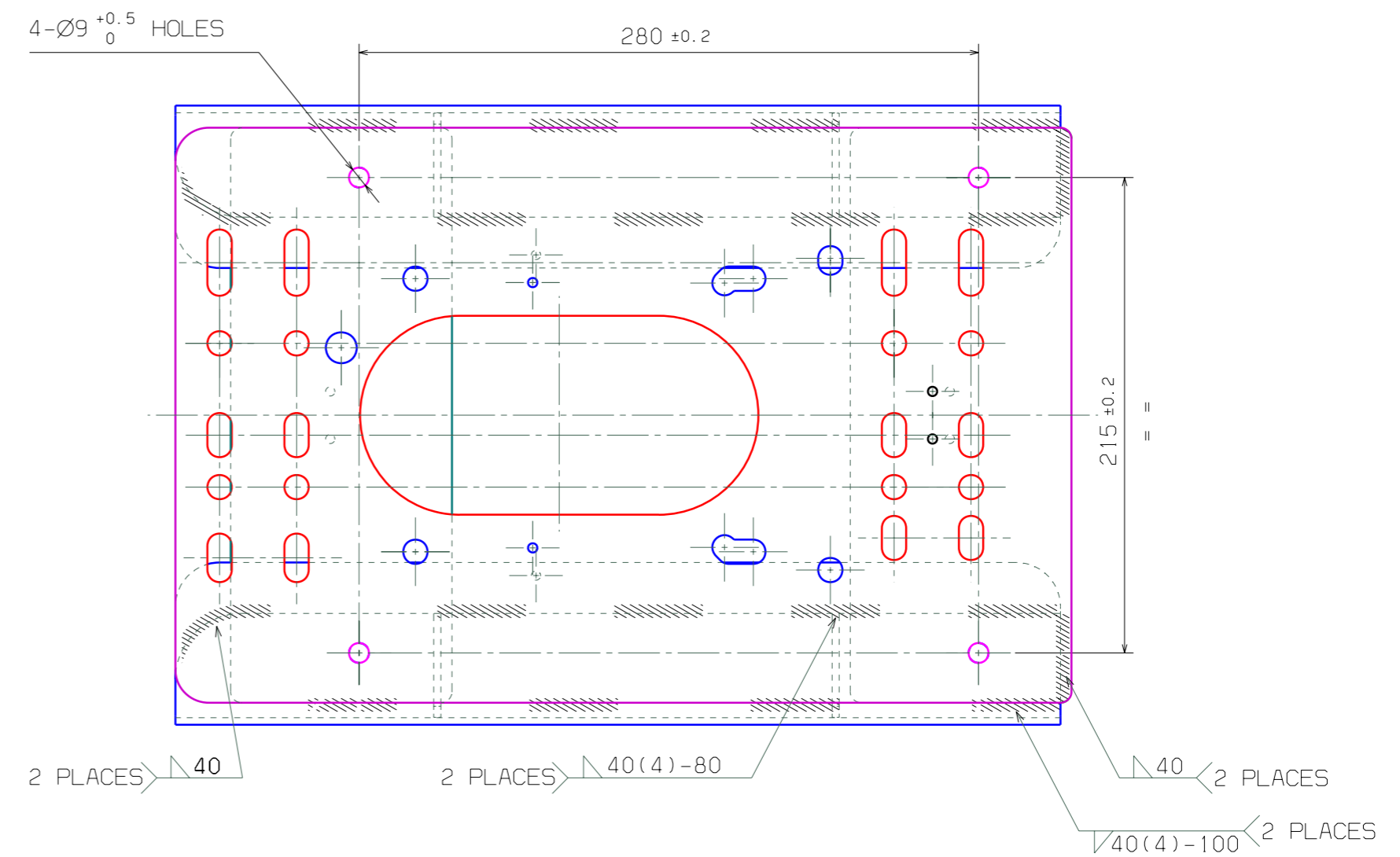
VIEW - A
