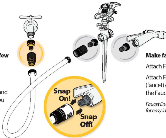
46C Metal Product End Connector with Water Stop
