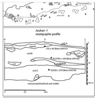
Figure 3. Site plan and stratigraphic profile drawings of Juukan-1.
