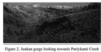
Figure 2. Juukan gorge looking towards Pulykunti Creek
