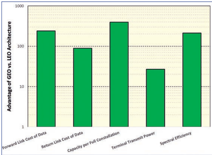
Figure 1. Comparison of LEO and GEO Metrics
