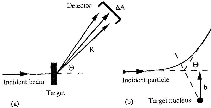
Fig. 1.14. Scattering (a) macroscopic view, (b) microscopic view
