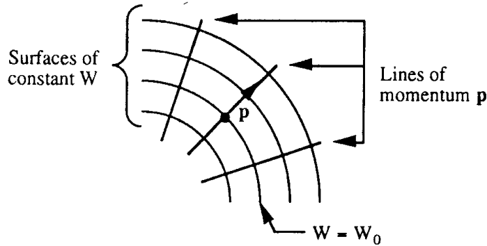
Fig. 8.06. Surfaces of constant W and lines of momentum \mathbf{p}
