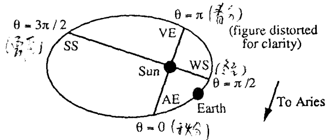
Fig. 1.13. Earth's orbit
