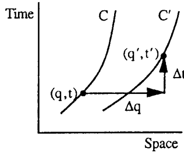
Fig. 5.06. Infinitesimal transformation of configuration space
