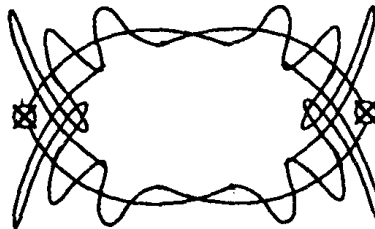
Fig. 10.14. Separatrices \Gamma_+ and \Gamma_-
