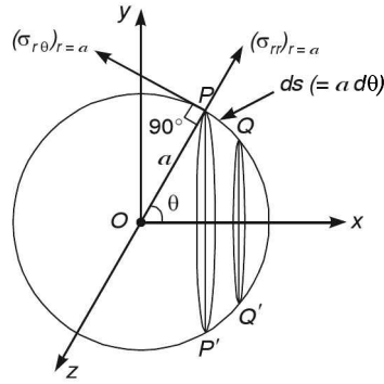
Fig. (iii) Computing the drag in Stokes flow past a sphere
