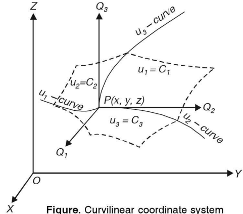
Figure. Curvilinear coordinate system
