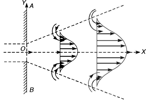
Fig. Spread of free jet
