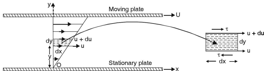
Figure showing fluid motion between a stationary plate and a moving plate. A small element shows the shear stress.
