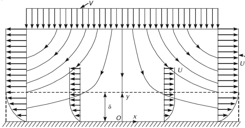
Fig. Stagnation in plane flow
