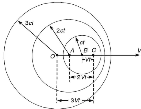
Fig. (ii) V < c , M < 1 . Subsonic flow
