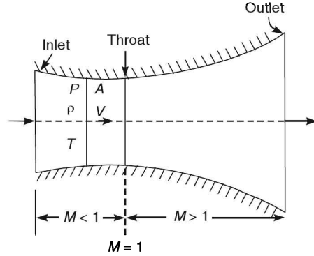
Figure. Laval nozzle
