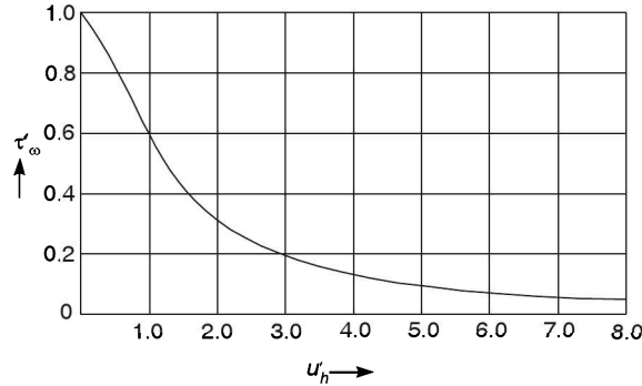
Fig.(ii) Dimensionless shearing stress on the stationary plate in variable viscosity. Plane Couette flow.
