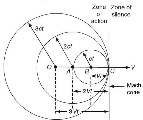
Fig. (iv) V = c, M = 1 . Sonic flow
