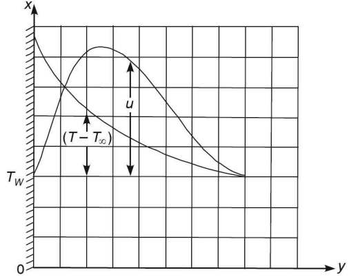
Fig. Temperature and velocity distributions in free convection from a heated vertical plate.
