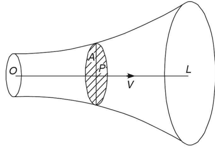
Fig. Flow through stream tube
