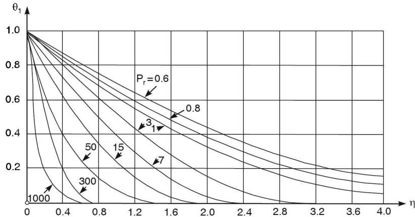
Fig. Temperature distribution in a heated flat plate at zero incidence with small velocity plotted for various Prandtl numbers. Pr (frictional heat neglected)
