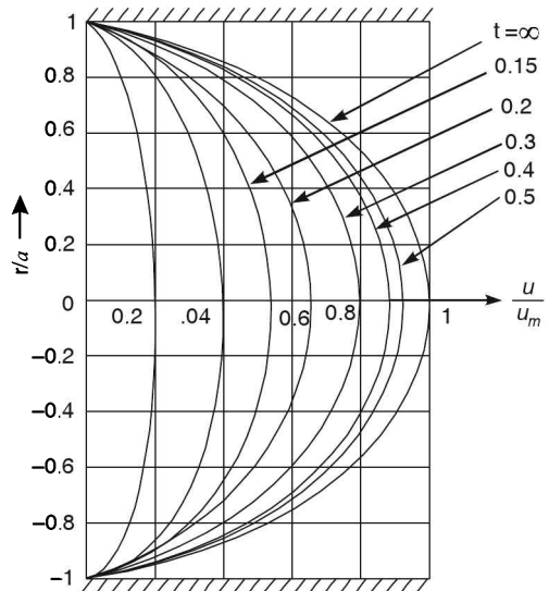
Fig. Velocity distribution for unsteady (starting) flow in a circular pipe
