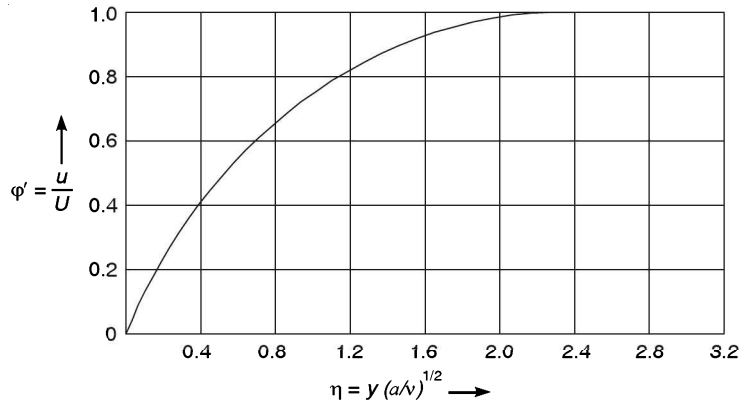
Fig. Velocity distribution in plane stagnation point flow
