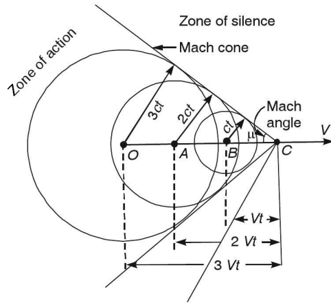
Fig. (iii) V > c, M > 1 . Supersonic flow
