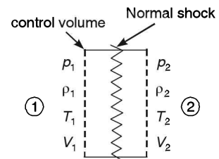
Fig. Flow model for normal shock
