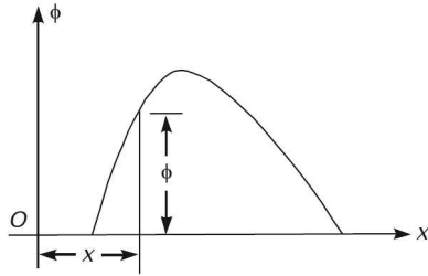
Fig. (i) Profile at t
