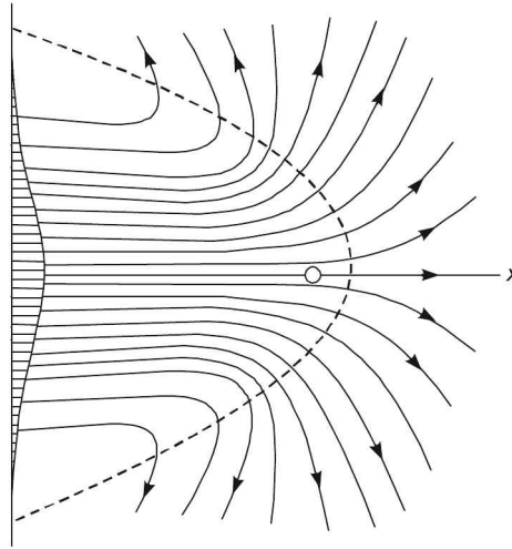
Figure showing streamlines in the flow past a sphere from Oseen's solution
