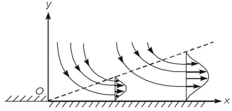
Fig. Spread of a plane wall jet
