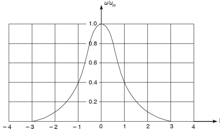
Fig. Velocity distribution in a two-dimensional free jet.
