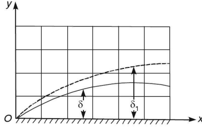
Fig. (i) Pr < 1
