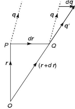
(iv) Rate of angular deformation
