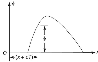
Fig. (ii) Profile at (t + T)
