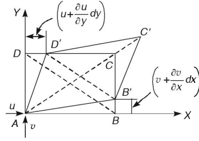
(iv) Rate of angular deformation
