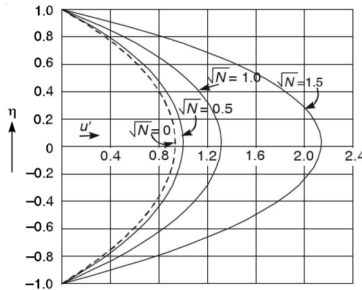
Fig. (ii) Velocity distribution in variable viscosity plane Poiseuille flow ( N = \beta Ec Pr )
