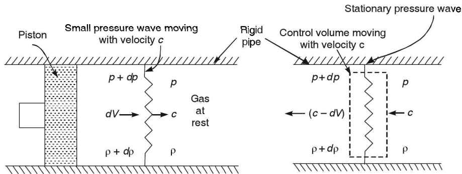
Fig. (i) Propagating wave front
