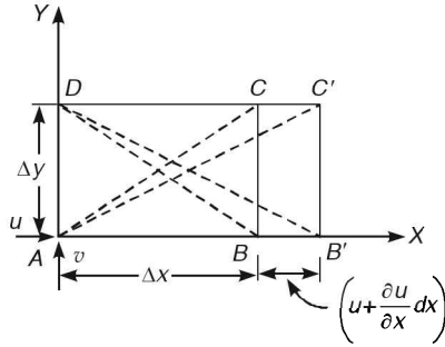
(iii) Rate of linear deformation
