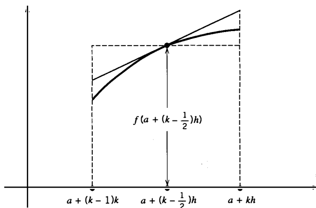
Figure 7.4.1 The tangent trapezoid.
