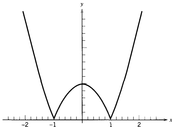
Figure 6.1.1 The function |f|(x) = |x^2 - 1| .
