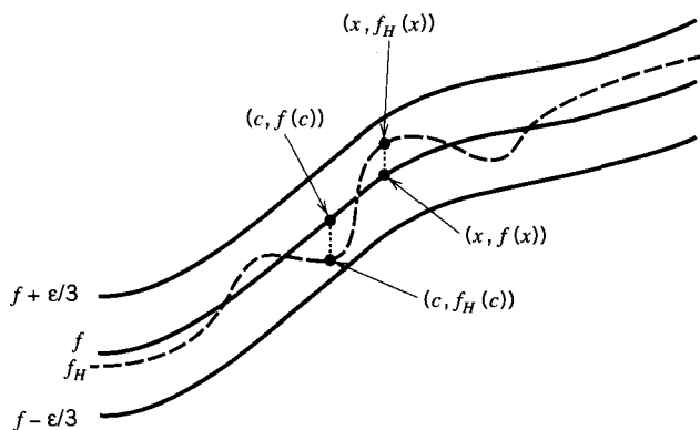
Figure 8.2.2 |f(x) - f(c)| < \varepsilon .
