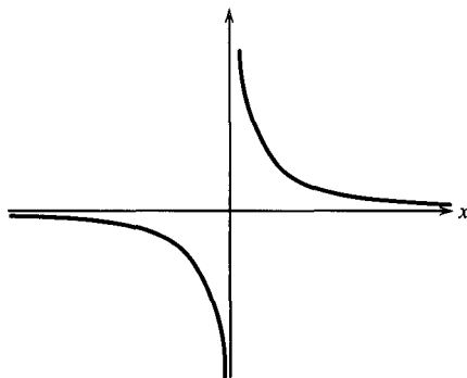
Figure 4.3.4 Graph of g(x) = 1/x ( x \neq 0 )
