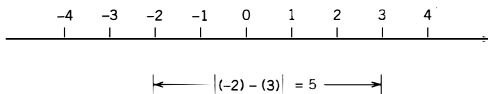
Figure 2.2.1 The distance between a = -2 and b = 3
