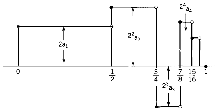
Figure 10.2.1 The graph of \varphi .
