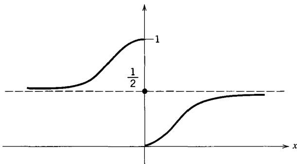
Figure 4.3.2 Graph of h(x) = 1/(e^{1/x} + 1) ( x \neq 0 ).
