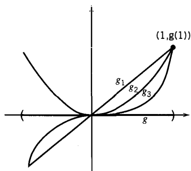
Figure 8.1.2 g_n(x) = x^n .
