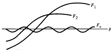
Figure 8.1.4 F_n(x) = \sin(nx + n)/n .
