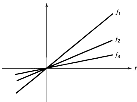
Figure 8.1.1 f_n(x) = x/n .
