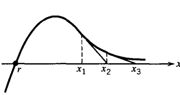
Figure 6.4.3 x_n \rightarrow \infty .
