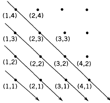
Figure 1.3.1 The set \mathbb{N} \times \mathbb{N}
