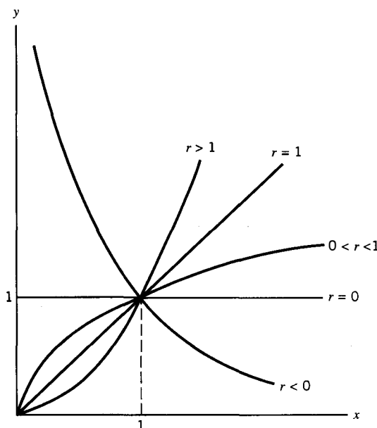
Figure 5.6.8 Graphs of x \rightarrow x^r ( x \geq 0 ).
