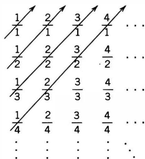
Figure 1.3.2 The set \mathbb{Q}^+
