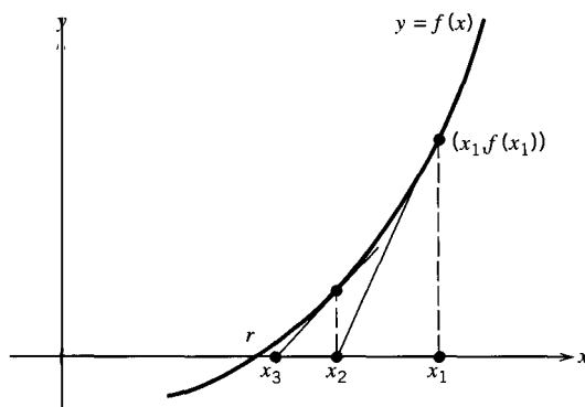
Figure 6.4.2 Newton's Method
