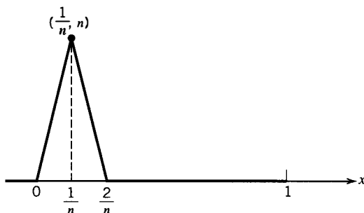
Figure 8.2.1 Example 8.2.1(c).
