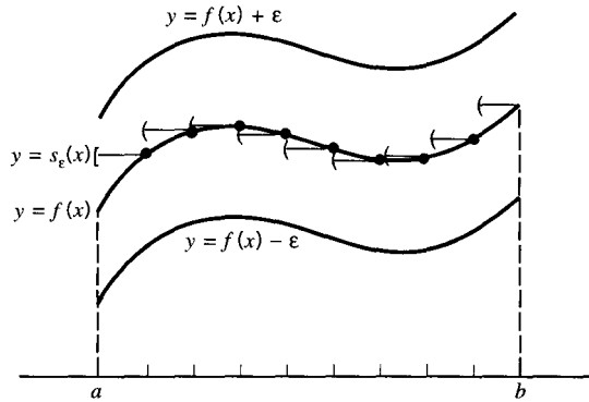
Figure 5.4.4 Approximation by step functions.
