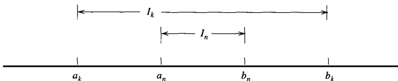
Figure 2.5.2 If k < n , then I_k \supseteq I_n
