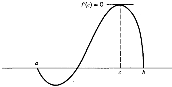
Figure 6.2.1 Rolle's Theorem
