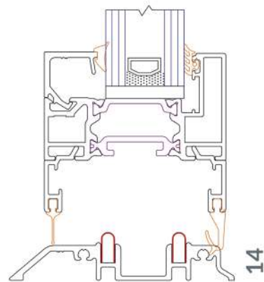
LEVEL THRESHOLD DETAIL
