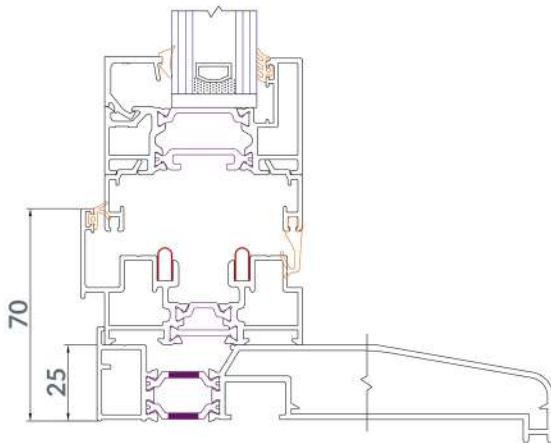
CILL & THRESHOLD DETAIL
