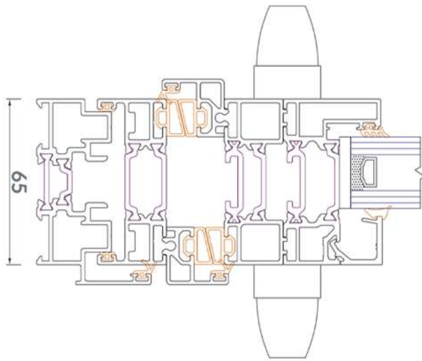
LOCK DETAIL
