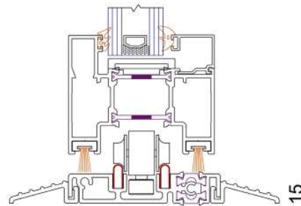
LEVEL THRESHOLD DETAIL
