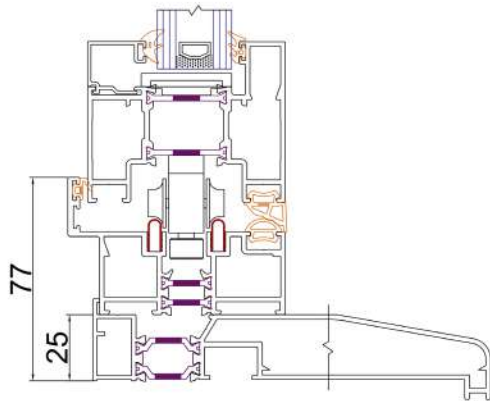
CILL & THRESHOLD DETAIL
