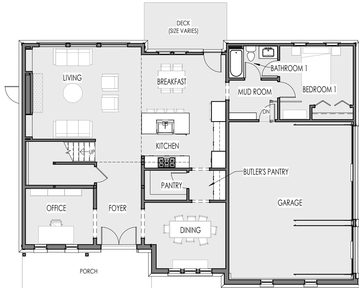
MAIN LEVEL 10' CEILING HEIGHT
