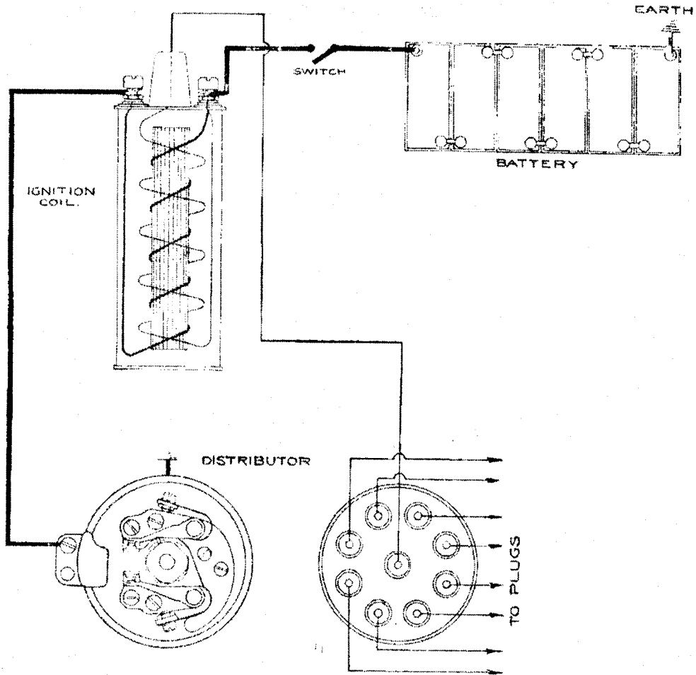
IGNITION DIAGRAM.
