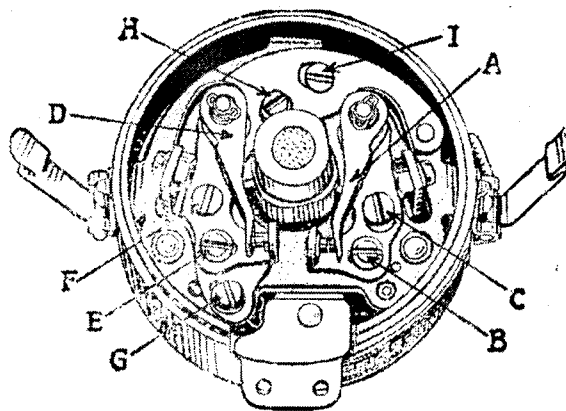
CONTACT MAKER. (Fig 6).
