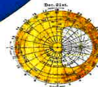
DECEMBER SOLSTICE.
