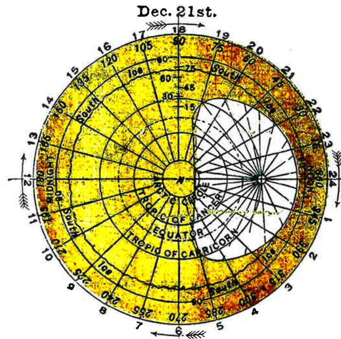
DECEMBER SOLSTICE.
