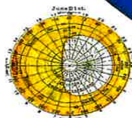
JUNE SOLSTICE.
