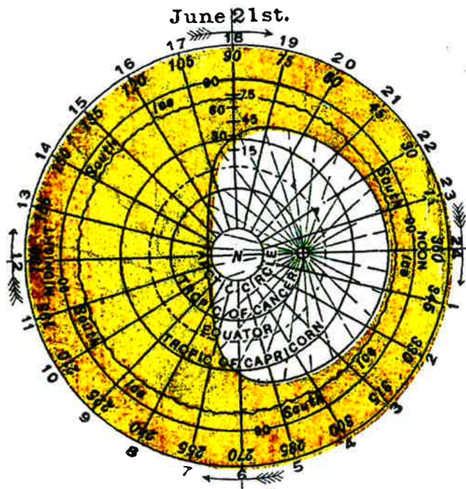
JUNE SOLSTICE.
