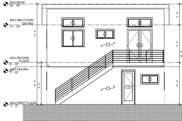
(N)NORTH ELEVATION Scale: 1/4" = 1'-0"
