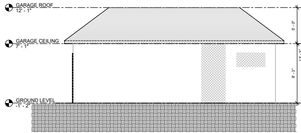
(E)NORTH ELEVATION Scale: 1/4" = 1'-0"
