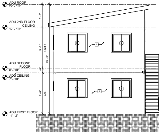
(N)EAST ELEVATION Scale: 1/4" = 1'-0"
