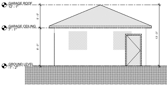
(E)EAST ELEVATION Scale: 1/4" = 1'-0"
