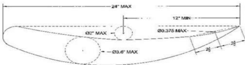
Nose wing diagram/specification
