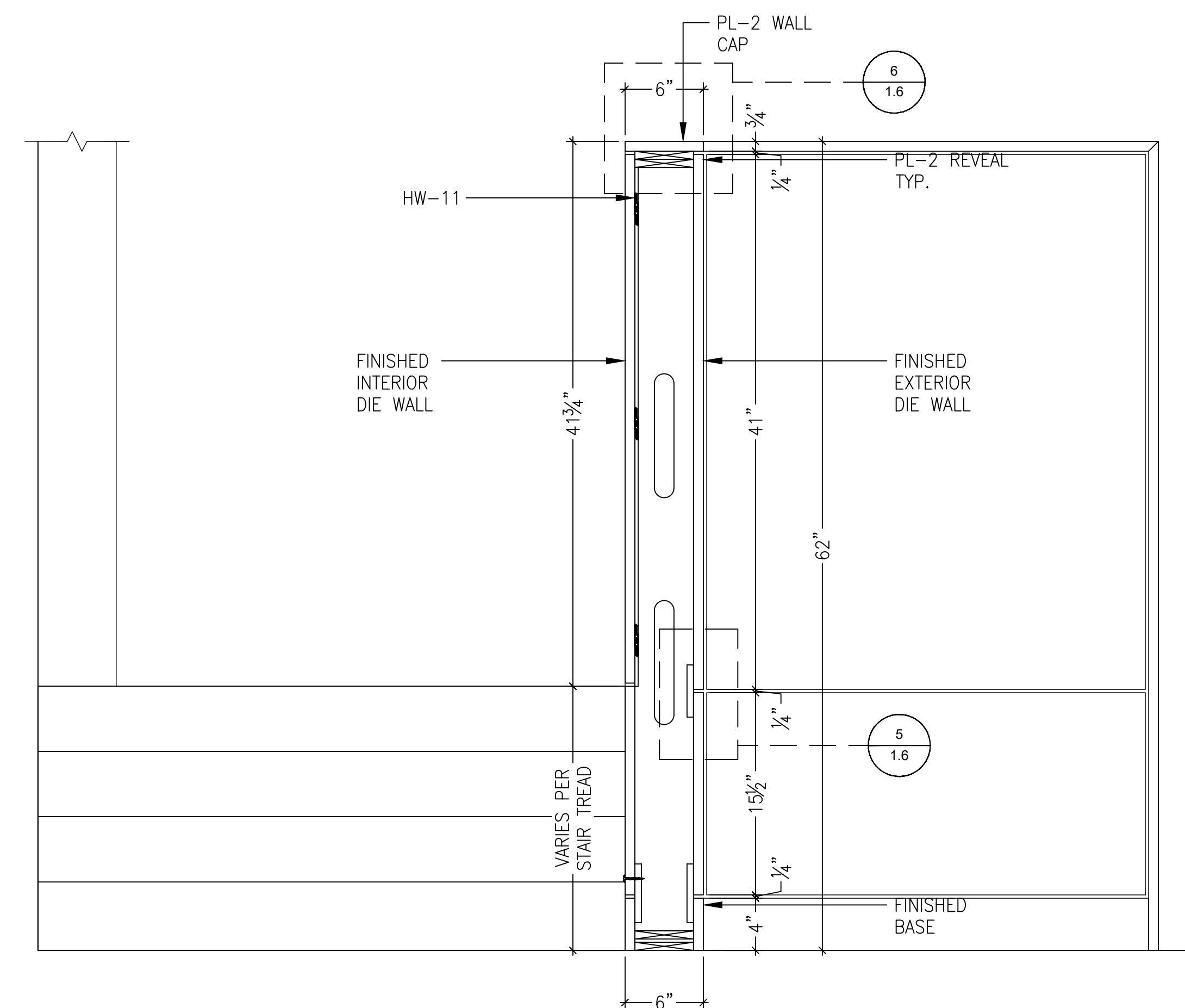
2 SECTION SCALE: 1-1/2" = 1'-0" REF: N/A
