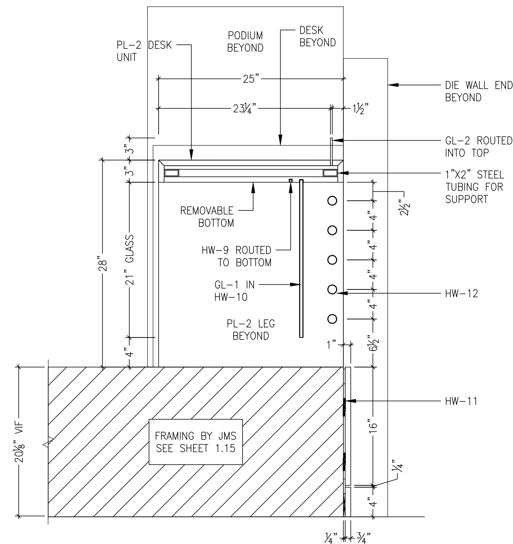
2 SECTION SCALE: 1-1/2" = 1'-0" REF: N/A
