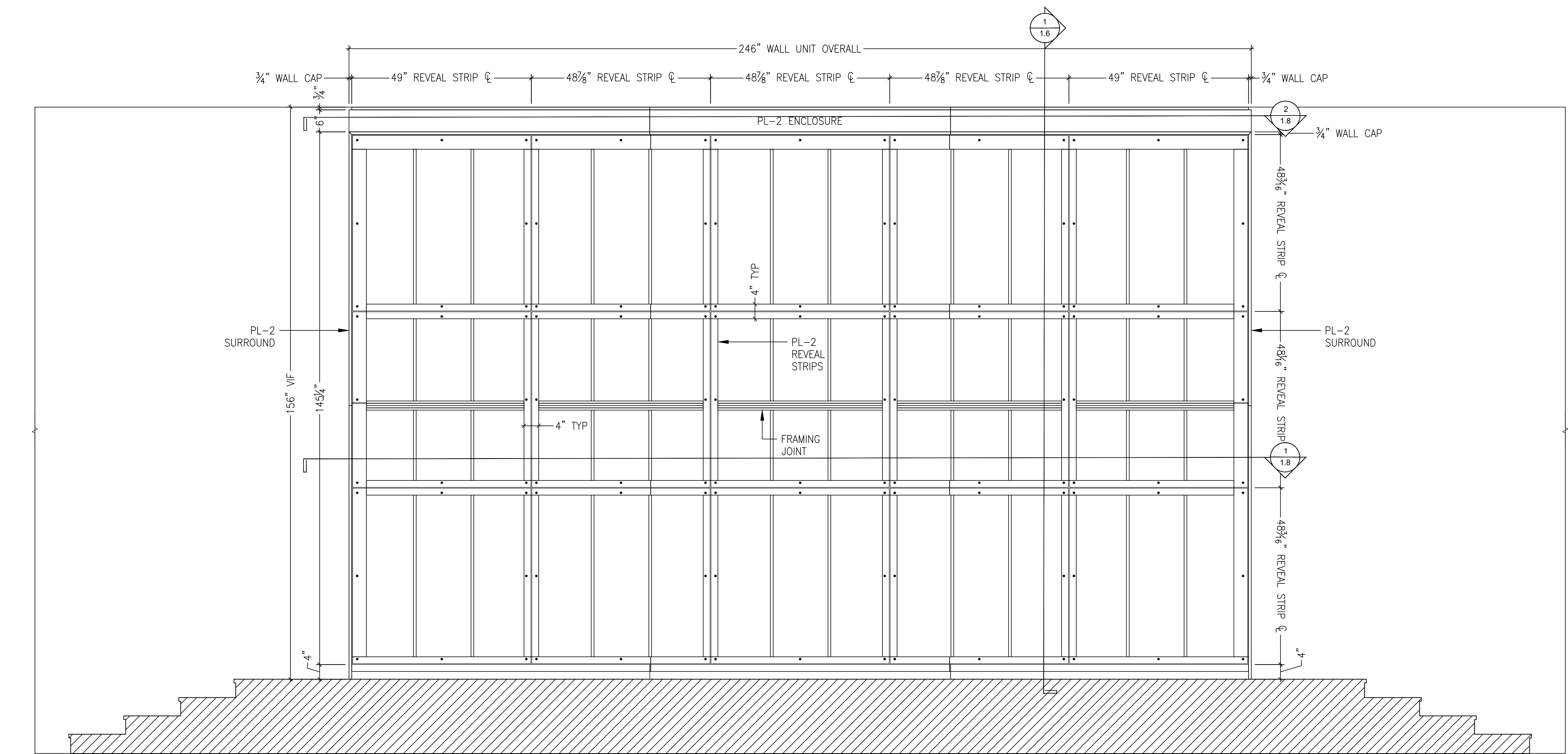
A 127 MEETING HALL STAGE - REVEAL STRIPS SCALE: 3/4" = 1'-0" REF: N/A
