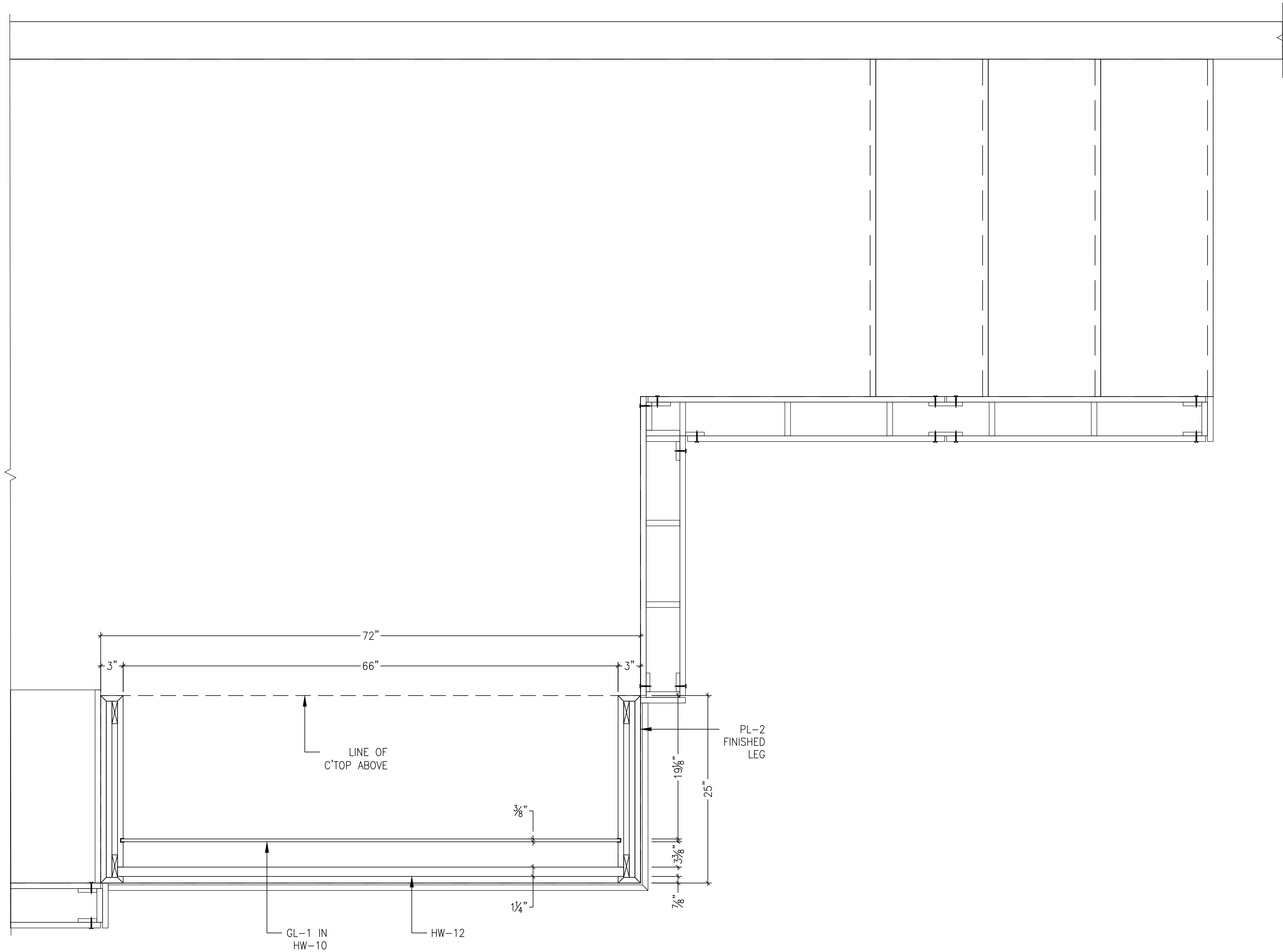
1 SECTION SCALE: 1-1/2" = 1'-0" REF: N/A
