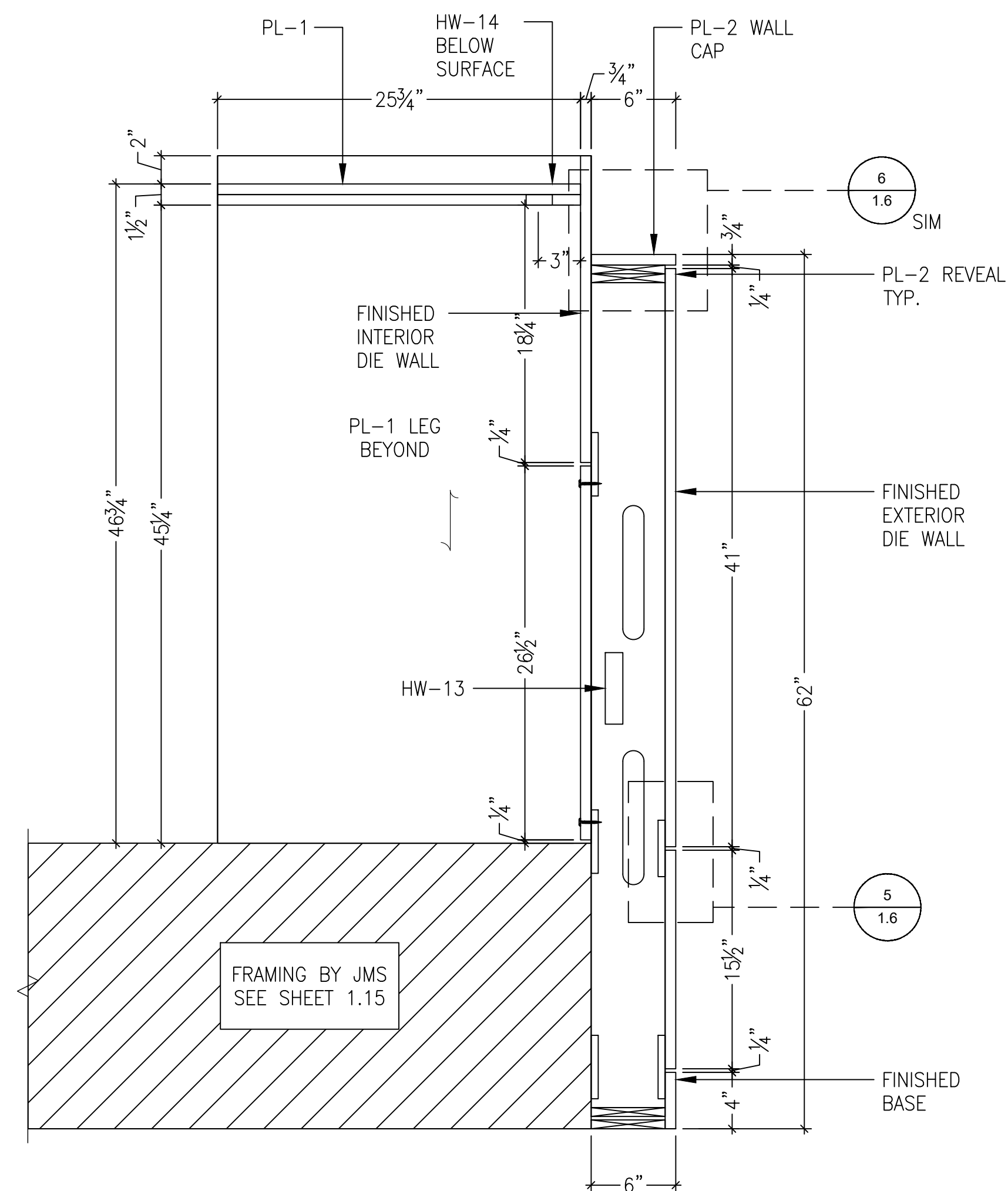
1 SECTION SCALE: 1-1/2" = 1'-0" REF: N/A
