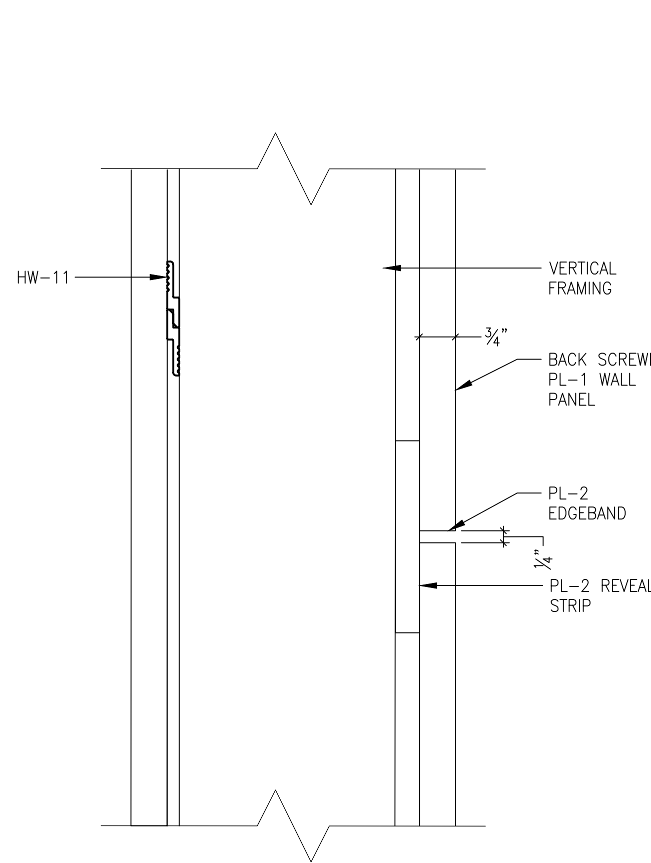
5 SECTION SCALE: 6" = 1'-0" REF: N/A
