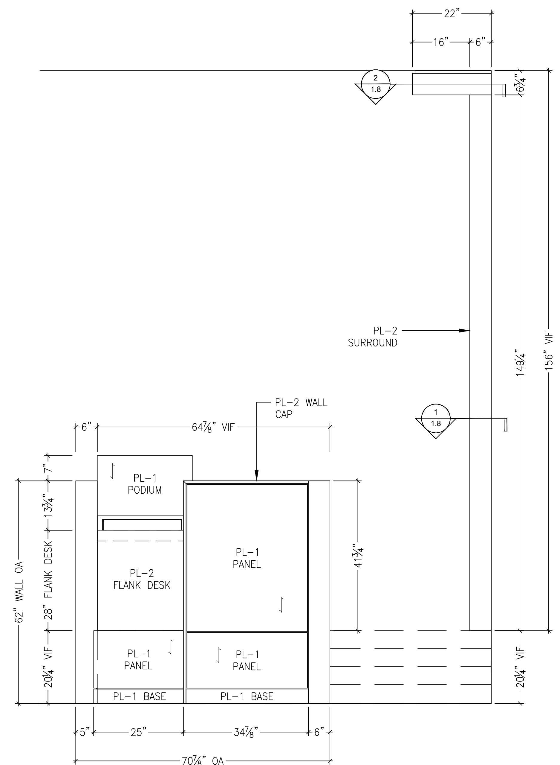
A 127 MEETING HALL STAGE SCALE: 3/4" = 1'-0" REF: N/A
