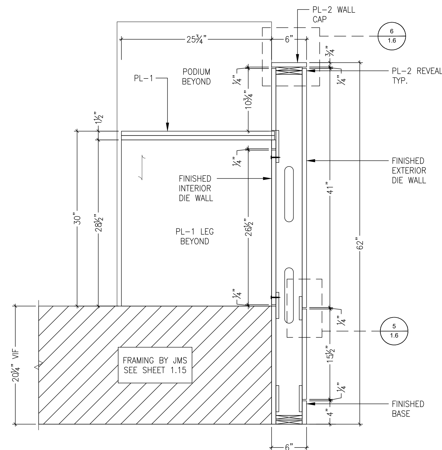
3 SECTION SCALE: 1-1/2" = 1'-0" REF: N/A
