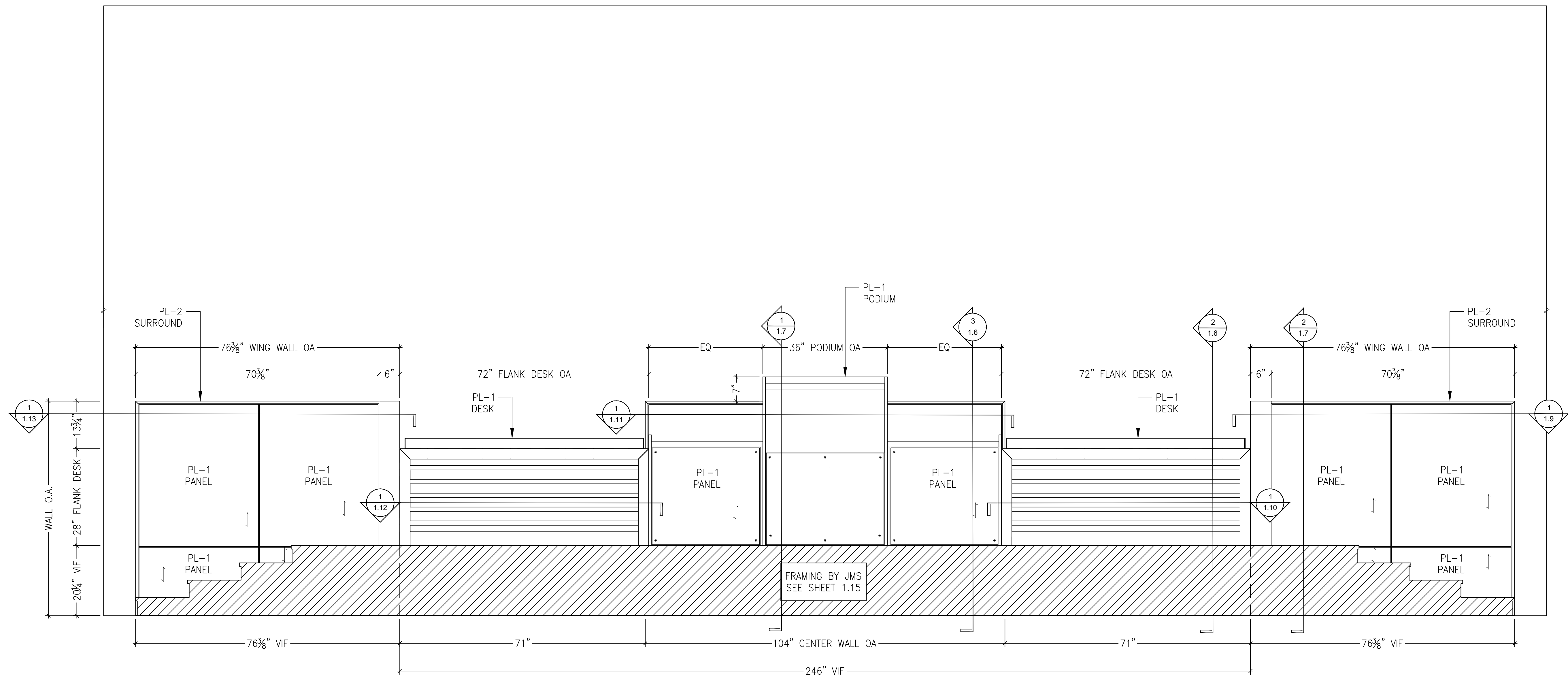
A 127 MEETING HALL STAGE SCALE: 3/4" = 1'-0" REF: N/A
