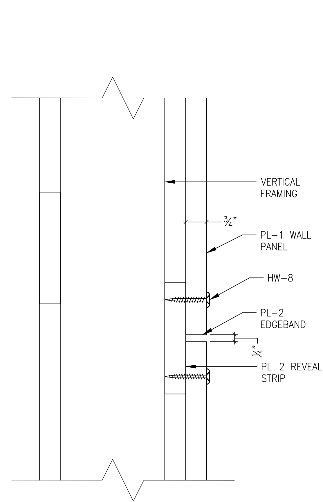
4 SECTION SCALE: 6" = 1'-0" REF: N/A
