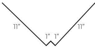
W-Valley 24"
