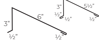
Single Slope Ridge Cap Single Slope Ridge Cap w/Hem
