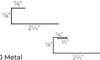
J Metal J Metal W/Hem FAB CODE - 152 BLANK SIZE - 4" FAB CODE - 184 BLANK SIZE - 4.5"
