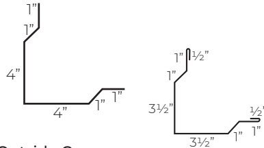
Outside Corner Outside Corner W/Hems FAB CODE - 165 BLANK SIZE - 12" FAB CODE - 194 BLANK SIZE - 12"
