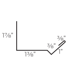
Z Wainscot Transition Z Wainscot Transition W/Hems FAB CODE - 158 BLANK SIZE - 4.5" FAB CODE - 187 BLANK SIZE - 4.5"
