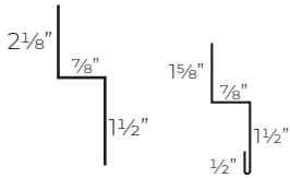
Z Wainscot Transition Z Wainscot Transition W/Hems FAB CODE - 158 BLANK SIZE - 4.5" FAB CODE - 187 BLANK SIZE - 4.5"
