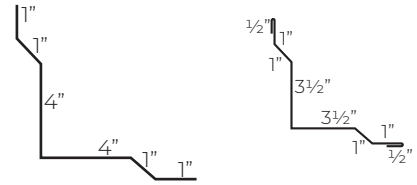
Inside Corner Inside Corner W/Hems FAB CODE - 162 BLANK SIZE - 12" FAB CODE - 193 BLANK SIZE - 12"
