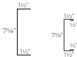
Door Jamb Metal 7-5/8" Face Door Jamb Metal 7-5/8" Face W/Hems FAB CODE - 188 BLANK SIZE - 10.625" FAB CODE - 190 BLANK SIZE - 11.375"
