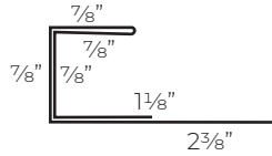
J Metal W/Double Hem FAB CODE - 155 BLANK SIZE - 7"
