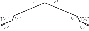
Step Ridge Cap
