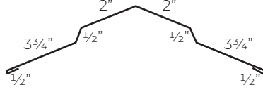
High Step Ridge Cap
