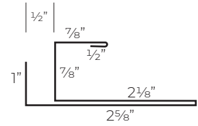
F&J Trim FAB CODE - 169 BLANK SIZE - 8"
