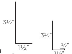
2x4 Fascia 2x4 Fascia W/Hem
