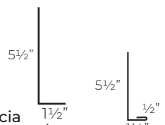
2x6 Fascia 2x6 Fascia W/Hem
