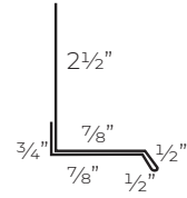
Base Trim W/Under Hem FAB CODE - 146 BLANK SIZE - 6"
