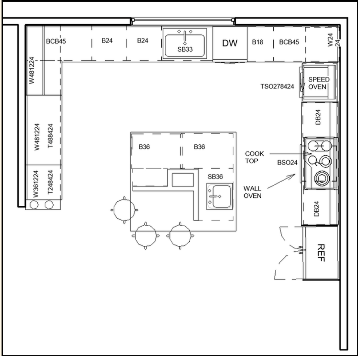
NEW CONSTRUCTION FLOOR PLAN | REVIT
