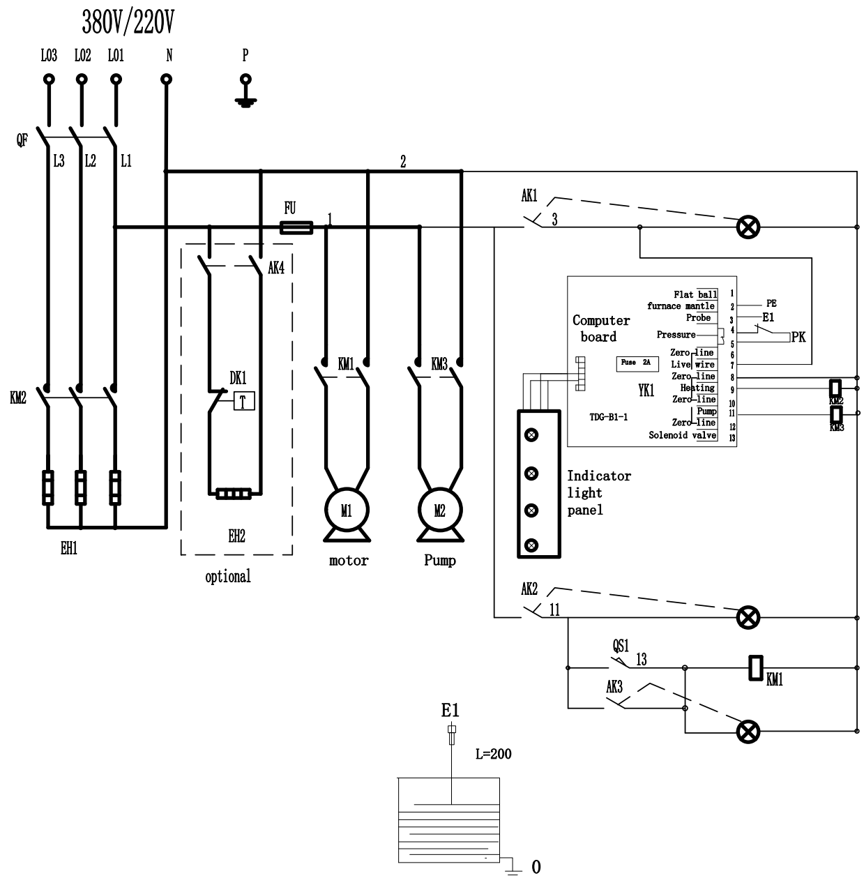
TDG-B1-1 Schematic diagram of energy-saving ironing table
