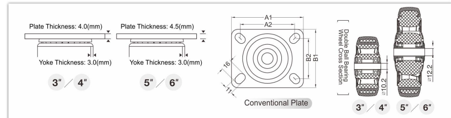
Yoke Finished Options
