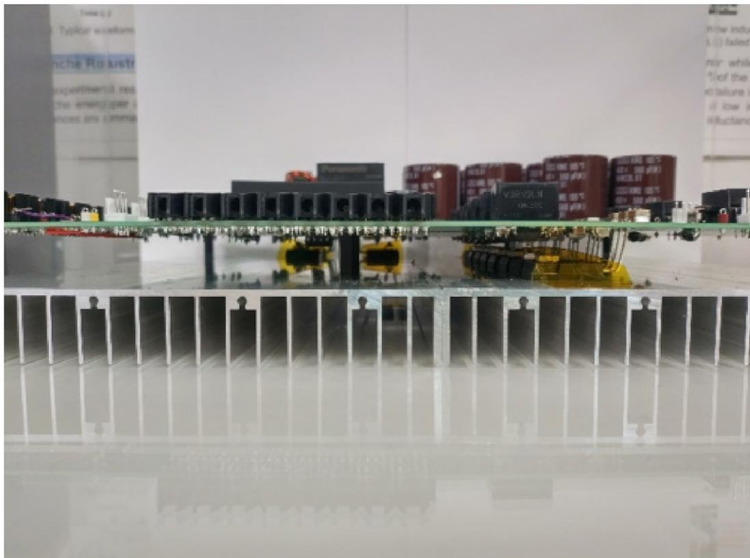
Figure 4. The side view of the AZ-SiC-EVB-10kW-MD evaluation board
