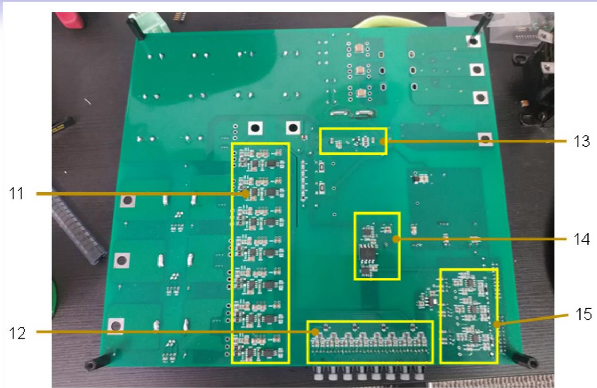
Figure 3. The bottom view of the AZ-SiC-EVB-10kW-MD evaluation board
