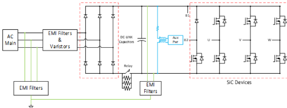
Figure 1. The block diagram of the AZ-SiC-EVB-10kW-MD
