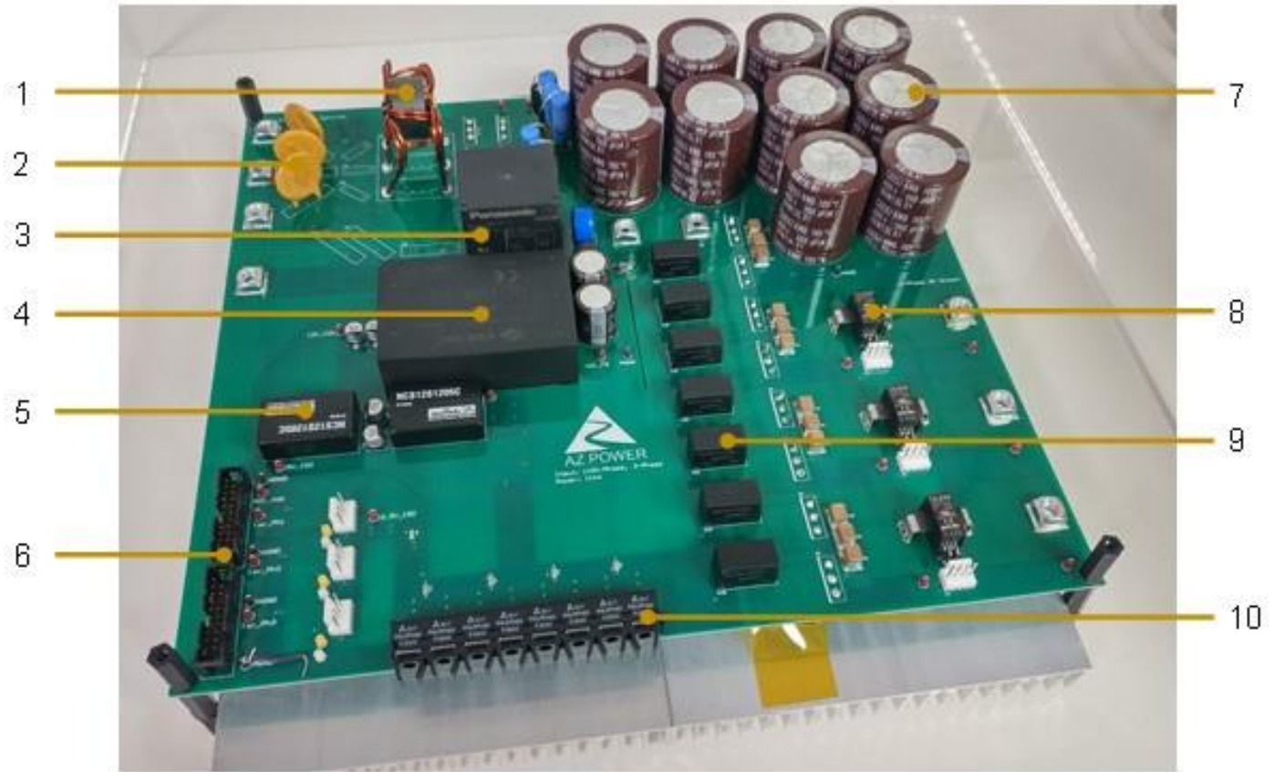
Figure 2. The top view of the AZ-SiC-EVB-10kW-MD evaluation board
