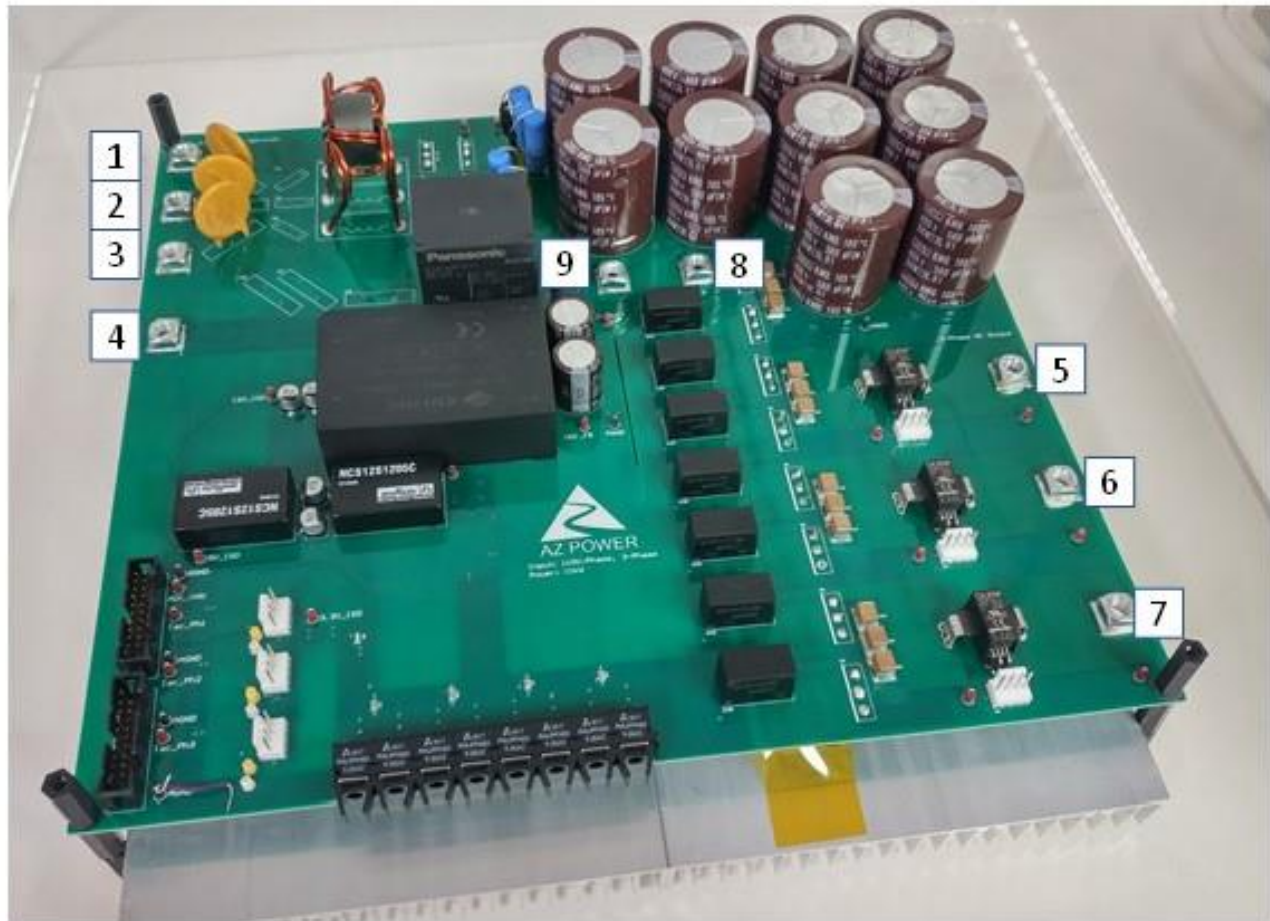
Figure 5. The power interface of the AZ-SiC-EVB-10kW-MD evaluation board
