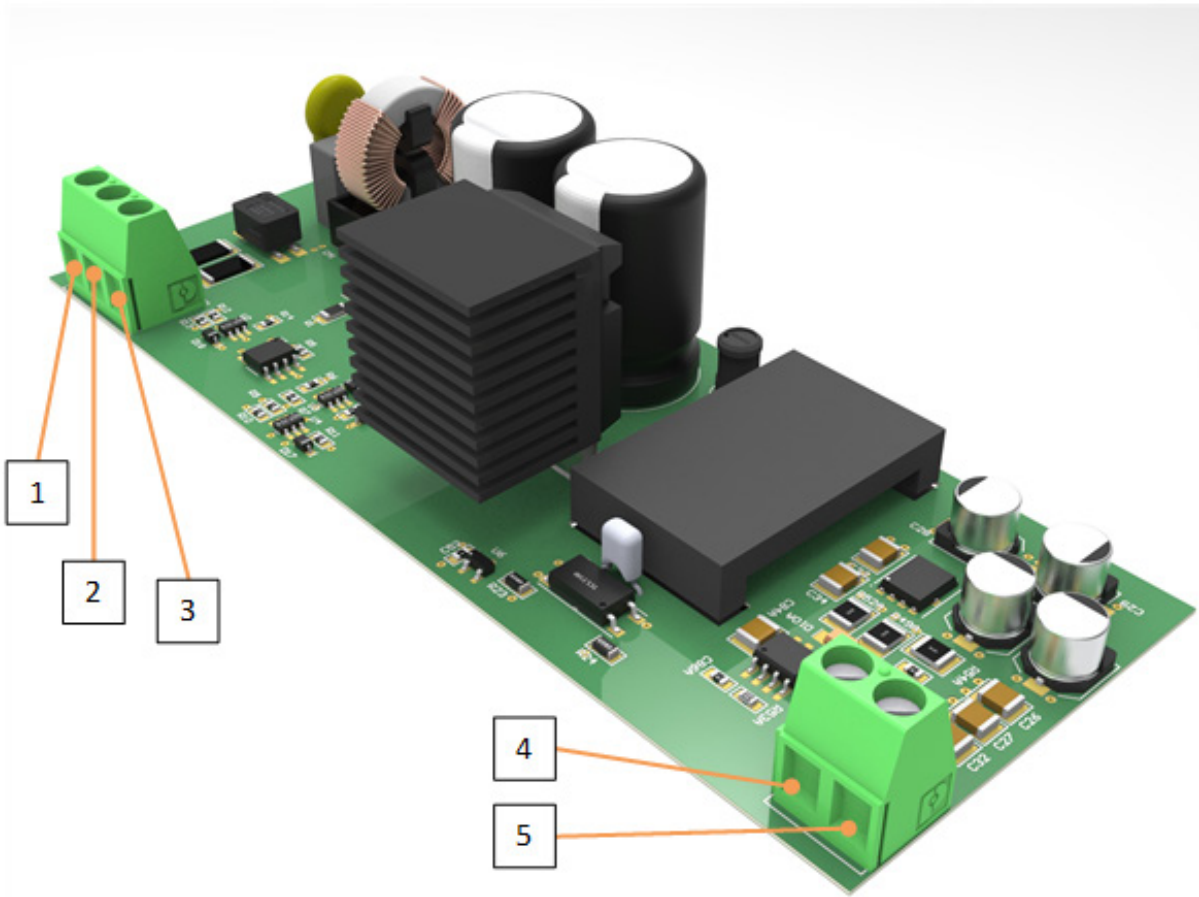
Figure 5. The power interface of the AZ-SiC-EVB-45W-FB evaluation board
