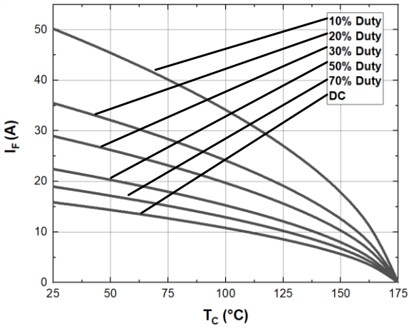
Fig. 3 Current Derating
