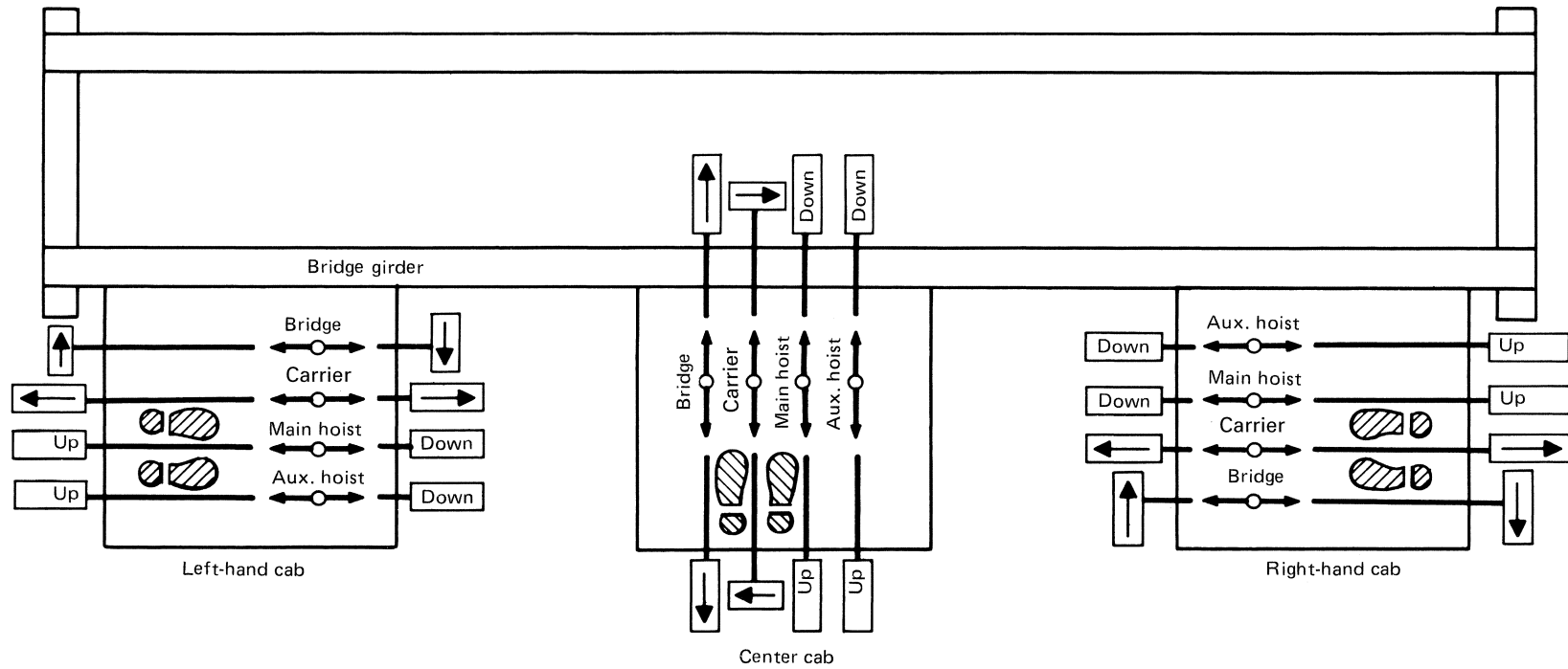
Fig. 11-1.9.3-2 Recommended Arrangement of Controllers (Four-Motor Crane)
