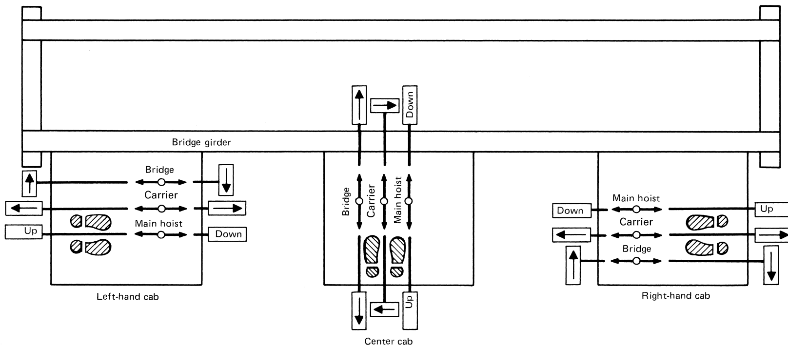
Fig. 11-1.9.3-1 Recommended Arrangement of Controllers (Three-Motor Crane)
