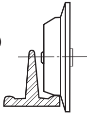
Detail E: Patented Rail With Crown Tread Wheel (Acceptable)
