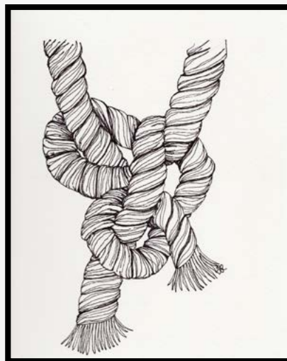
"Knotted." 9"x12"
