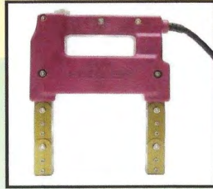
DA400 - A.C./D.C. Contour Probe Available in various kit forms. May be ordered with the Y400 Yoke Light at extra cost.
