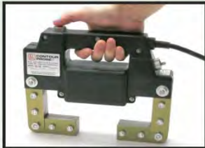
DA200 - A.C./D.C. Contour Probe Model A210 available for A.C. only operation.
