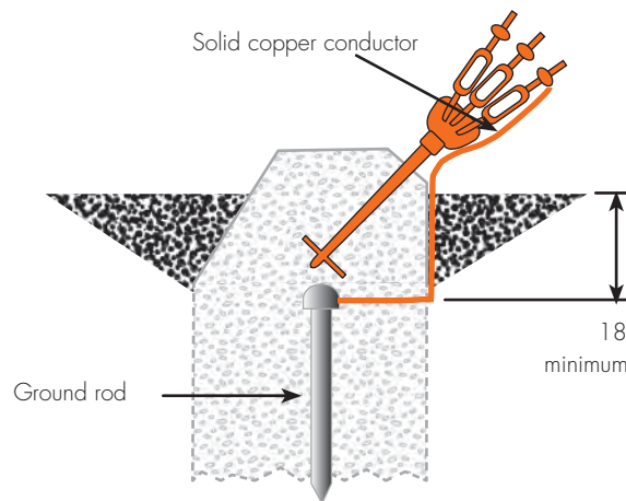
Support grounding installed in a tower's guy wire anchors
