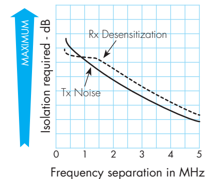
The effect of frequency separation on receiver desensitization and transmitter noise
