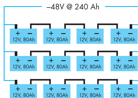
A multi-string battery configuration offering additional redundancy
