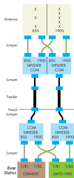
Shared feeders using diplex crossband couplers
