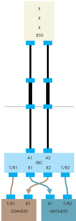
4.16 Antenna sharing accomplished with integrated Duplex/RX SBC
