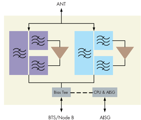
4.25 Dual diplexed dual-band TMA with AISG
