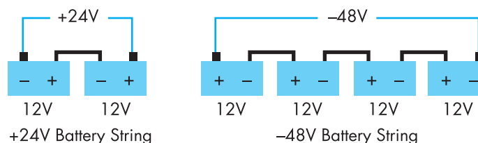
VRLA batteries configured in series for +24V and -48V applications
