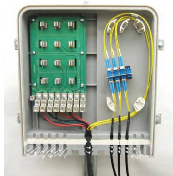
Inside an RRH surge protector module, cover removed
