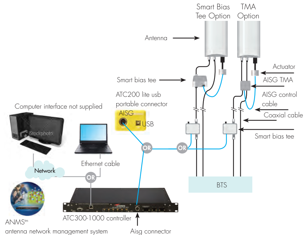
12.3 An example of a cell site using RF cable to carry AISG controller signals
