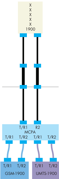
4.11 An MCPA with integrated RX distribution
