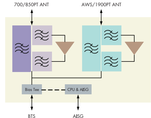
4.26 Diplexed dual-band TMA with pass-through and AISG
