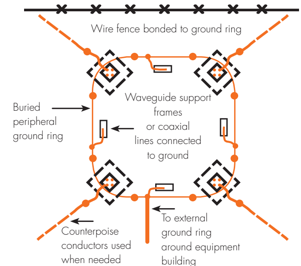
Support grounding for a freestanding tower structure
