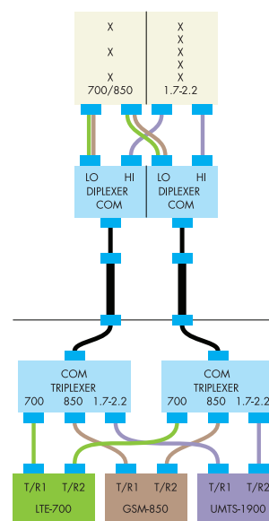
Shared feeders using triplex crossband couplers, with broadband antennas using diplex crossband couplers
