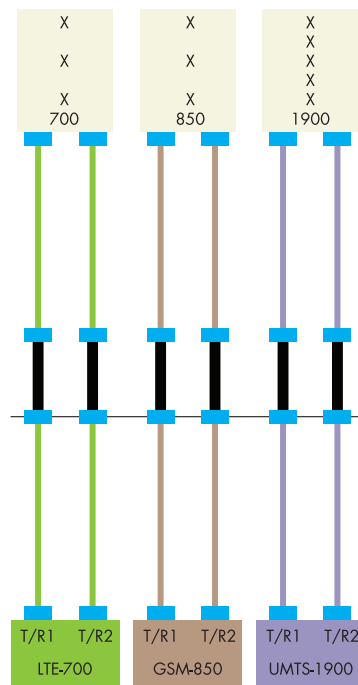
Multiband sector with separate feeders
