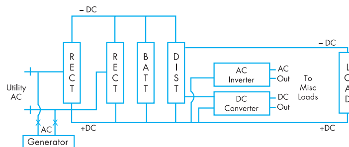
Block diagram of a basic telecommunications power system
