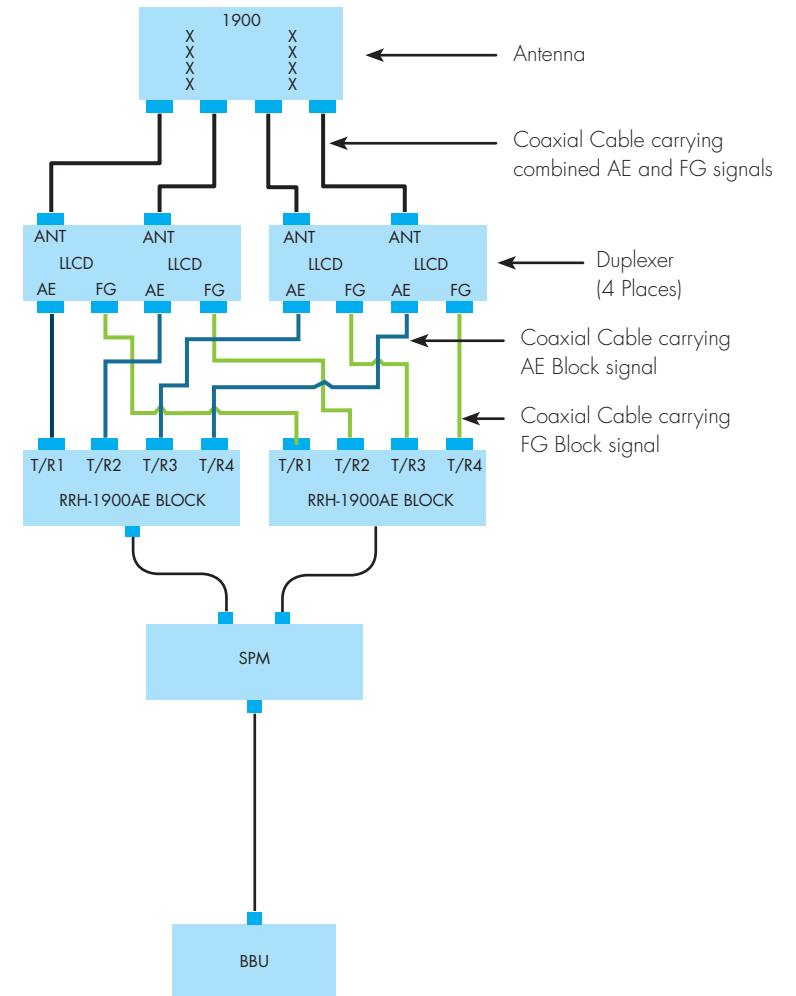
A typical cell site duplexer configuration
