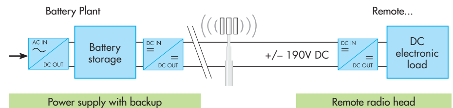
10.25 Line power voltage conversion used for an RRH application
