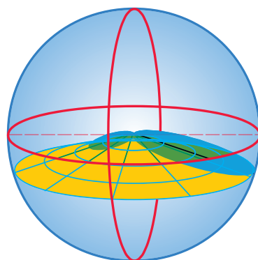
Electrical tilt
