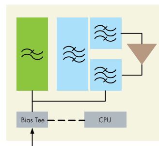
TMA with integrated diplexer, bypass path
