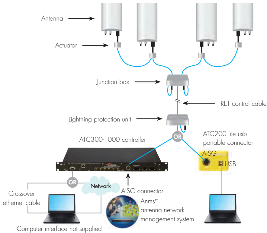
12.2 An example of a cell site using dedicated AISG cable
