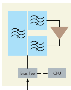
Single-band TMA
