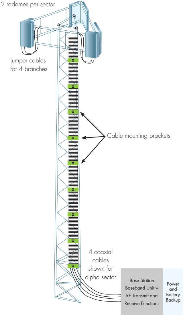
5.2 Typical cell site application, no RRH
