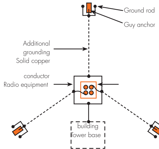
Support grounding installed in a tower pier
