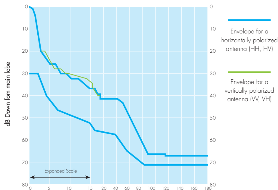
9.9 A typical radiation pattern envelope (RPE) document
