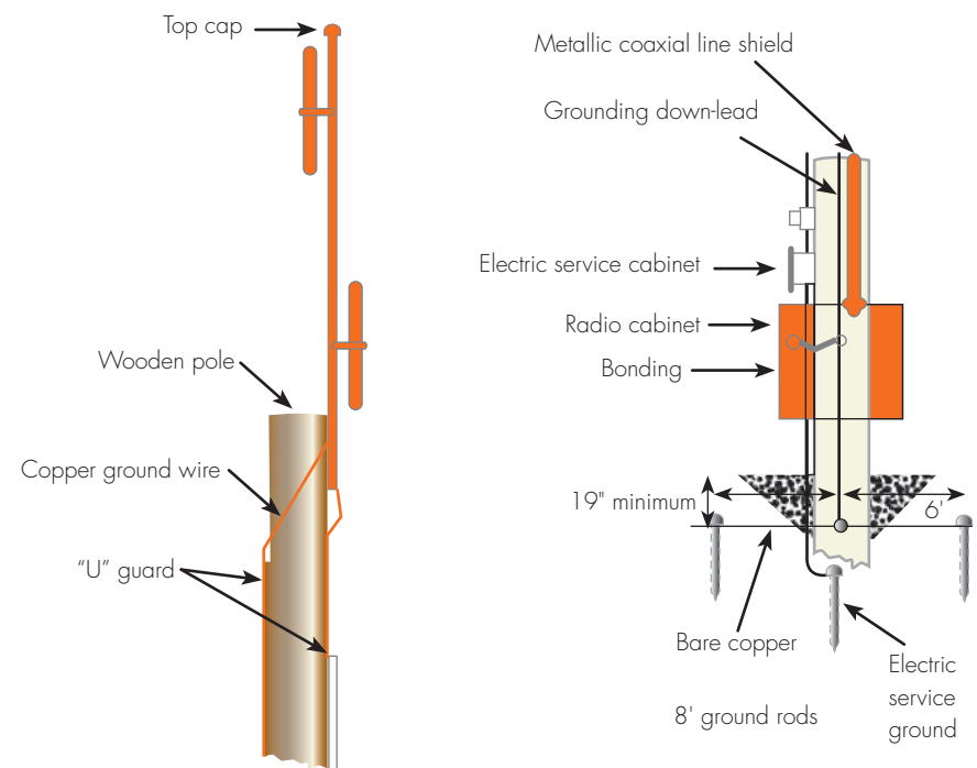
Grounding details for a wooden pole-mounted antenna
