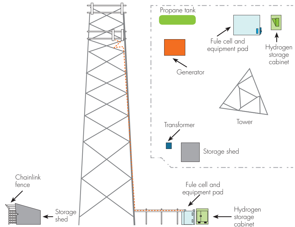
10.8 A typical layout for a base station's fuel cell power plant
