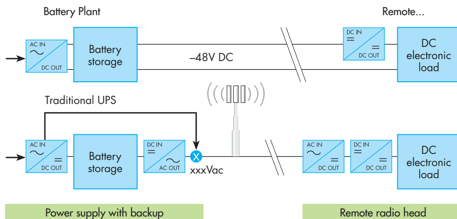
10.24 DC powering options for remote radio heads (RRHs)
