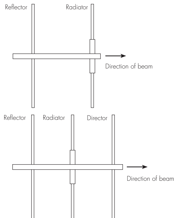
Two-element and three-element Yagi directional antenna
