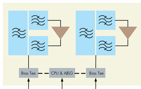
Twin single-band TMA with AISG support
