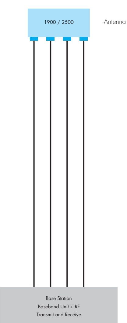
5.1 Typical cell site architecture, no RRH
