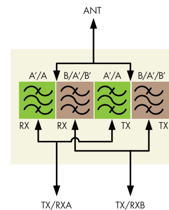
4.8 Filter multiplexer for downlink and uplink – a quadruplexer
