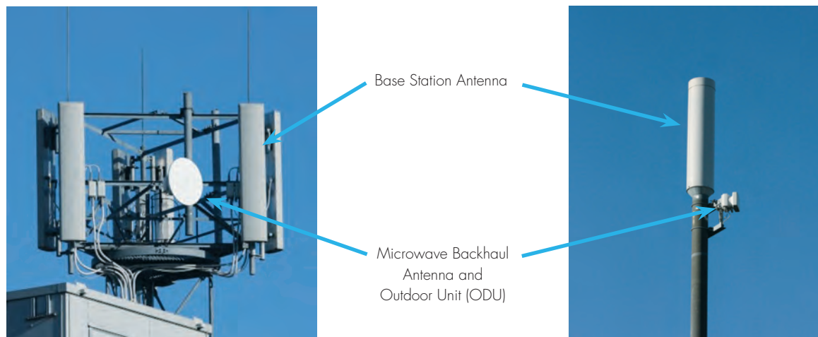
9.5 Typical microwave backhaul antenna integrated into a base station antenna location
