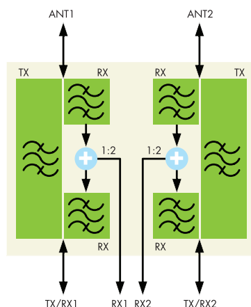
4.18 Integrated SBC
