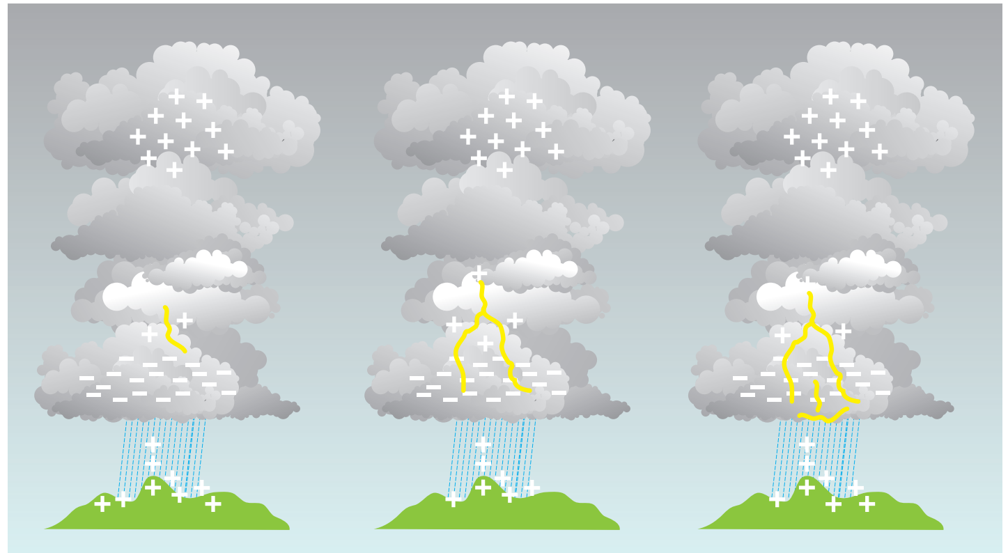
The origination and path of a cloud-to-ground strike
