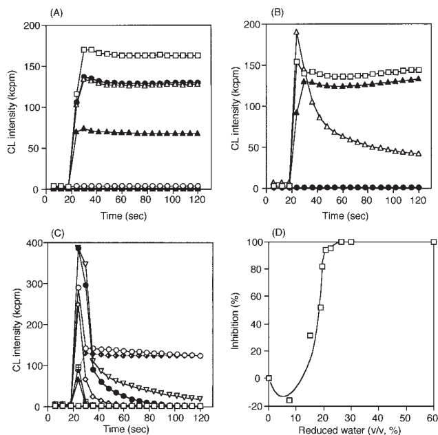
FIG. 2. Analysis of the SOD-like activity of reduced water. (A) Effects of reduced water, SOD, H_2 -water and N_2 -water on the accumulation of O_2^{\cdot -} generated by the HX-XOD system. The CL intensity was determined in phosphate buffer (pH 7.0) in the presence of reduced water (RP -820 mV, pH 11.0; IC_{50}SO(18\%) ), a NaOH solution of the same pH as reduced water, SOD, H_2 -water, or N_2 -water. \square , control NaOH solution; \blacksquare , reduced water; \blacktriangle , SOD (0.13 U/ml); \circ , SOD (66.7 U/ml); \bullet , H_2 -water; \triangle , N_2 -water. (B) Stability of the SOD-like activity of reduced water. \square , control NaOH solution. \bullet , reduced water and reduced water treated with repeated freezing and melting, deflation with sonication, vigorous mixing for 10 minutes, boiling for 10 minutes, repeated filtration with 0.22 \mu m filter, or closed autoclaving at 121°C for 20 minutes. \blacktriangle , reduced water treated with opened autoclaving at 121°C for 20 minutes. \triangle , reduced water treated with closed autoclaving in the presence of tungsten trioxide (0.5 g/70ml reduced water) at 121°C for 20 minutes. (C) The SOD-like activity of diluted reduced water. Amount of reduced water (%): \square , 60%; +, 30%; *, 26%; \blacktriangle , 23%; \square , 21%; \diamond , 20%; \bullet , 19%; \nabla , 15%; \circ , 7.5%; \blacklozenge , 0% (control). (D) Inhibition of the accumulation of O_2^{\cdot -} by variously diluted reduced water. All experiments were triplicated and the average values were shown in the figures. The SD errors were within 5%.
